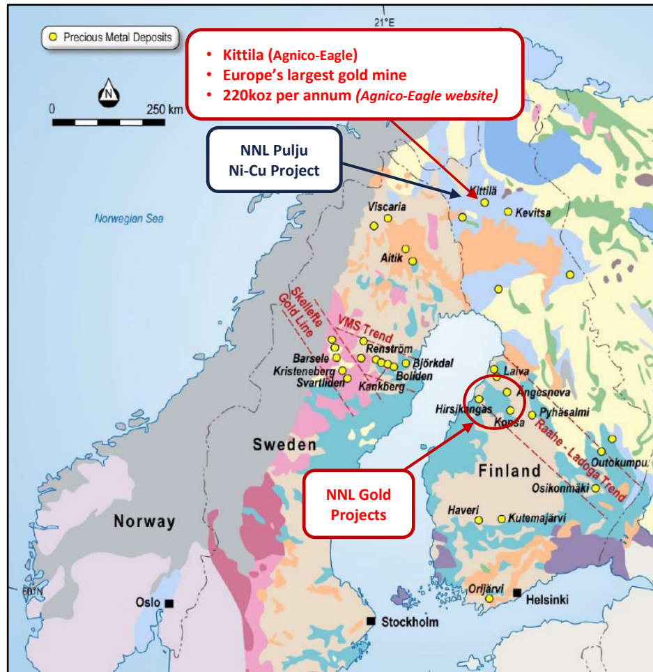
Figure 5: Location of NNL's three gold projects shown over a geological map of Finland.
