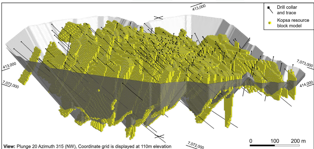
Figure 3. View to the NW of the entire in situ Kopsa block model (no classification applied) and the associated optimised pit shell. Coordinates presented in ETRS-TM35FIN system (EPSG:3067).
