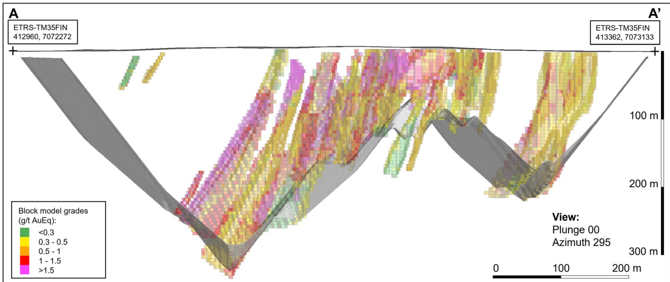
Figure 4. 100m wide cross section of the block model (blocks classified by grade) and optimised pit shell. Positioning of the cross section is provided in Figure 2. Coordinates presented in ETRS-TM35FIN system (EPSG:3067).
