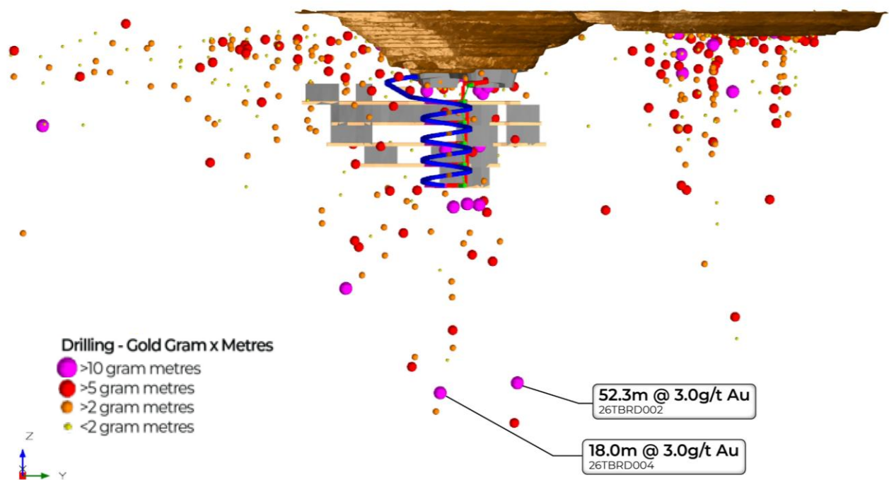
Figure 5: Fairway long section showing the initial mine plan (~18 months) and 2026 drill results well below the initial Ore Reserve.
