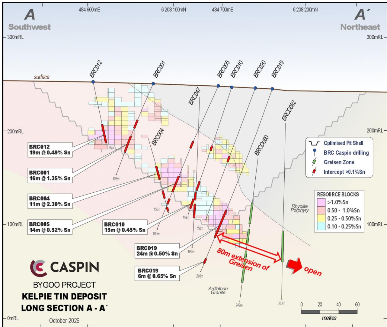
Figure 3. Long section in the plane of the Dumbrell's Fault showing the position of greisen-style alteration in recent diamond holes BRC012, BRC001, BRC004, BRC005, BRC010, BRC019, BRC047, BRC080, and BRC082, demonstrating at least an 80m likely continuation of mineralisation.
