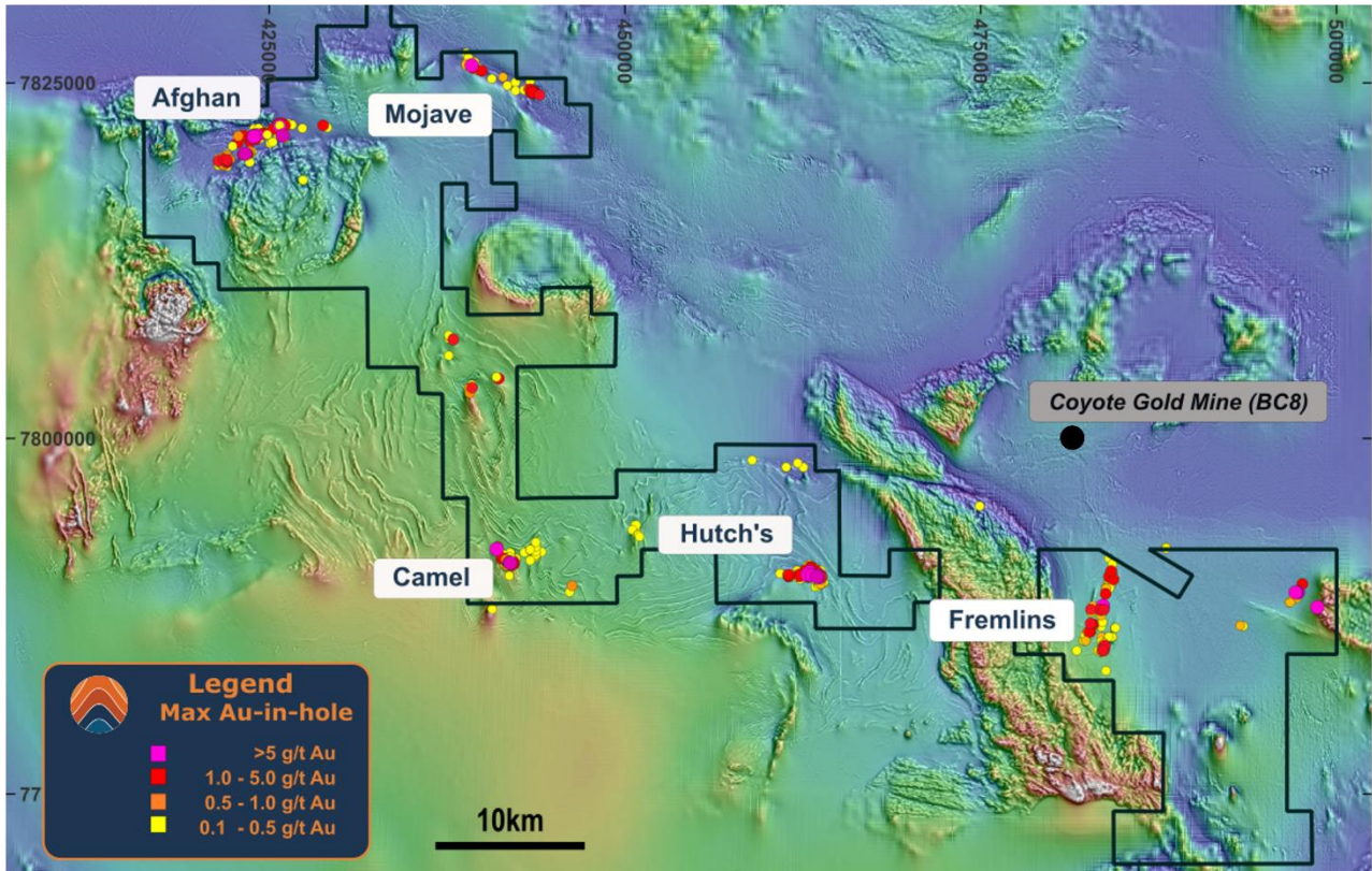
Figure 8: West Tanami Leases, max gold-in-hole 2 (+0.1g/t Au), key prospects on magnetics (GDA94 z52)
