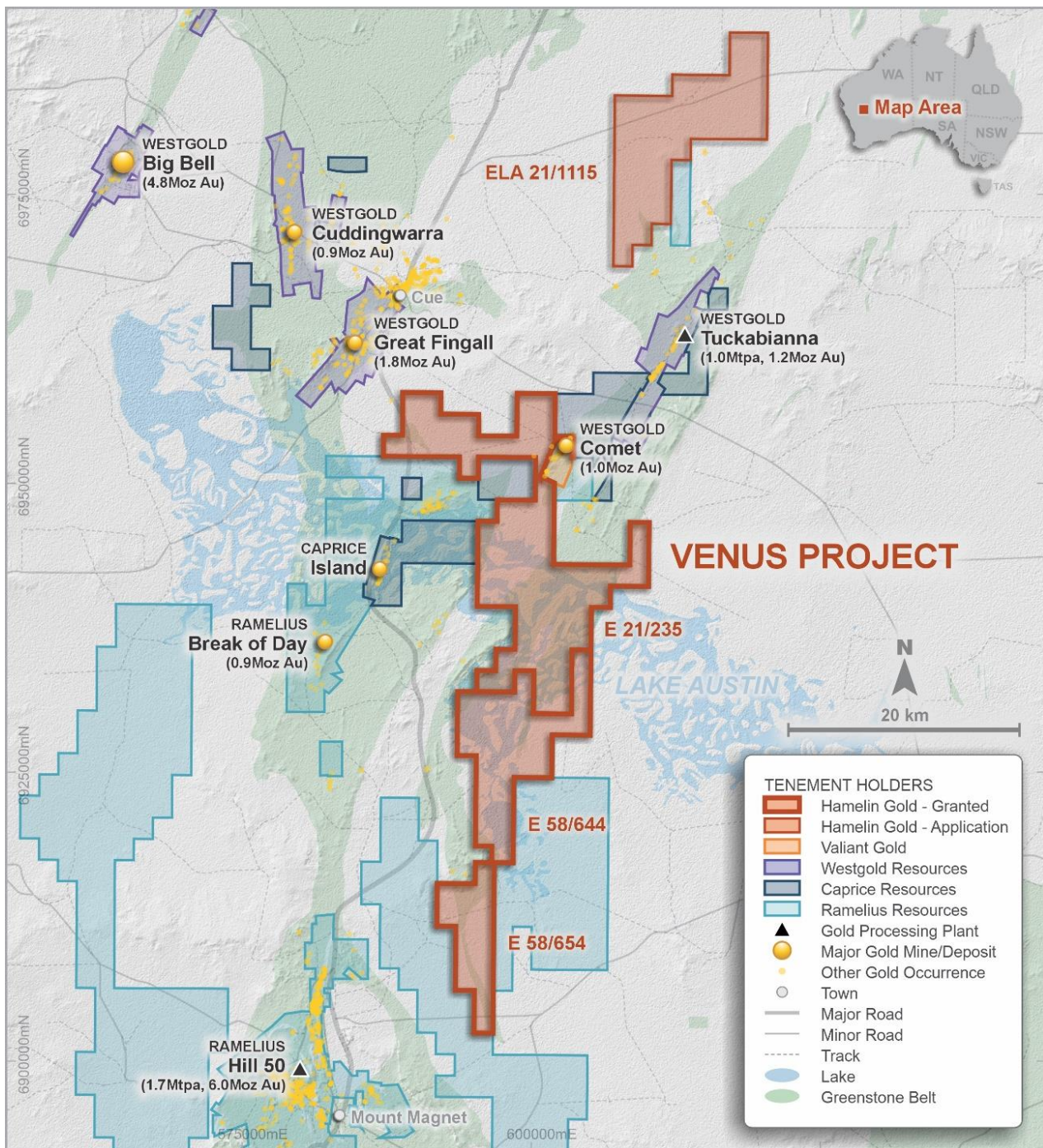
Figure 6: Venus Project – Location plan, major gold occurrences and regional leasing (GDA94 z50)
