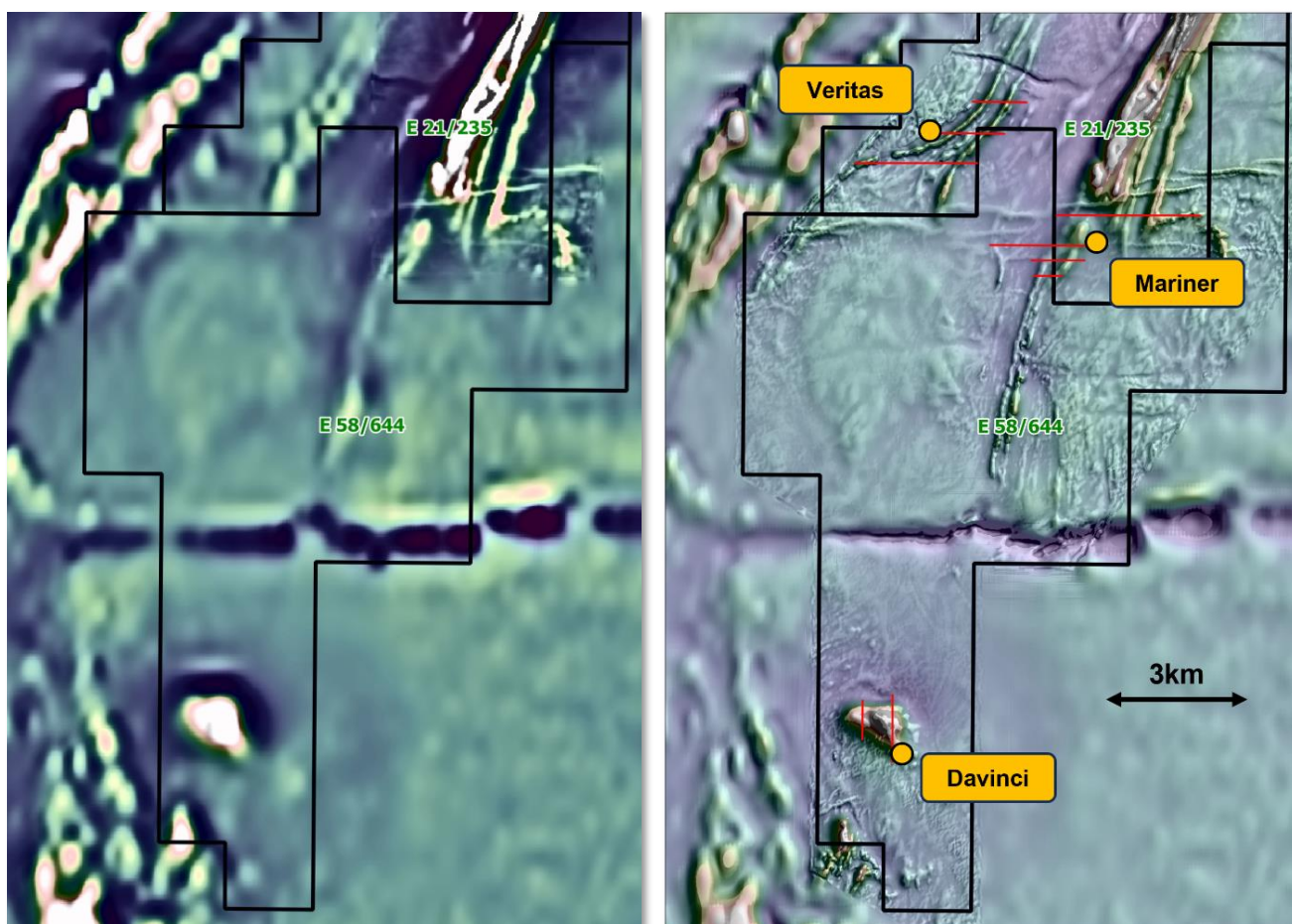
Figure 7a: Venus Project – Regional aeromagnetic data on leasing
