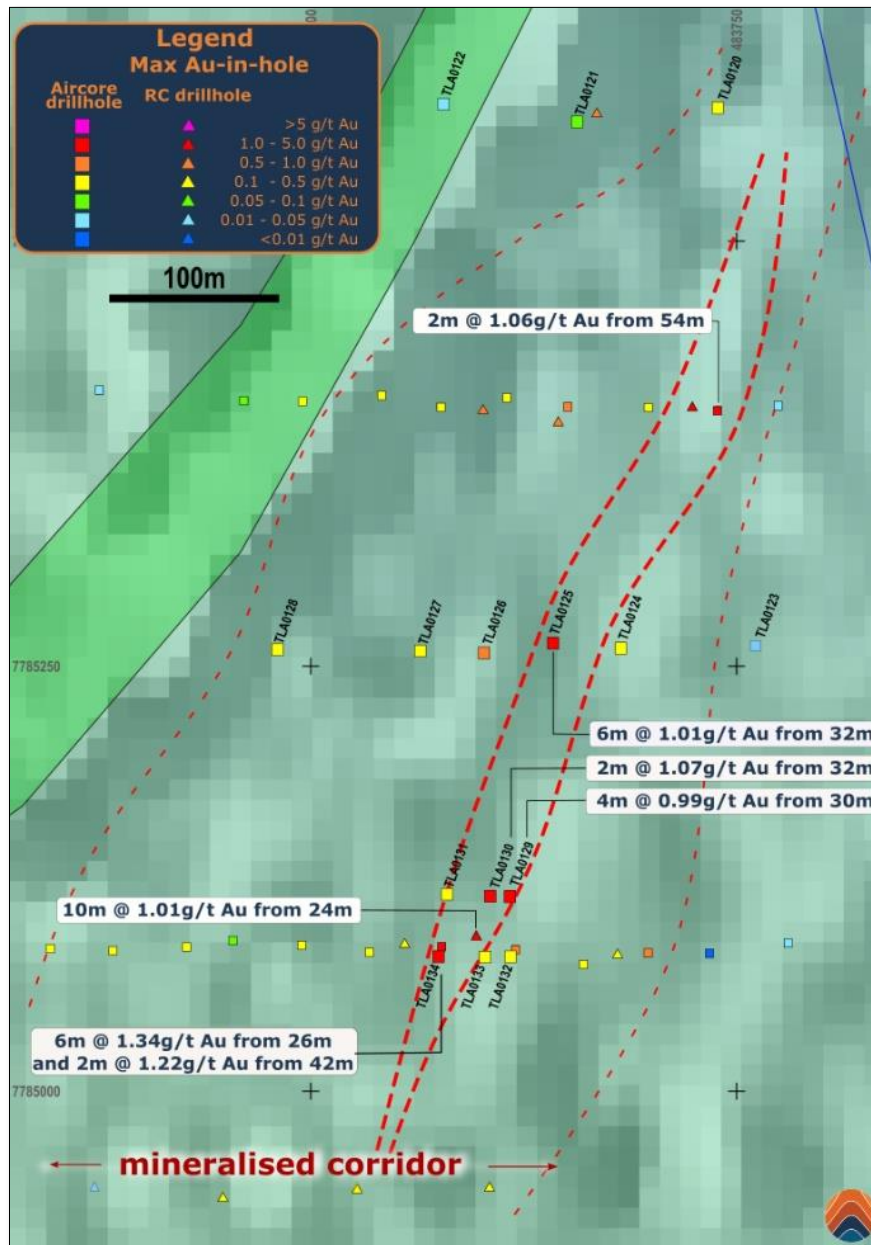
Figure 9: Fremlins South RC drilling results (GDA94 z52) see ASX announcements 12 Sep 2025 & 14 Nov 2025
