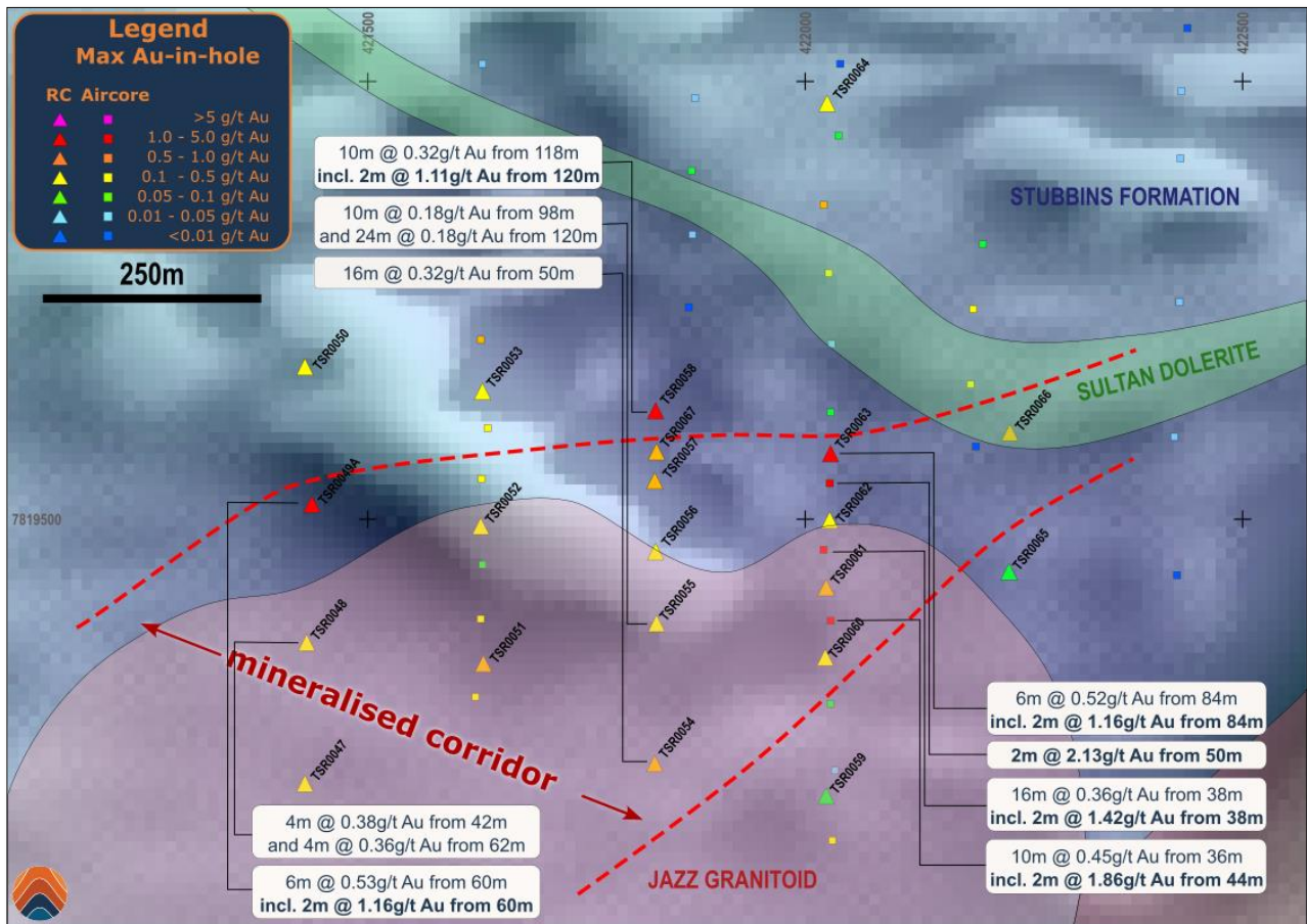
Figure 10: RC drilling results and interpreted geology at Jazz (GDA94 z52) see ASX Announcement 13 Jan 2025 & 14 Nov 2025
