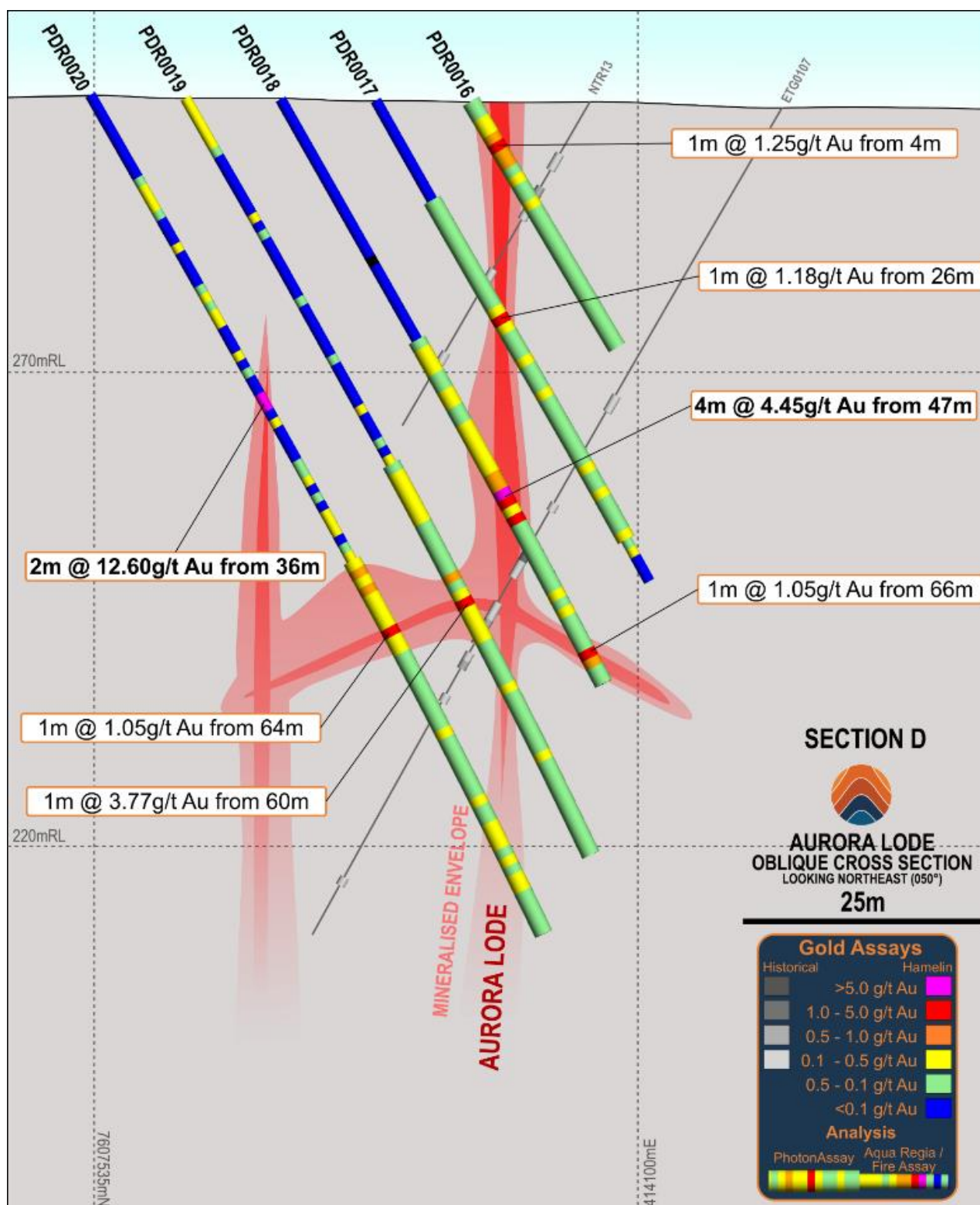
Figure 3: Aurora Cross Upper Lode
