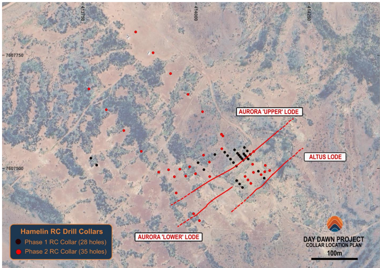
Figure 2: Day Dawn Project – Aurora / Altus Lodes, Phase 1 (28 holes) and Phase 2 (35 holes) RC collar plan on Bing Sat image MGA94 z51
