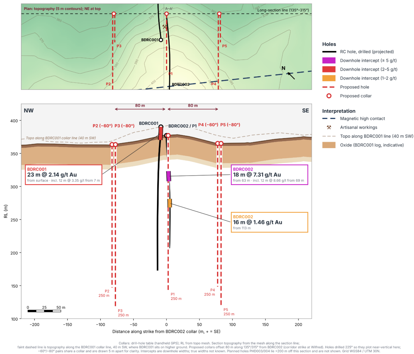
Figure 3. Vertical long section through the BDRC002 collar (looking NE, true scale), showing the BDRC001 and BDRC002 intercepts and proposed step-out holes 80 m NW and 80 m SE of BDRC002. A -60° and a -80° hole are planned at each step-out collar, plus the -70° follow-up from the BDRC002 collar, all to 250 m. Downhole widths; true widths not known.
