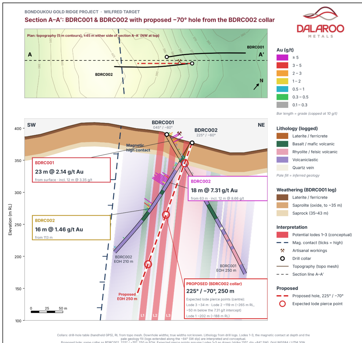
Figure 1. Cross-section A-A' (looking NW) through BDRC001 and BDRC002, showing downhole gold assays, logged lithology and the interpreted lodes. BDRC001 returned 23 m @ 2.14 g/t Au from surface, and BDRC002 returned 18 m @ 7.31 g/t Au from 63 m and 16 m @ 1.46 g/t Au from 113 m. A follow-up hole ( 225^\circ / -70^\circ , 250 m) is proposed from the BDRC002 collar to test the lodes about 50 m below the high-grade intercept. Lodes and geology away from the drill holes are interpreted. Downhole widths; true widths not known.
