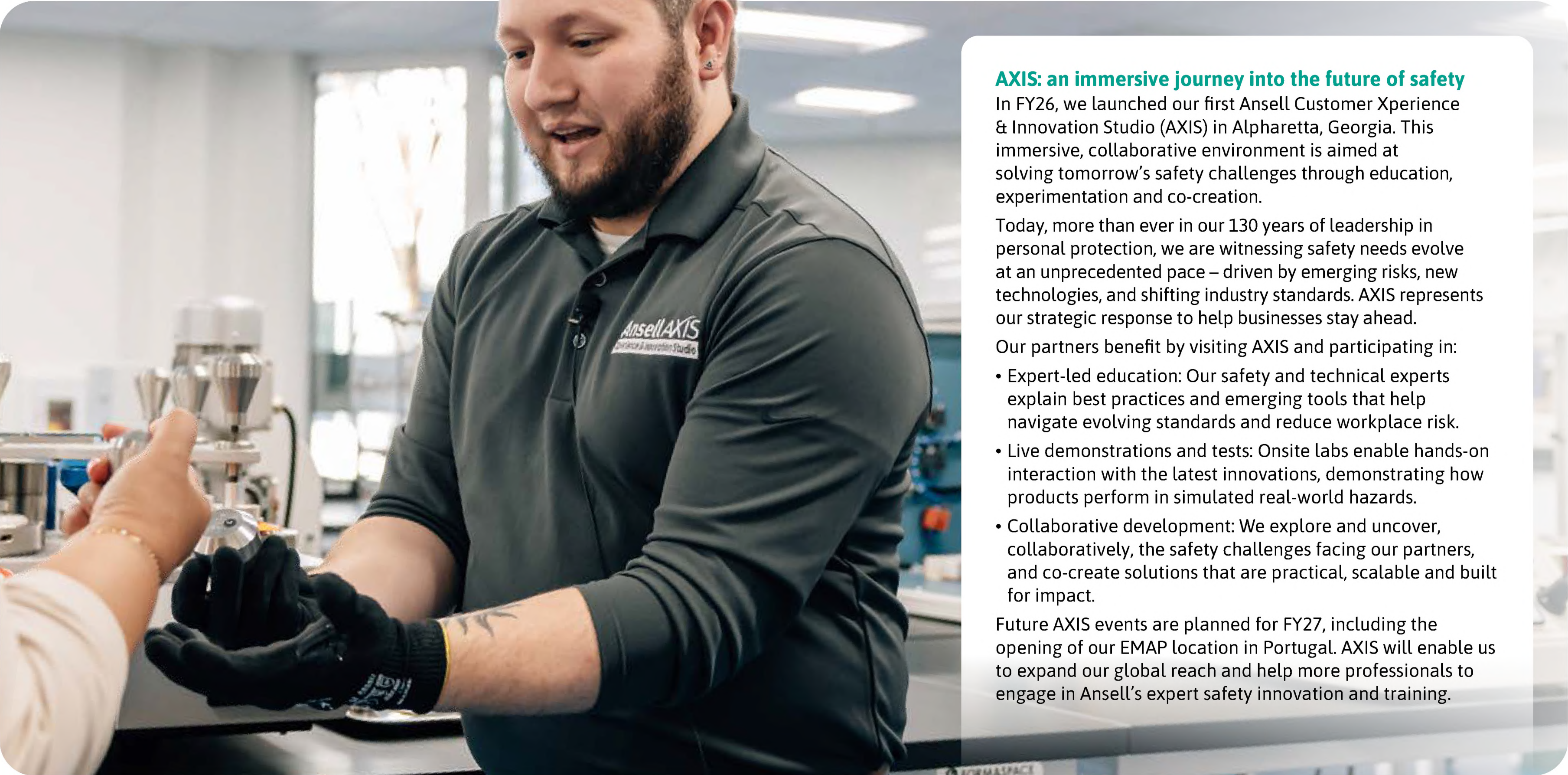
← Image caption: During the opening of the AXIS facility in October 2025, an Ansell R&D Engineer demonstrates one of the testing methods used to evaluate glove performance and abrasion resistance.
