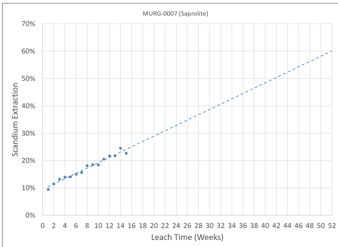
Figure 2: 52-week projection of weekly scandium recovery data for saprolite host rock material derived by applying a linear line of best fit (excluding the initial rapid extraction).
