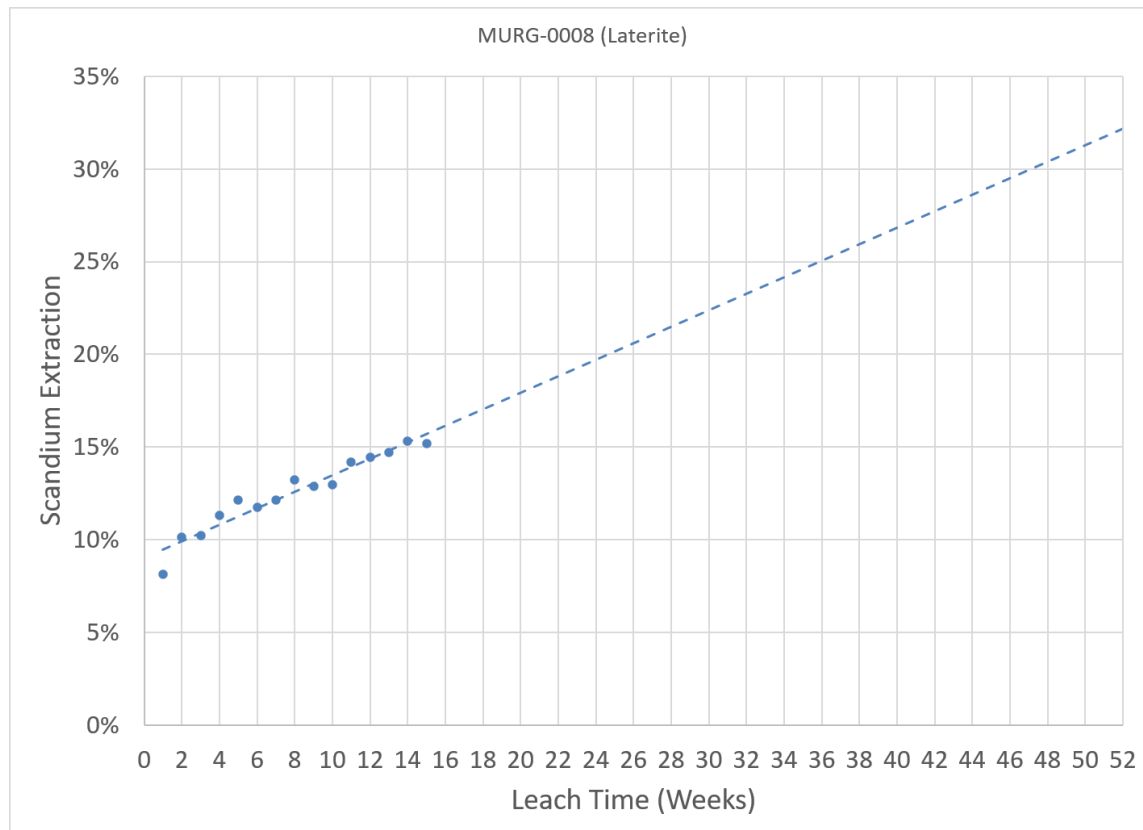
Figure 3: 52-week projection of weekly scandium recovery data for laterite host rock material derived by applying a linear line of best fit (excluding the initial rapid extraction).
