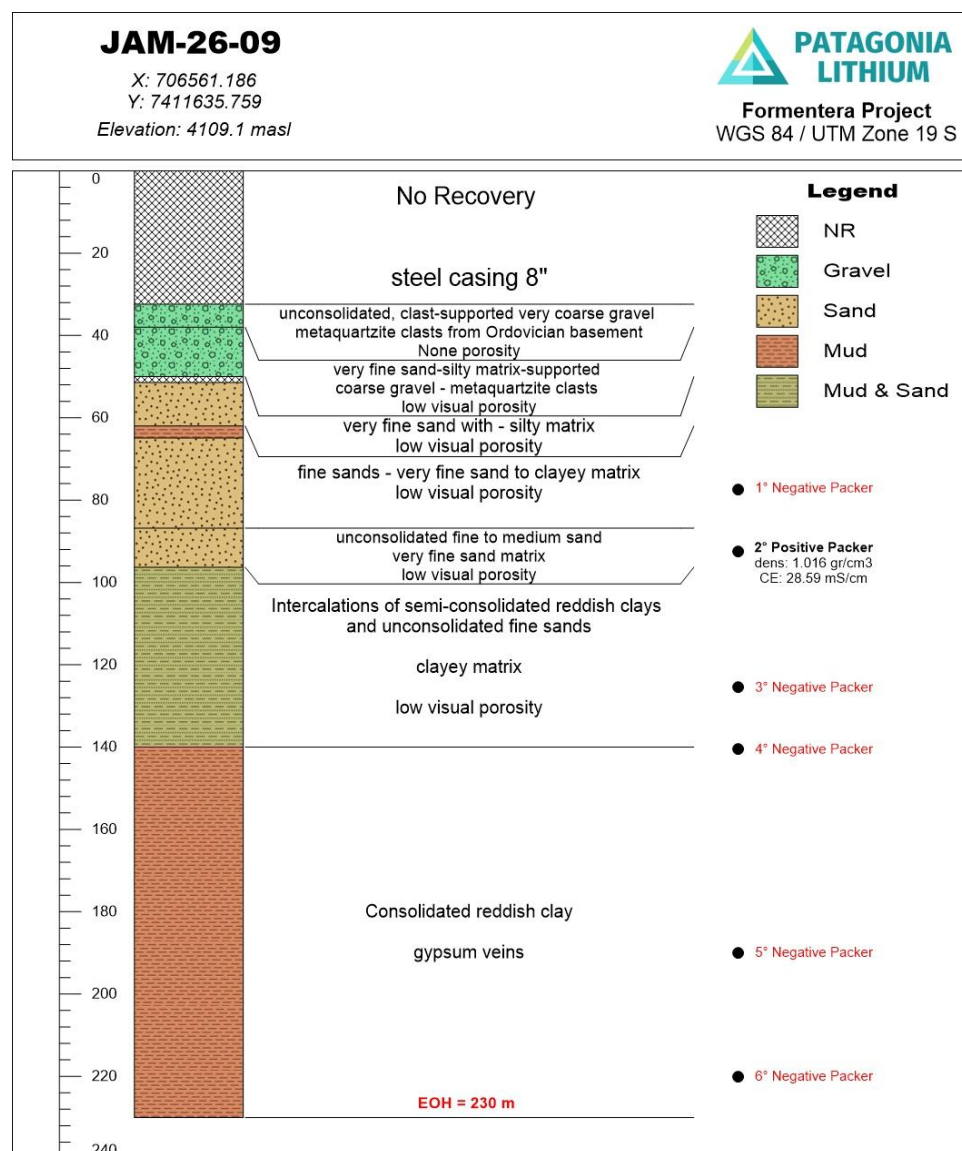
Figure 2. Lithological column showing clays from 140m to 230m and packer test depths for JAM 26-09.
