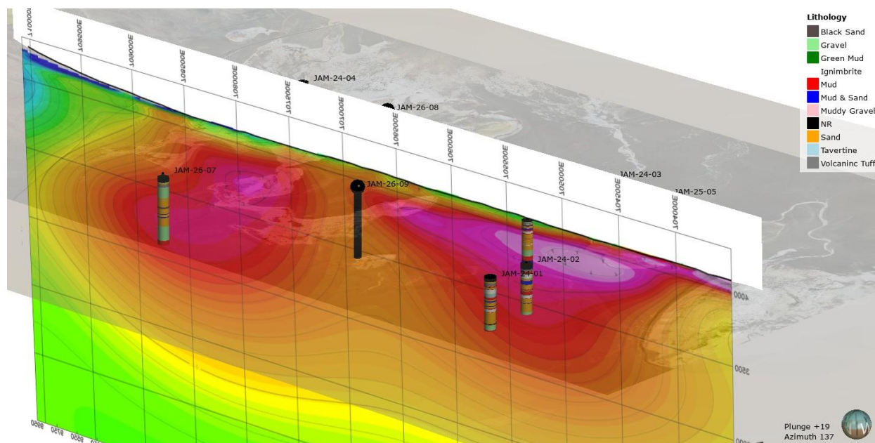
Figure 3. Well 9 positioned against the 2D Inversion data from the MT surveys and drilling the further most extent of the aquifer. Pink area has the lowest resistivity.
