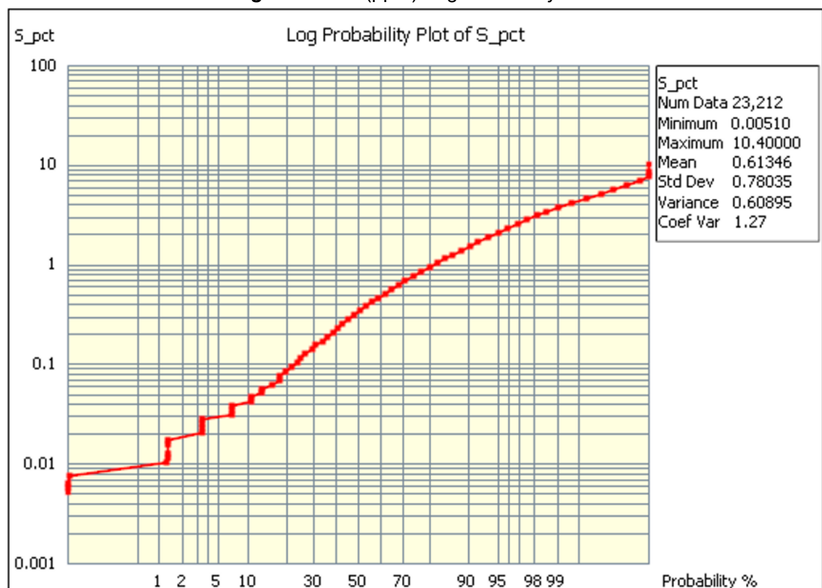
Figure 13: S (%) Log Probability Plot
