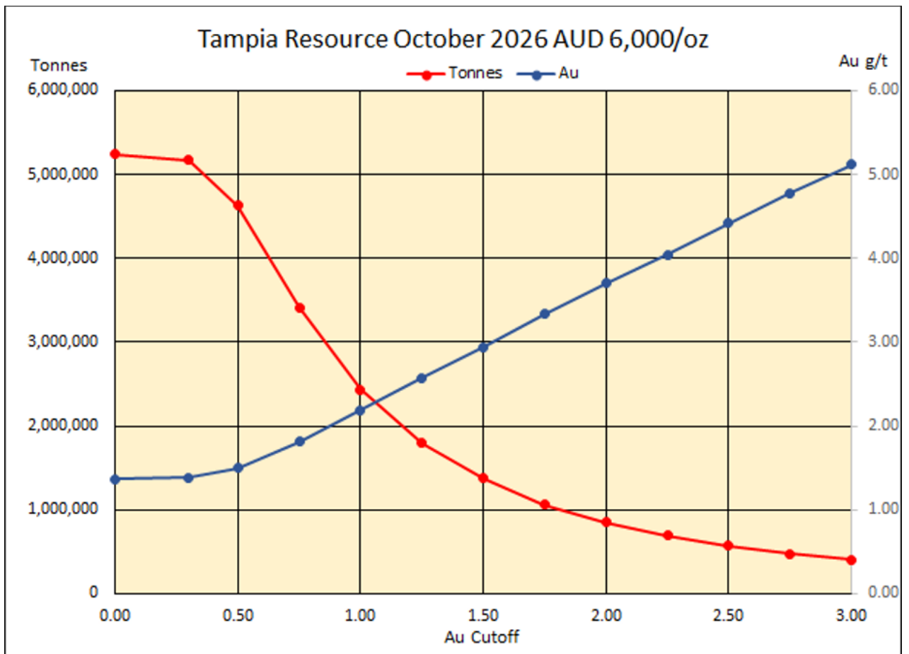
Figure 17: Optimal Grade Tonnage Curve for the Tampia Deposit (Indicated + Inferred)
