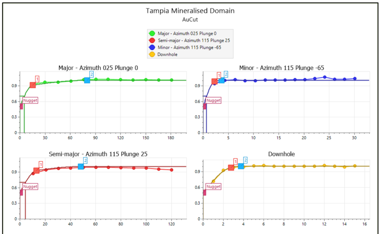
Figure 14: Variogram Models
