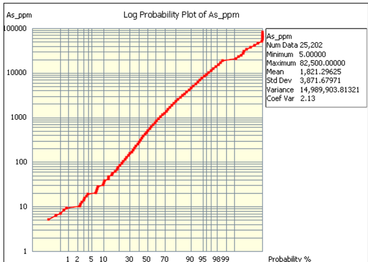
Figure 12: As (ppm) Log Probability Plot
