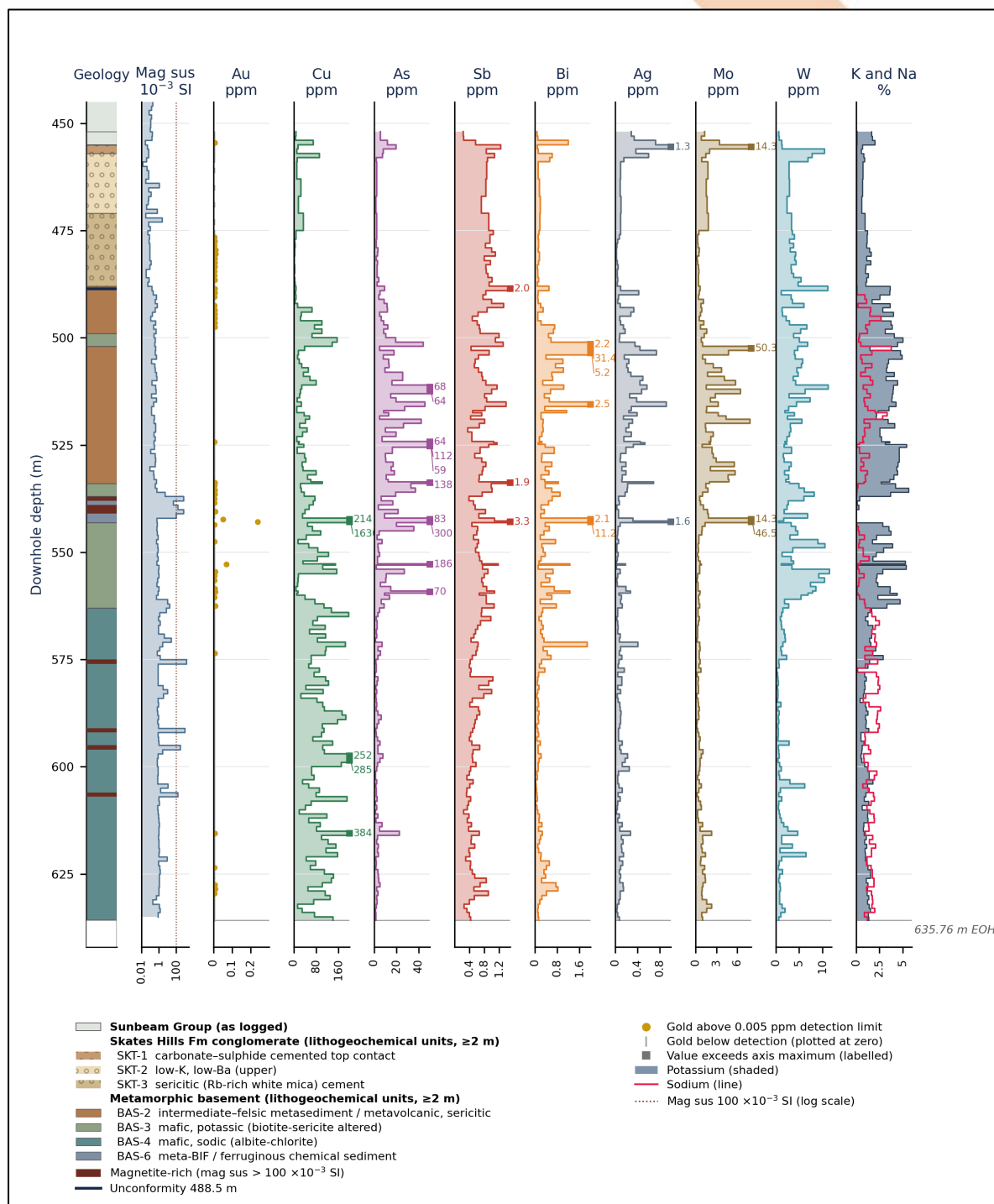
Figure 2: MD002DD downhole summary with simplified geological log and downhole assay results for selected elements, plotted over each sampled interval. The 4.0 m intervals within the Skates Hills Formation conglomerate (459.0–475.0 m) are laboratory composites of 1 m half-core samples. Gold results below the 0.005 ppm detection limit are shown at zero in grey. The strongest coincident gold-copper result occurs at 542.72–543.09 m (previously reported 20 August 2026). Geology is shown as lithogeochemical classes derived from the assay data; magnetite-rich intervals (magnetic susceptibility greater than 100 \times 10^{-3} SI) are highlighted.
