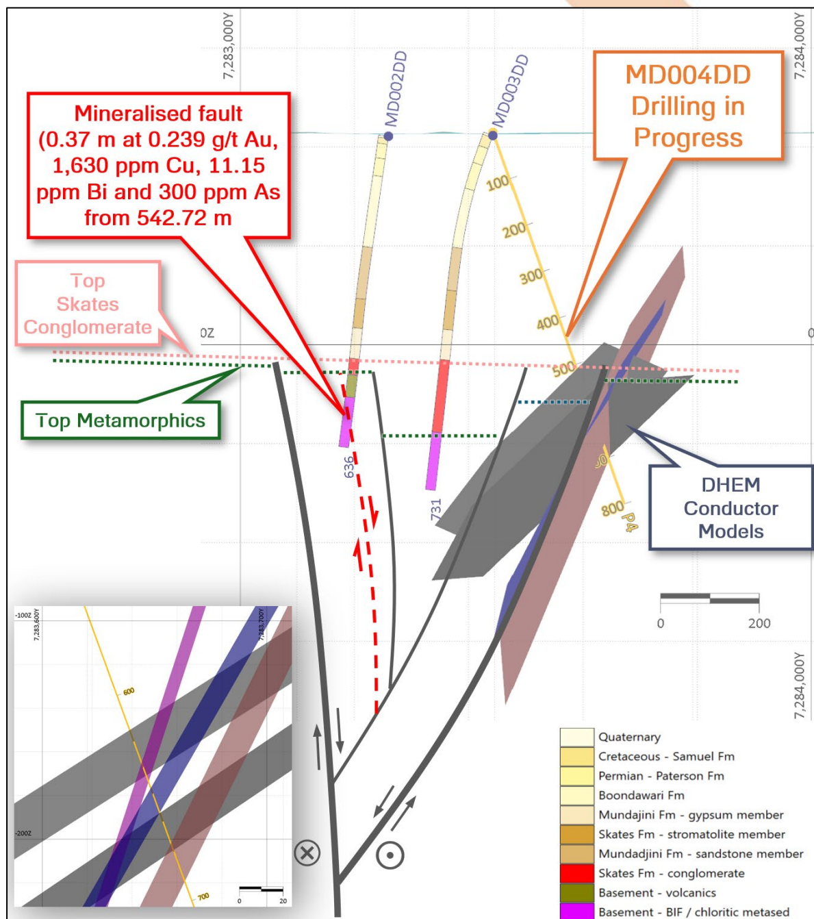
Figure 4: Madman Project summary cross section (looking ~WNW) showing the planned MD004DD trace testing the finalised DHEM conductor plate models along with an interpretive fault model based on preliminary observations and measurements. The 800 m planned hole is projected to intersect the plates between approximately 600 m and 700 m downhole (see inset).
