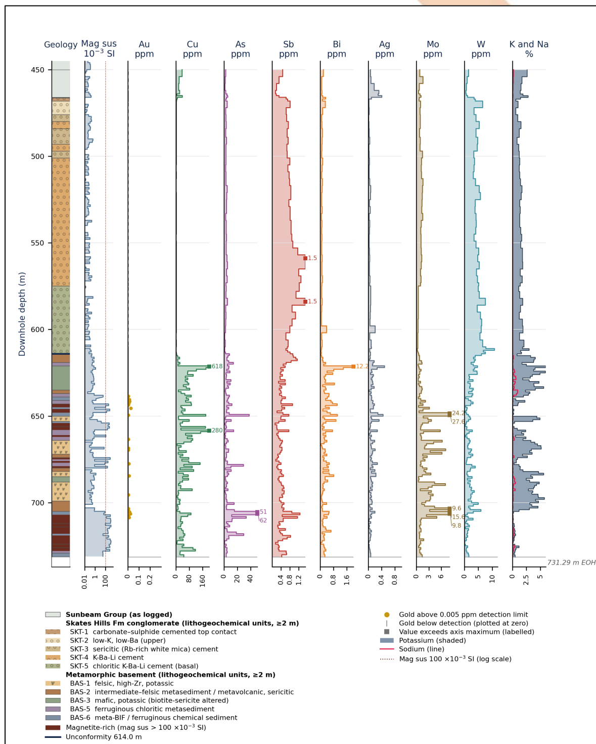
Figure 3: MD003DD downhole summary, plotted at the same scales as Figure 2.
