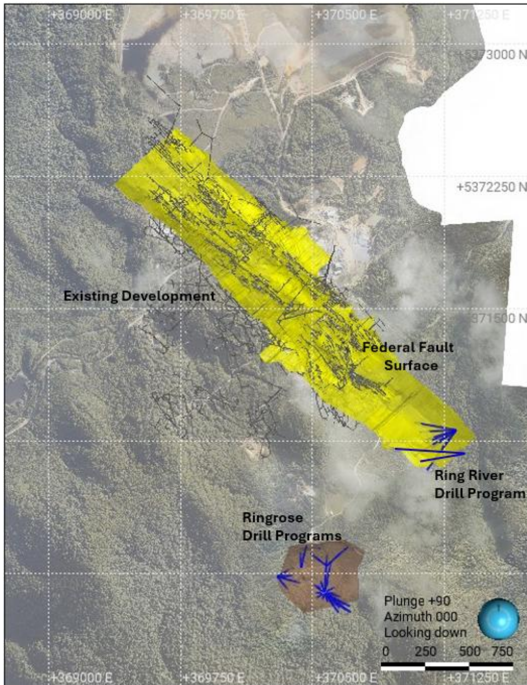
Figure 1: Location plan (MGA) of completed Ringrose and Ring River drill programs (blue traces) since last Metals X ASX Exploration release 18 November 2024. Existing development on the Federal Fault surface (yellow).
