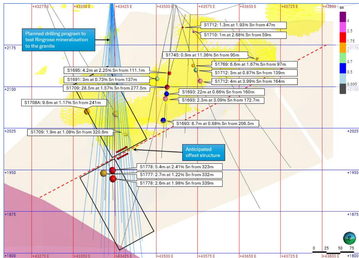
Figure 2: Ringrose Long Section (NRM Grid) showing mineralisation (yellow) and new significant intersections since Metals X ASX release 18 November 2024. Note previously unrecognised offset in mineralisation at depth. Coordinates are in New Renison Mine Grid.
