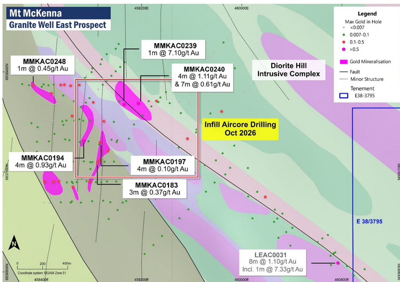
Figure 2. Map showing intercepts and mineralised trends identified from Platina's 2026 aircore drilling at the Granite Well East Prospect (Targets 4 and 5), Mt McKenna Gold Project. Map underlain by interpreted simplified bedrock geology.
