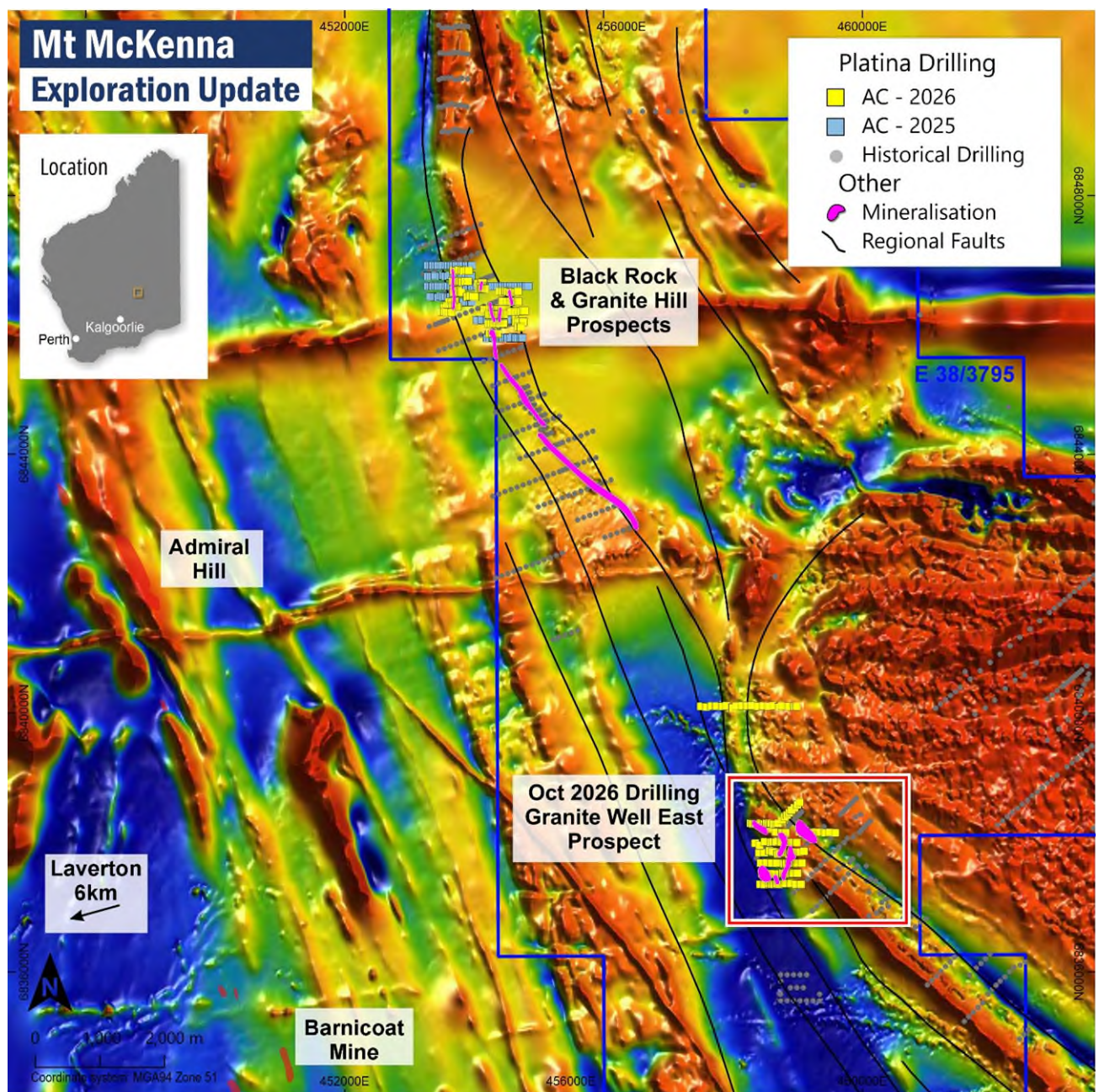
Figure 1. Map showing historical drilling along with Platina's aircore drilling on Mt McKenna's E38/3795 tenement. Red box indicates the current area of aircore drilling. Observed mineralised corridors are also shown in pink. Map underlain by Geological Survey of Western Australia's (GSWA) reprocessed and Platina's newly acquired merged TMIRTP 1VD magnetic image by Core Geophysics.
