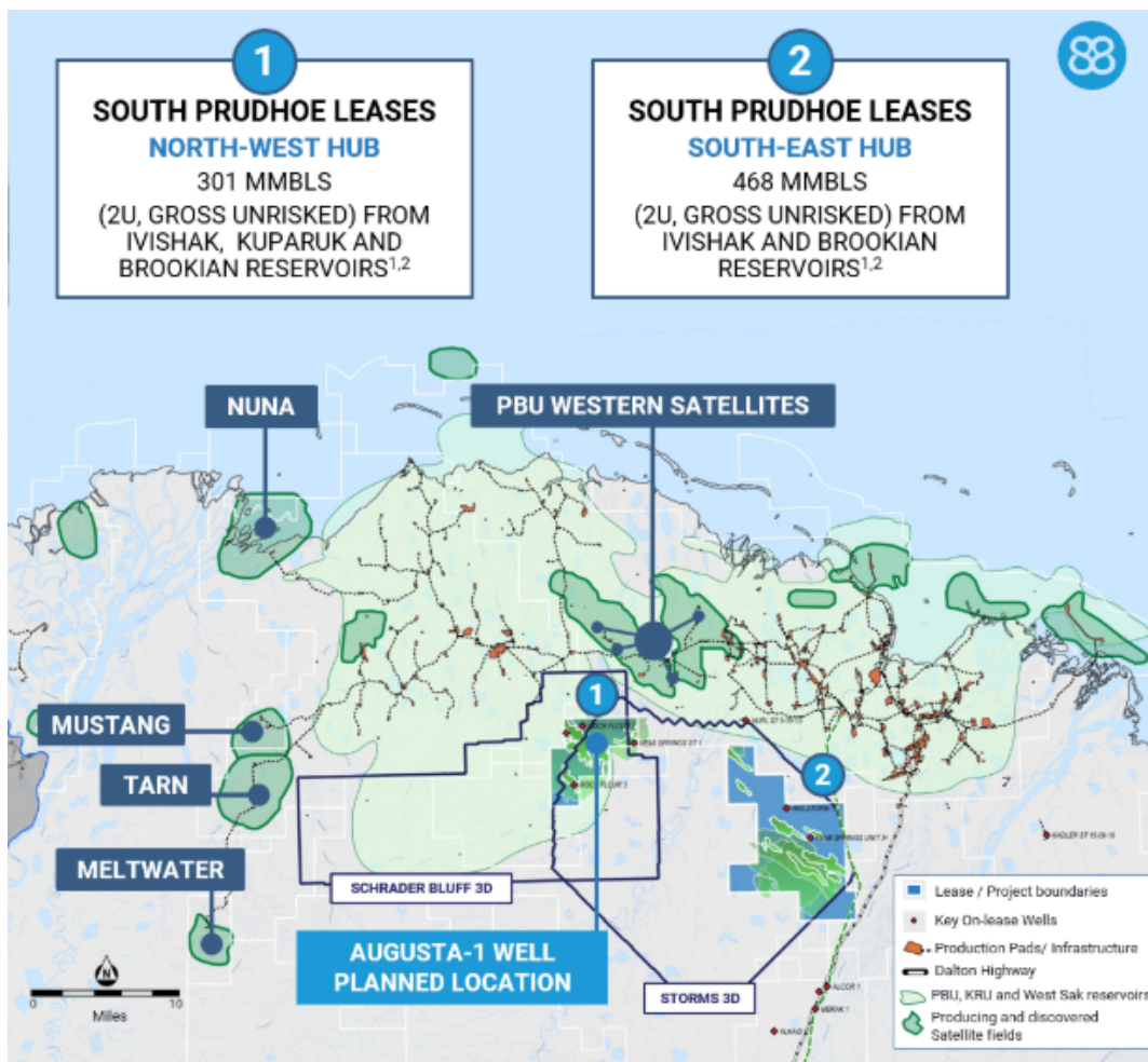
Figure 1: 88 Energy's North Slope position showing the planned location of the Augusta-1 exploration well.
