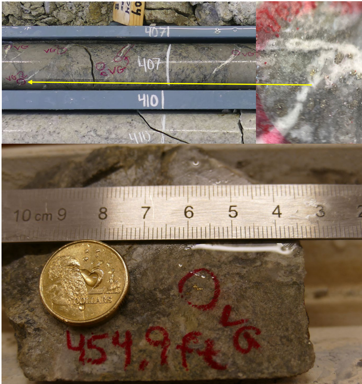
Image 2: Top: 26FRD001 HQ3 core (uncut) centred at approximately 407ft (124.1m) downhole showing multiple visible native gold grains (main photo, with close-up inset at right) associated with pervasively sericite altered brecciated metasediment near quartz-carbonate veining and pyrite mineralisation. Bottom: 26FRD001 HQ3 core (cut) at approximately 455ft (138.7m) downhole showing visible native gold blebs associated with sericite altered brecciated metasediment near boudinaged quartz-carbonate veining and pyrite mineralisation. Bottom image scale shown in cm/mm with a 20.5mm diameter coin; no scale in top images.
