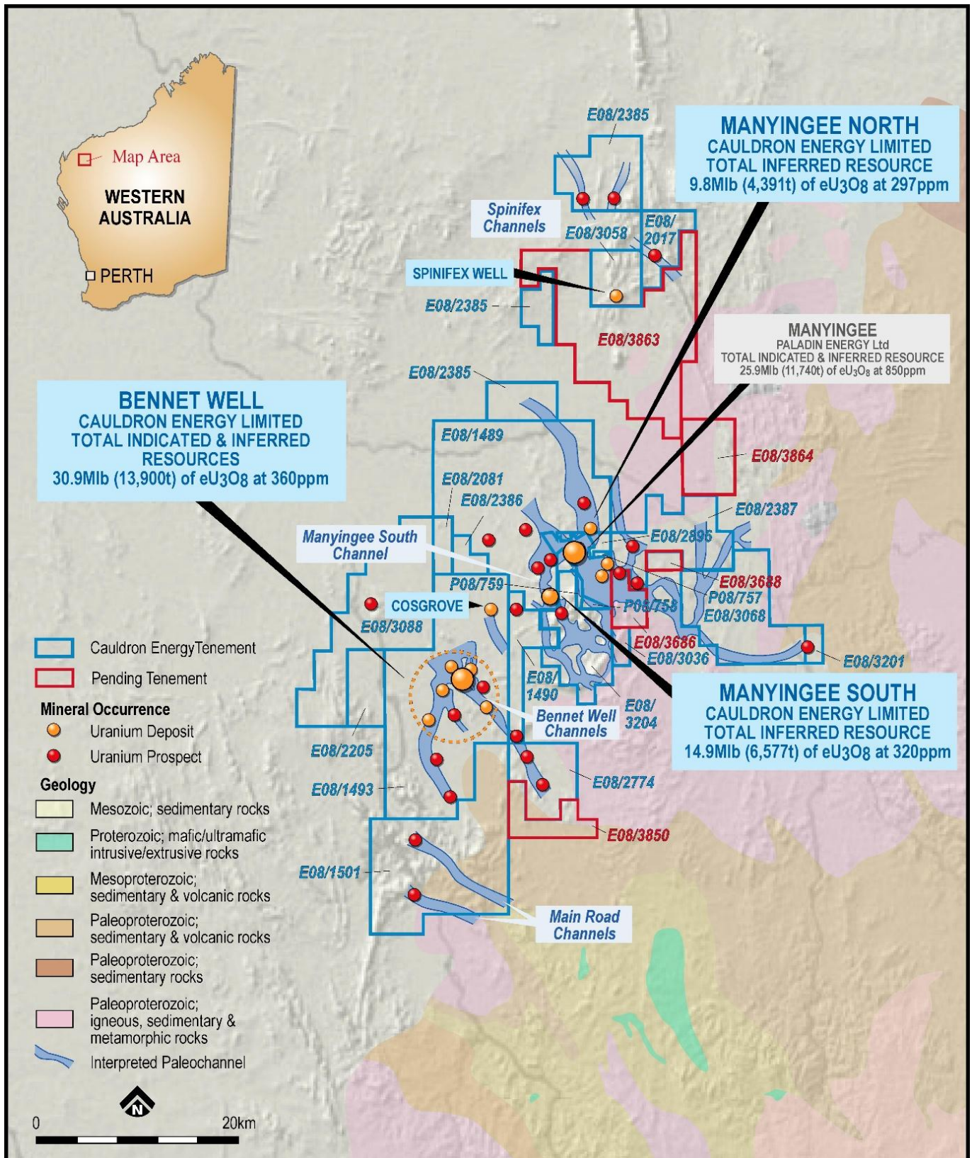
Figure 1. Yanrey Project tenements showing regional geology.
