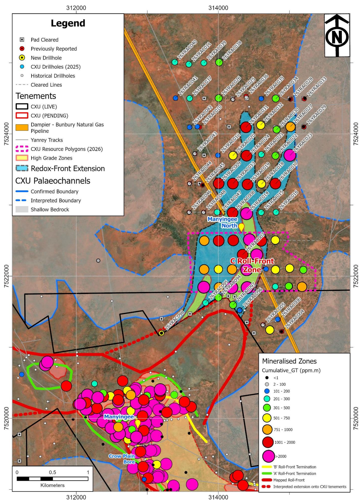
Figure 10. Manyingee North Cumulative GT (ppm*m) map showing the continuation of the Manyingee redox-front.
