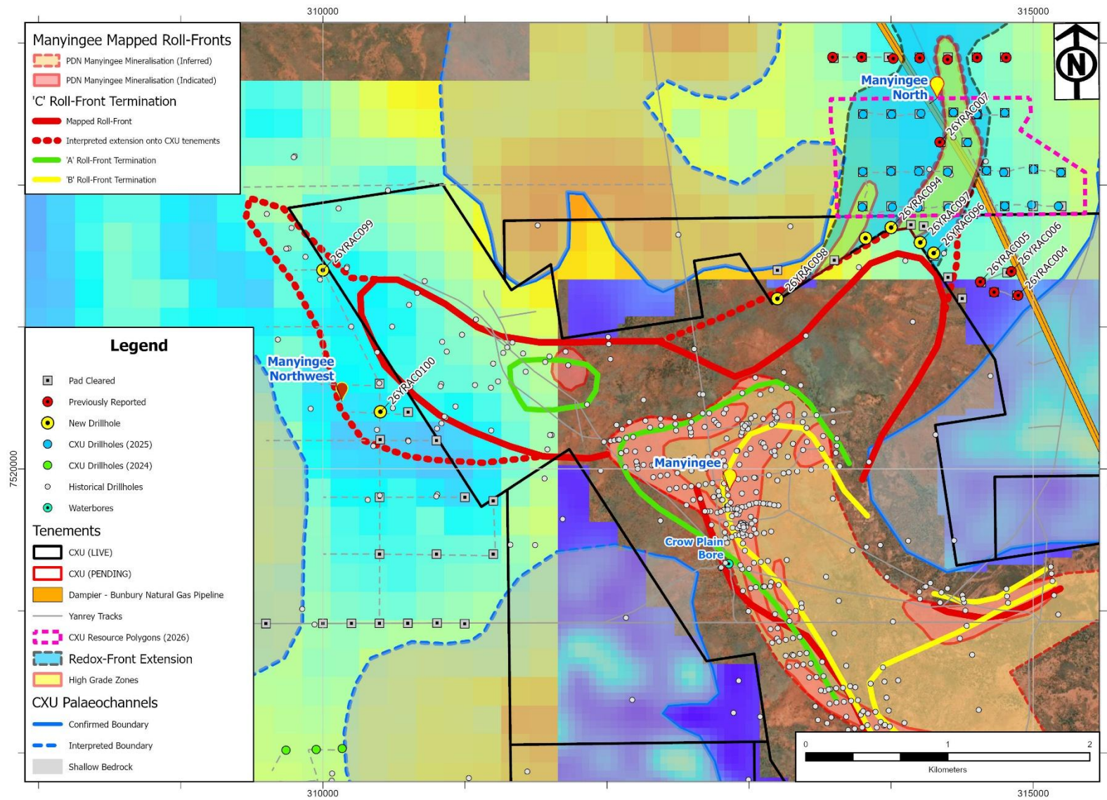
Figure 9. Manyingee South passive seismic interpreted depth to bedrock map showing drillhole locations.
