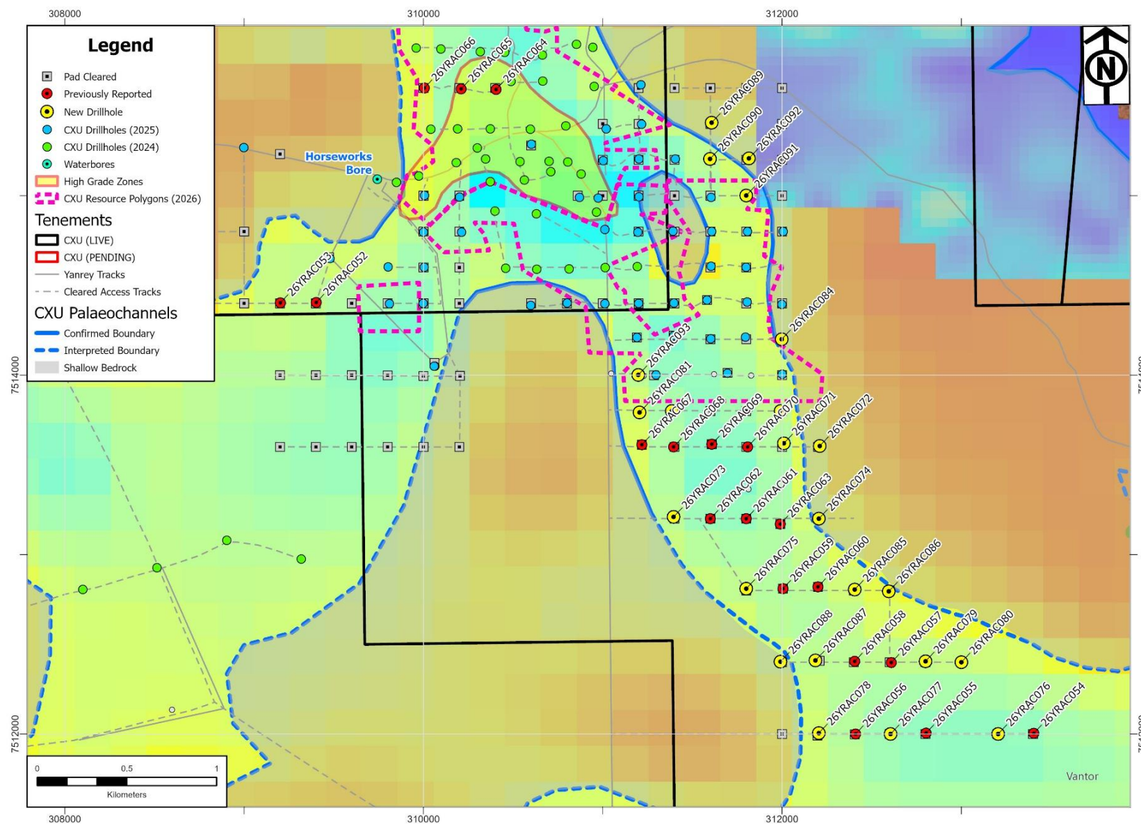
Figure 7. Manyingee South passive seismic interpreted depth to bedrock map showing drillhole locations.
