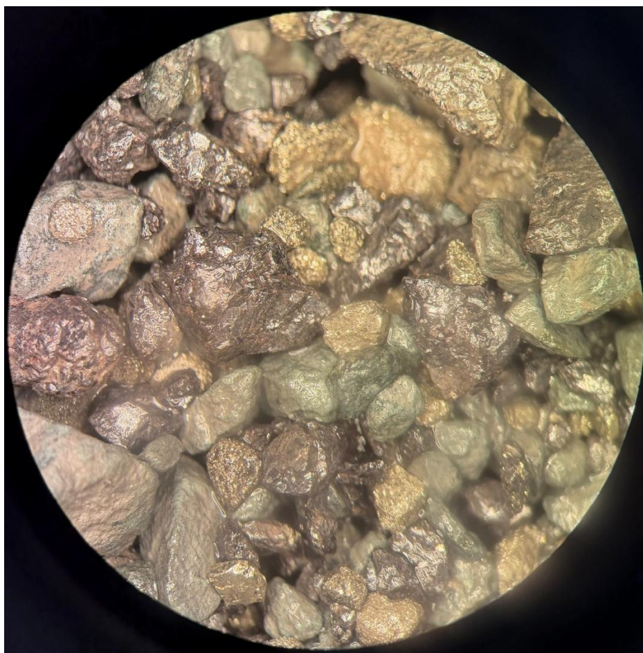
Figure 2: Photograph of mineralisation typical between logging interval 9.14m and 15.24m where massive black-brown sphalerite and brassy yellow pyrite can be observed. Mineralisation in the photograph returned 3.05m @ 29.5% Zn from 12.19m in drillhole SPC26001.
