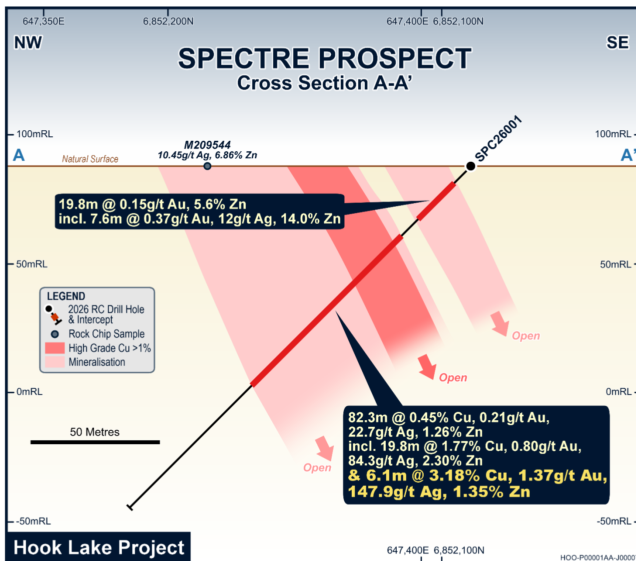
Figure 4: Cross section illustrating drillhole SPC26001 and the >80m of vertical continuity now established below the surface showings sampled in 2025.
