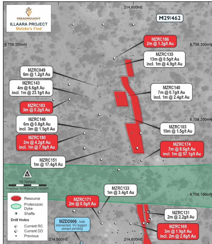
Figure 3: Inset plan view map of Metzke's North showing the break in mineralisation due to a Proterozoic dyke in relation to current and previous drilling.
