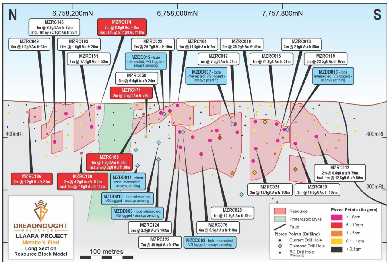
Figure 4: Long section of Metzke's Find/North showing the location of drill intercepts in relation to the current Resource outline.
