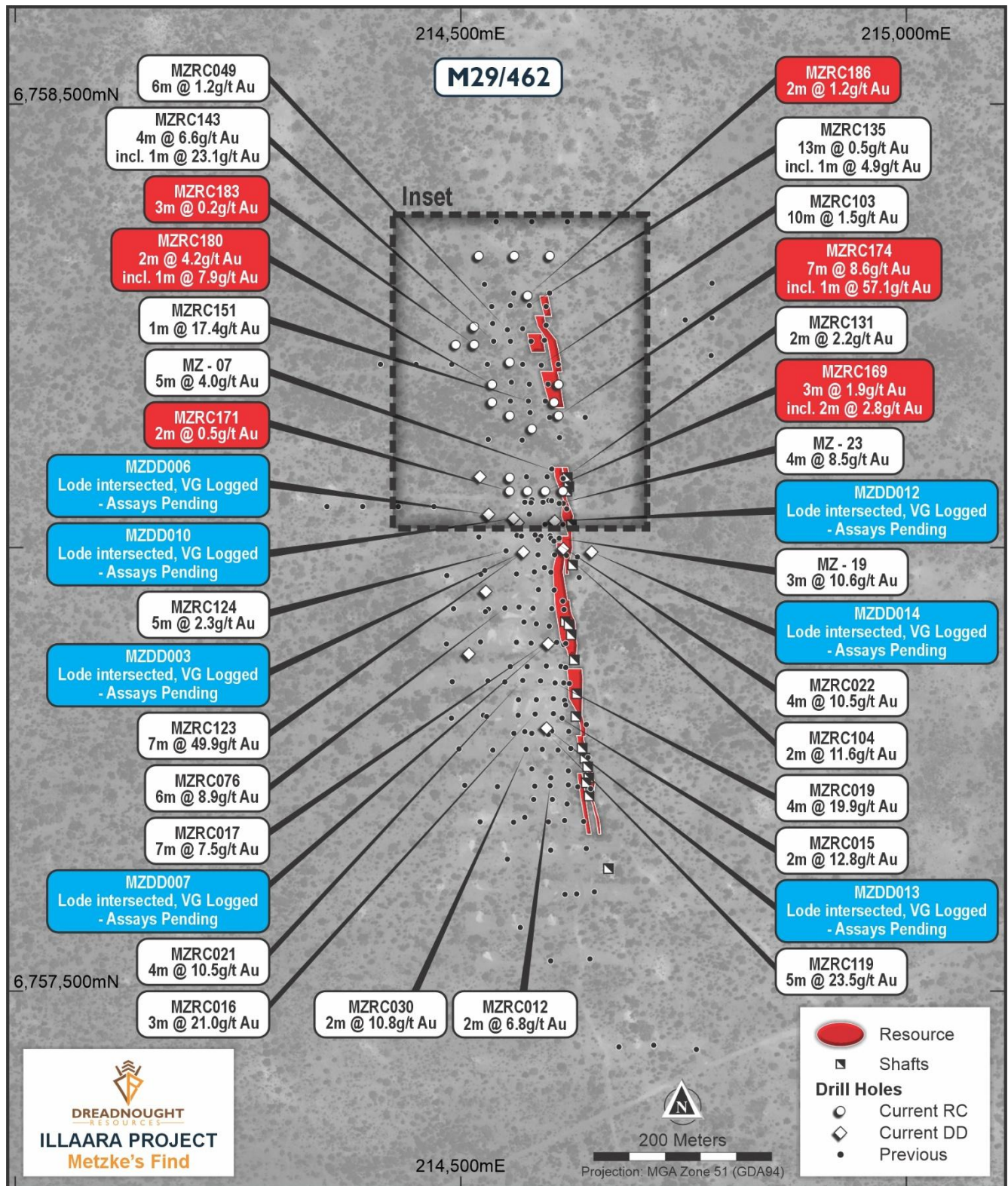
Figure 2: Plan view map of Metzke's Find and Metzke's North showing: the break in mineralisation due to a Proterozoic dyke; the location of the RC program mainly at Metzke's North (boxed area); the diamond program at Metzke's Find all in relation to previous drilling and the Metzke's Resource (24,900 oz @ 5.2 g/t Au - 84% Indicated).
