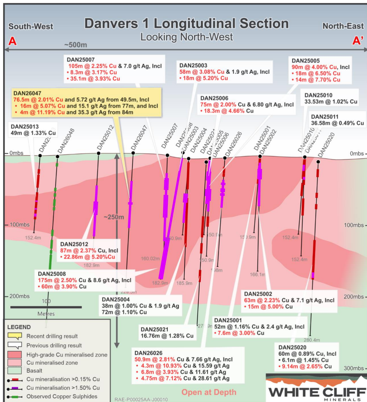
Figure 01 - Longitudinal section through Danvers 1 showing grade continuity and exceptional results across a approx. 500m strike length, which now represents just a fraction of the total drill confirmed strike length within the broader Danvers 1 and Teshierpi Fault Zone. DAN26048 has returned observations of copper sulphides below previously reported assay results, materially extending mineralisation to depth at Danvers 1.
