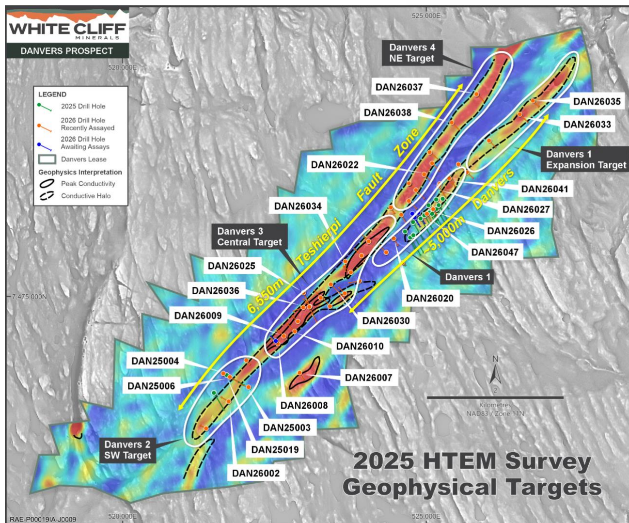
Figure 06 - Plan view map of the 2025 HTEM conductivity basemap and drilling completed along the Teshierpi Fault Zone and Danvers 1 trend. Mineralisation remains open along strike to the NE and SW, with several high-priority targets still untested by drilling along this >11.5km combined strike length.
