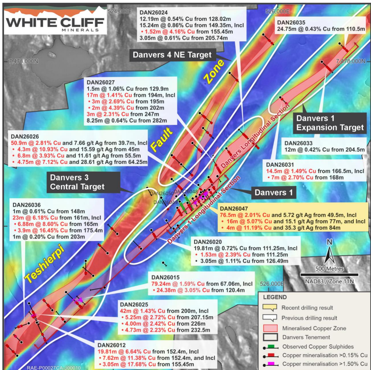
Figure 05 - Plan view map of the rapidly expanding Danvers District, highlighting the 76.5m @ 2.01% Cu from Danvers 1 infill hole DAN26047 and position of DAN26048-050 that returned visible copper sulphides below historic and 2025 drilling at the southwestern end of the core of Danvers 1.
