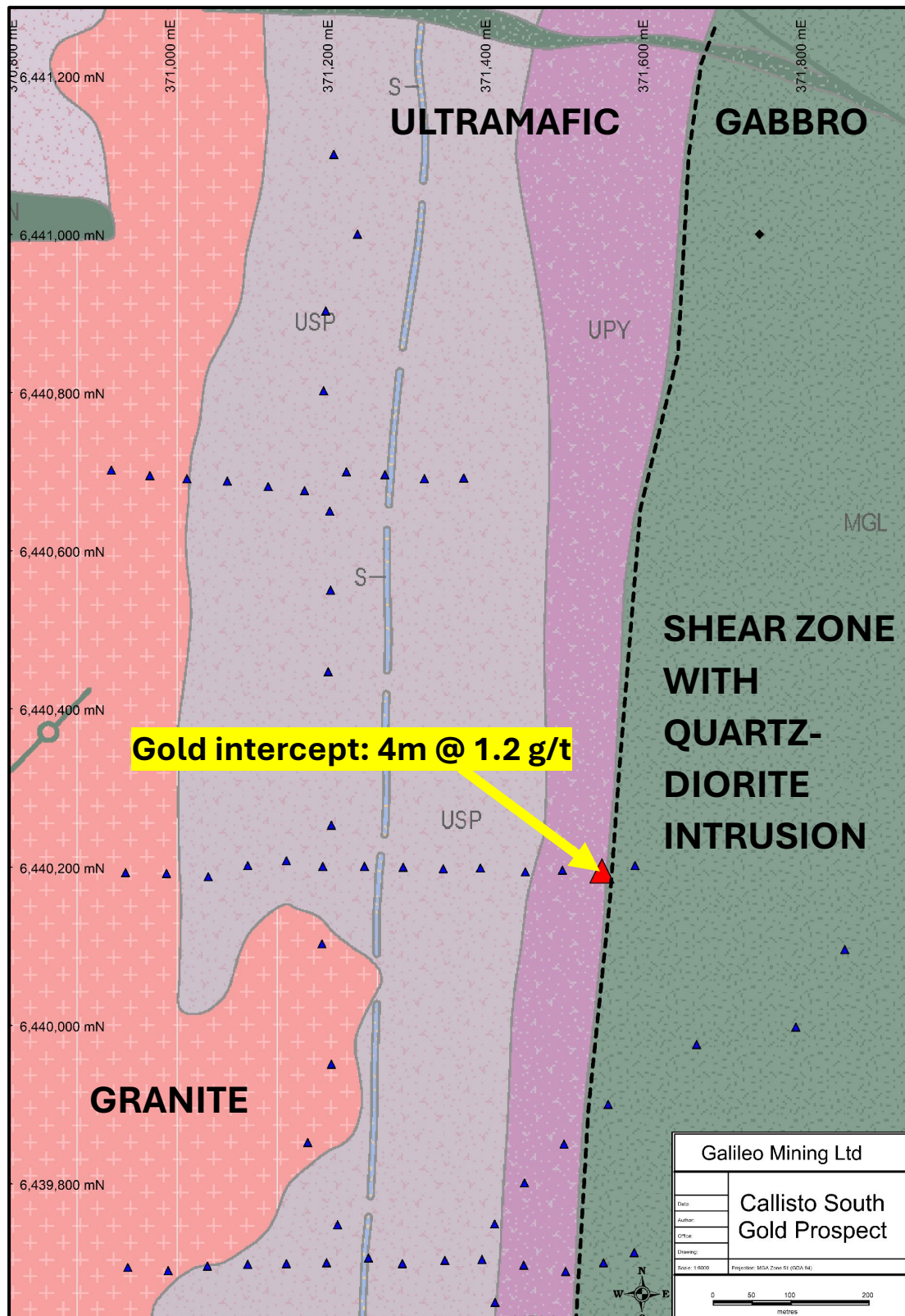
Figure 4 – Callisto South gold prospect with air core drilling (triangles), gold drill intersection, 10k mapped geology and interpreted shear zone. See ASX announcement dated 10 th August 2026 for further details.
