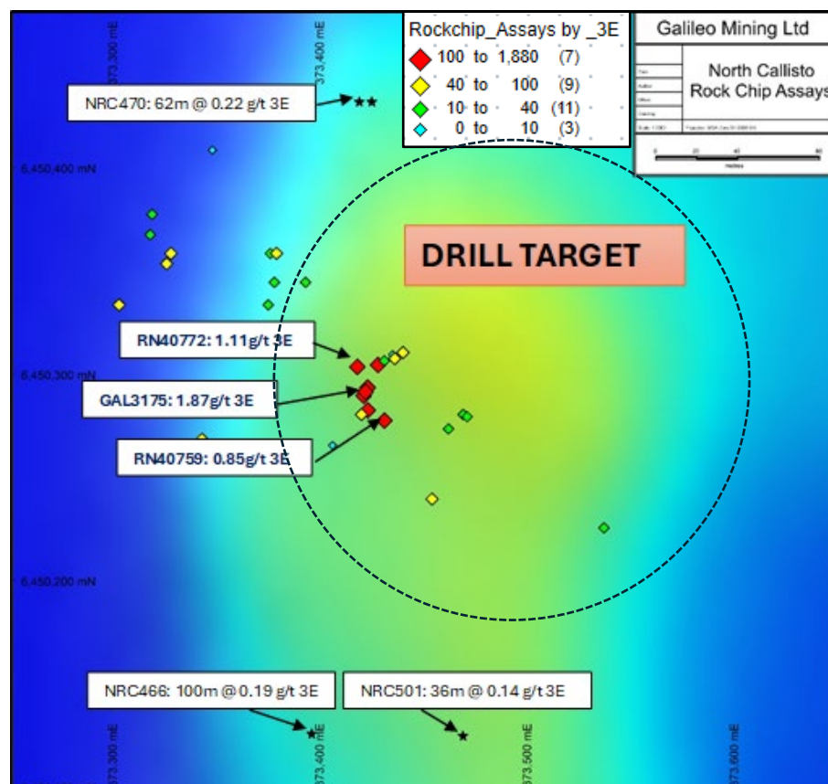
Figure 2 – Rock chip sampling from North Callisto prospect with anomalous drilling to north and south (black stars) and current drill target area (dotted ellipse). TMI magnetic background.
