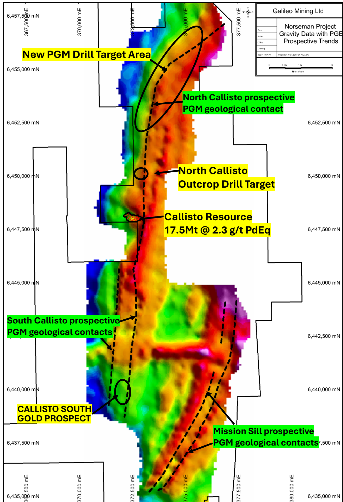
Figure 3 – Norseman Project residual gravity image with existing Callisto resource, new drill target at North Callisto, and additional PGM and gold targets in the current drill program.
