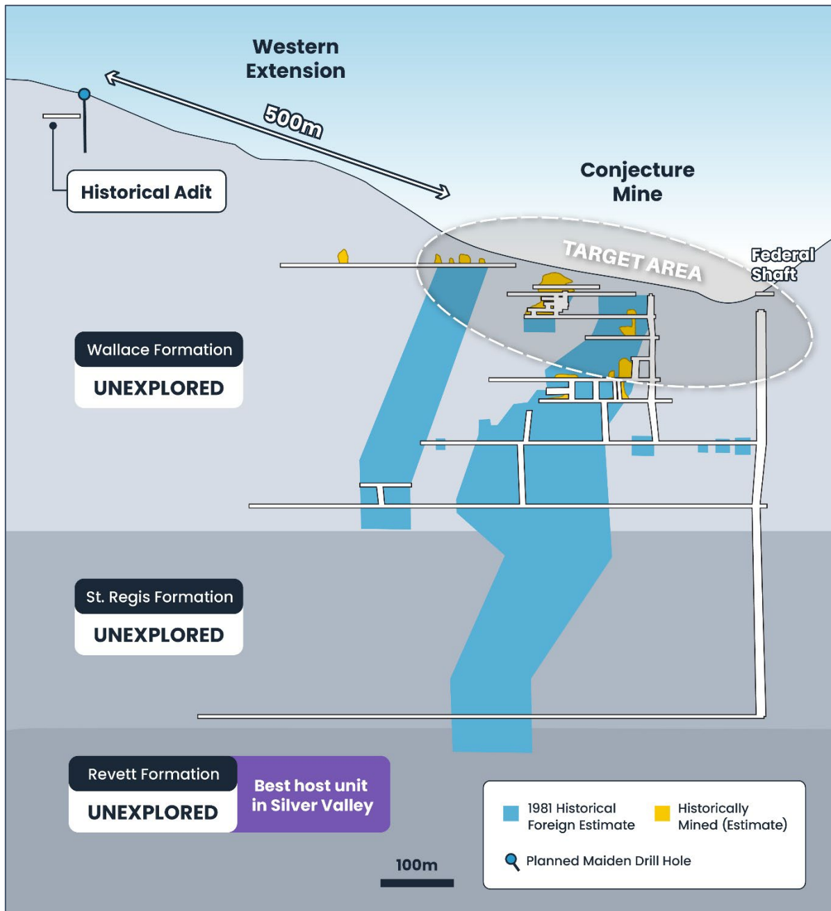
Figure 1: Conjecture Mine schematic long section (looking north-west) showing inferred geological boundaries, historically mined areas, the 1981 historical foreign estimate and the planned trace of the first drill hole 1
