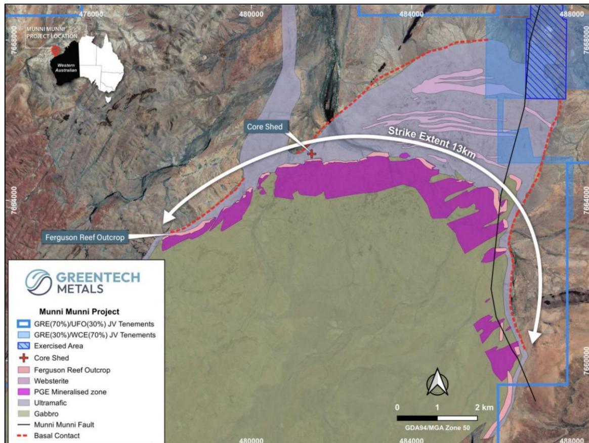
Figure 2: Northern extent of the Munni Munni intrusion showing basal contact target.
