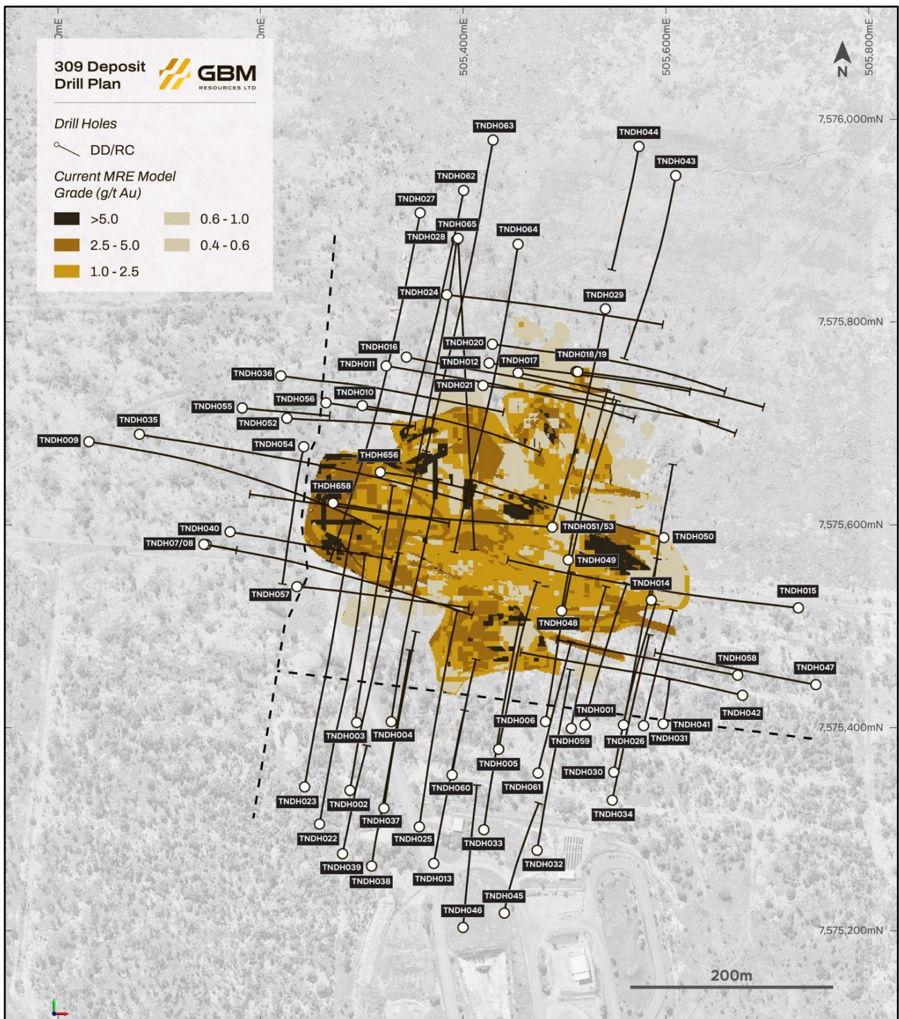
Figure 3 – Plan view of 309 Deposit with completed Stage 1 and 2 drill holes.
