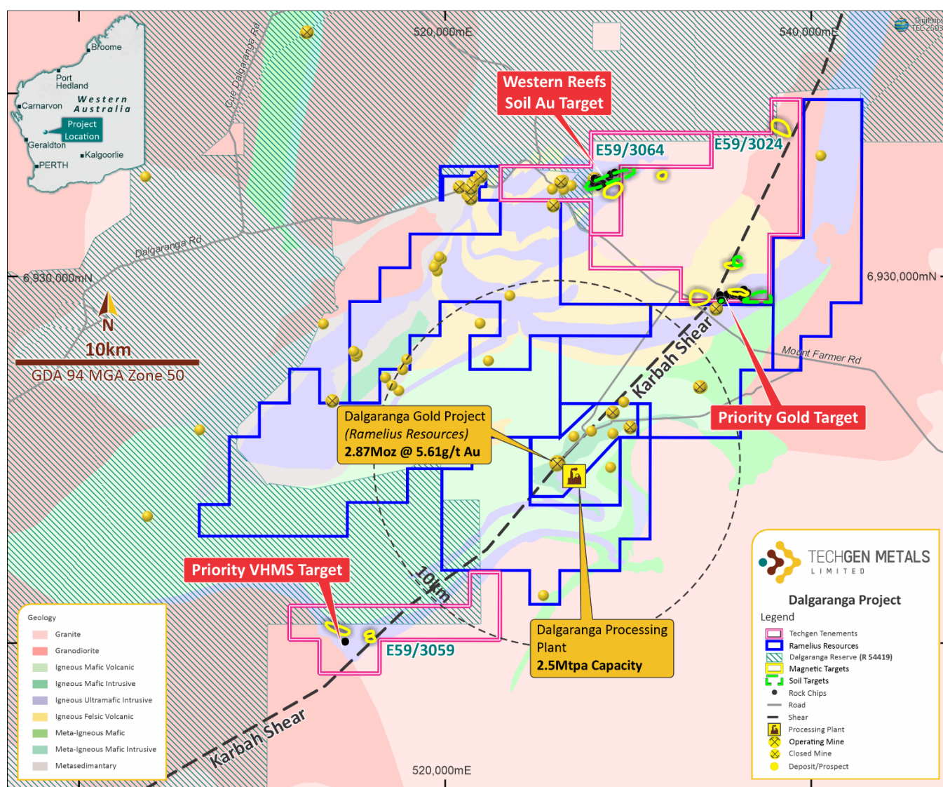
Figure 1: The Dalgara Gold Project over geology.
