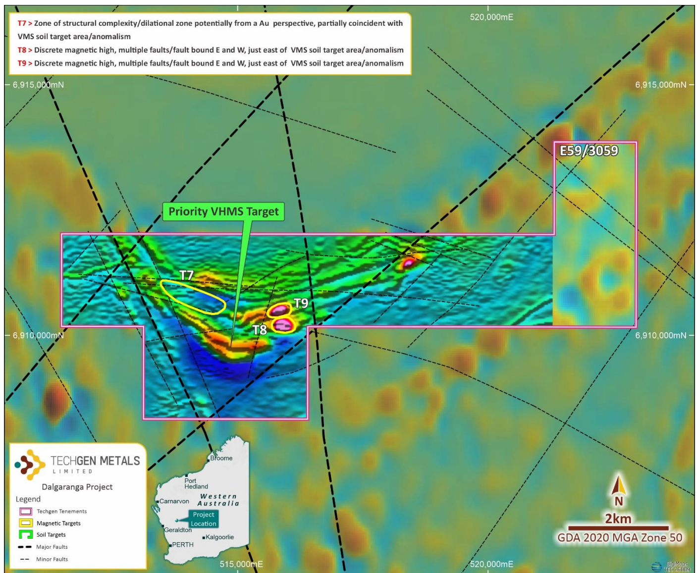
Figure 3: Target areas at the Dalgara Gold Project (Southern Area).
