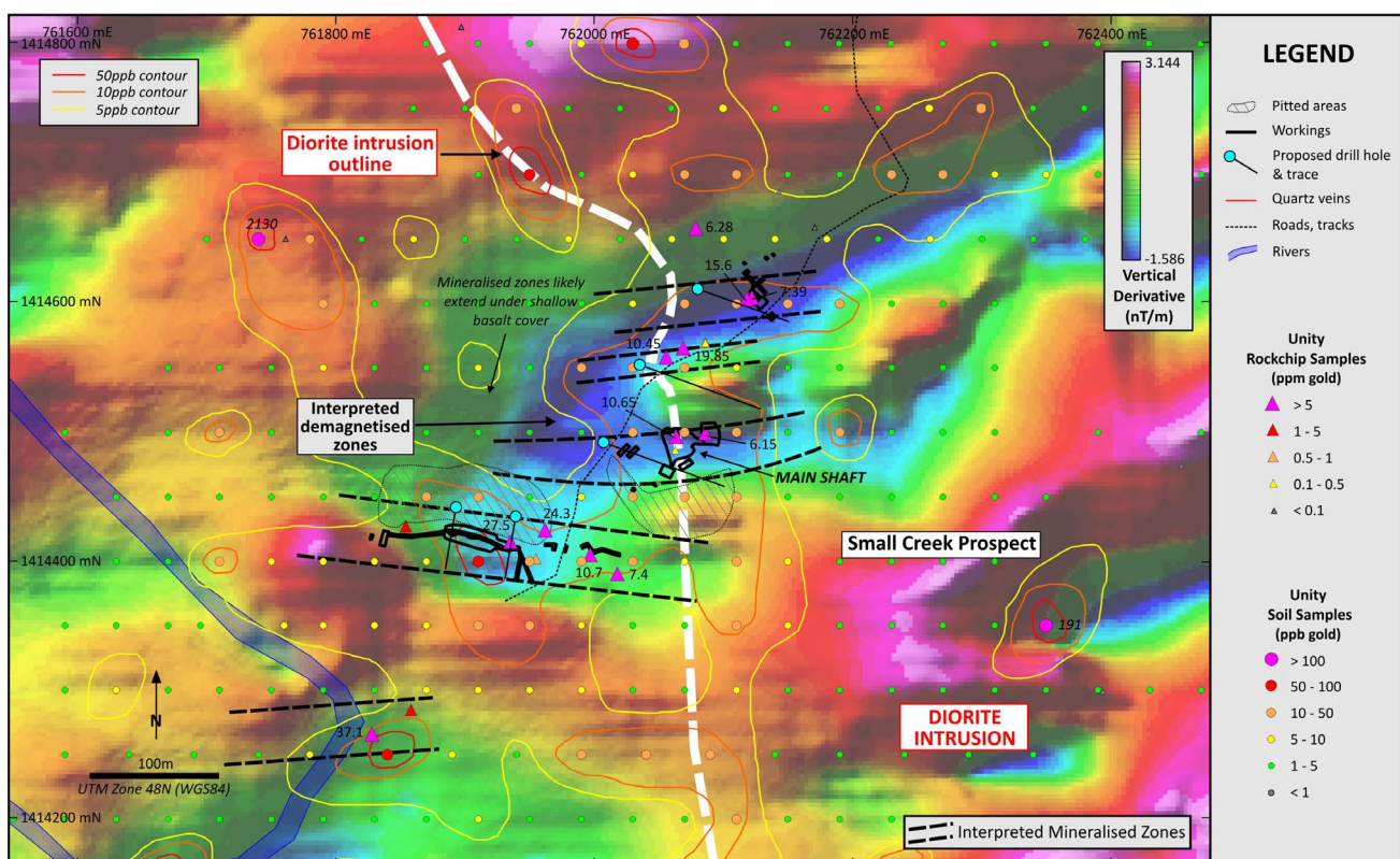
Figure 4: Historical gold mine workings and gold-in-soil sample results on a UAV magnetics image (1VD Tilt 60°) at the Small Creek Prospect. The NE-ENE trending magnetic lows in blue (interpreted demagnetised zones) associated with the areas of historical mine workings are clearly evident.
