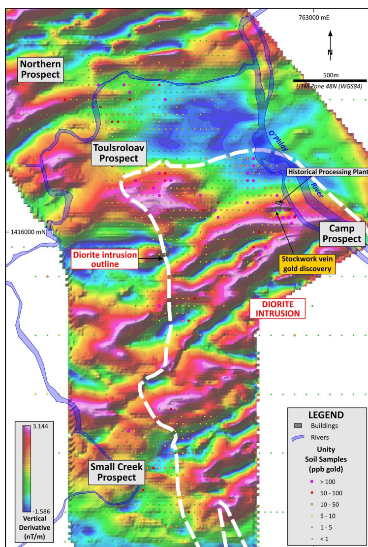
Figure 5: UAV magnetics image (1 st VD Tilt 60°) from O'Phlay showing the stacked NE-ENE trending magnetic anomalies & demagnetised zone targets that extend across the top of a diorite intrusion with gold-in-soil results and prospect locations.
