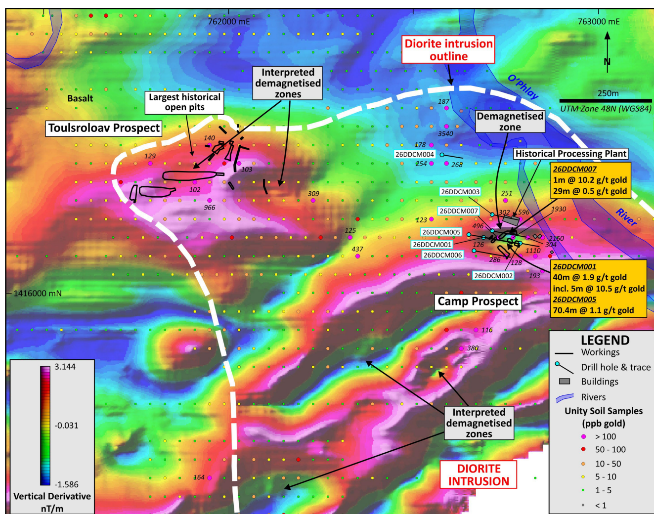
Figure 3: Historical gold workings and gold-in-soil sample results on a UAV magnetics image (1VD Tilt 60°) at the Camp and Toulouloav prospects. Magnetic lows in blue-yellow (interpreted demagnetised zones) associated with the areas of historical mine workings and the stockwork gold discovery are evident. Completed drill holes are depicted.
