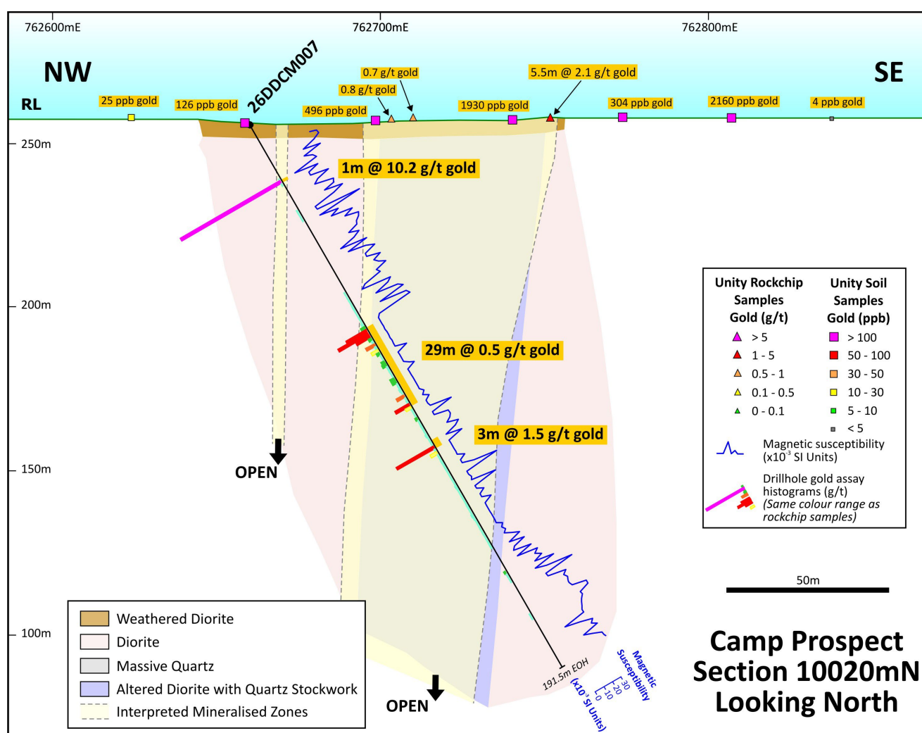
Figure 1: Drilling Cross Section 10,020mN with hole 26DDCM007 at Camp Prospect with gold intersections, magnetic susceptibility readings and a geological interpretation.
