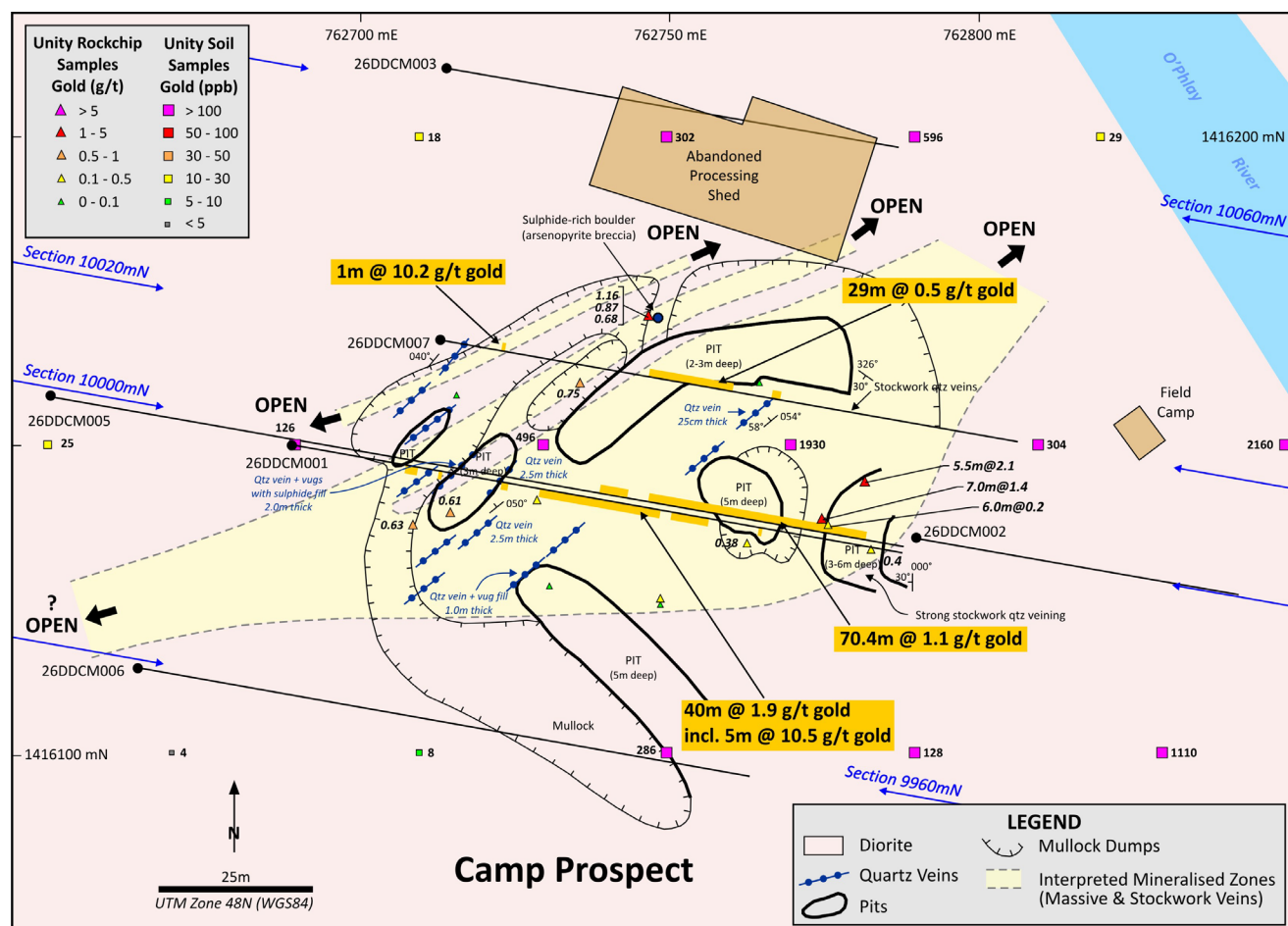
Figure 2: Location of the broad gold mineralised stockwork vein zone discovered in the eastern portion of the Camp Prospect showing drill holes, historical mine workings, soil sample gold results & rock chip sample gold results on geological mapping.
