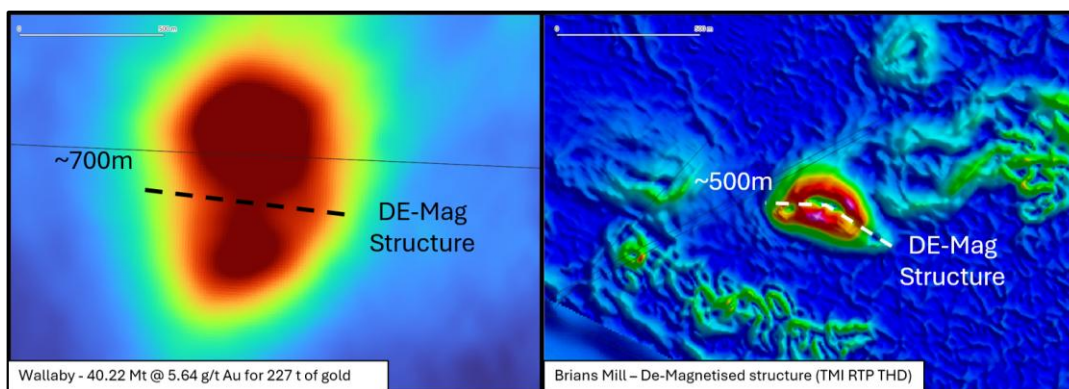
Figure 3 – Magnetic geophysics (TMI RTP) and satellite imagery comparing Wallaby (Gold Fields, left) and Brians Mill (Parbo, right)
