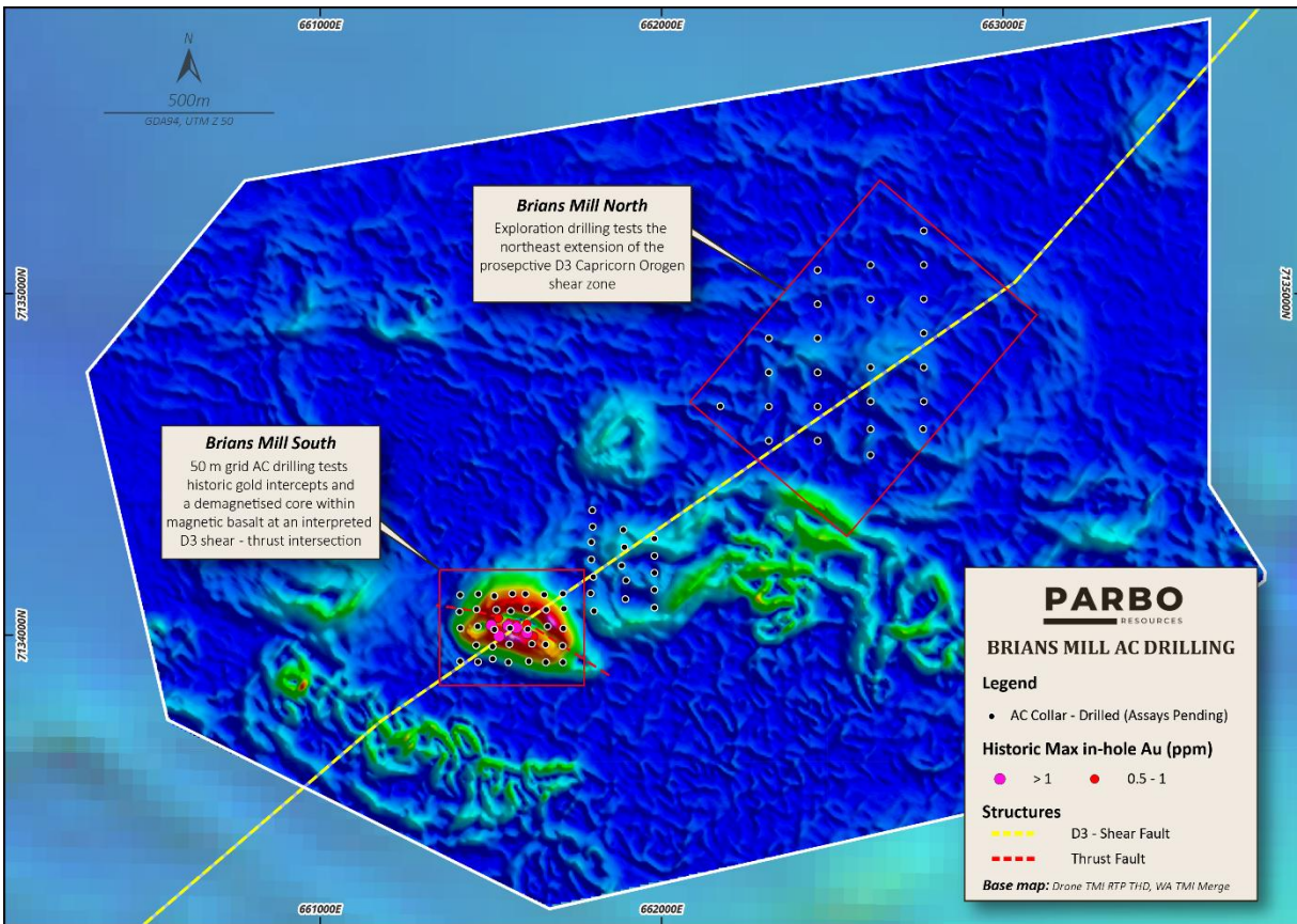
Figure 2 – Brians Mill drone magnetics (TMI) showing Parbo's 2026 AC collars (Brians Mill South and North), historic drilling, interpreted structures and previously reported historic intercepts 1
