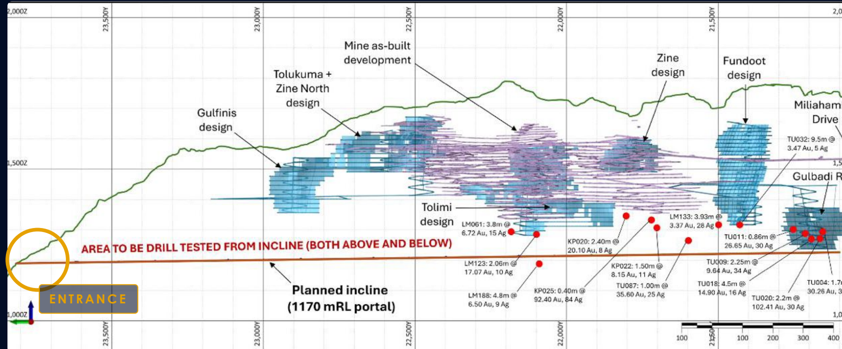
Tolukuma incline & gravity dewatering (long section) — commencement Q1 2027. Graphic: Dec 2025 "Tolukuma Operations & Development Update".
