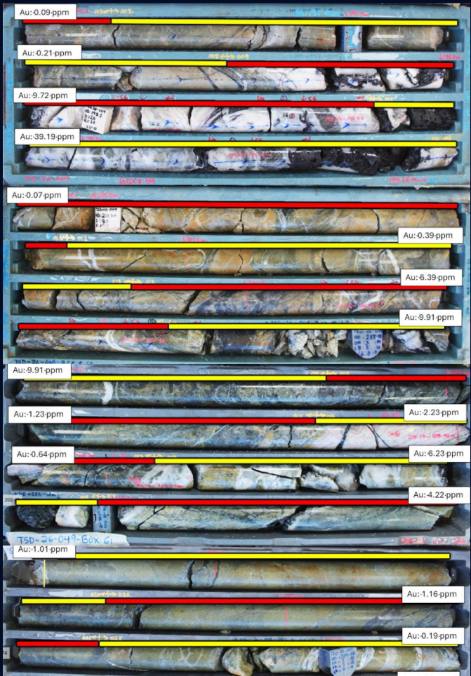
Diamond core, TSD-26-049 (boxes 59–61) — gold assays in ppm (120 Vein)
