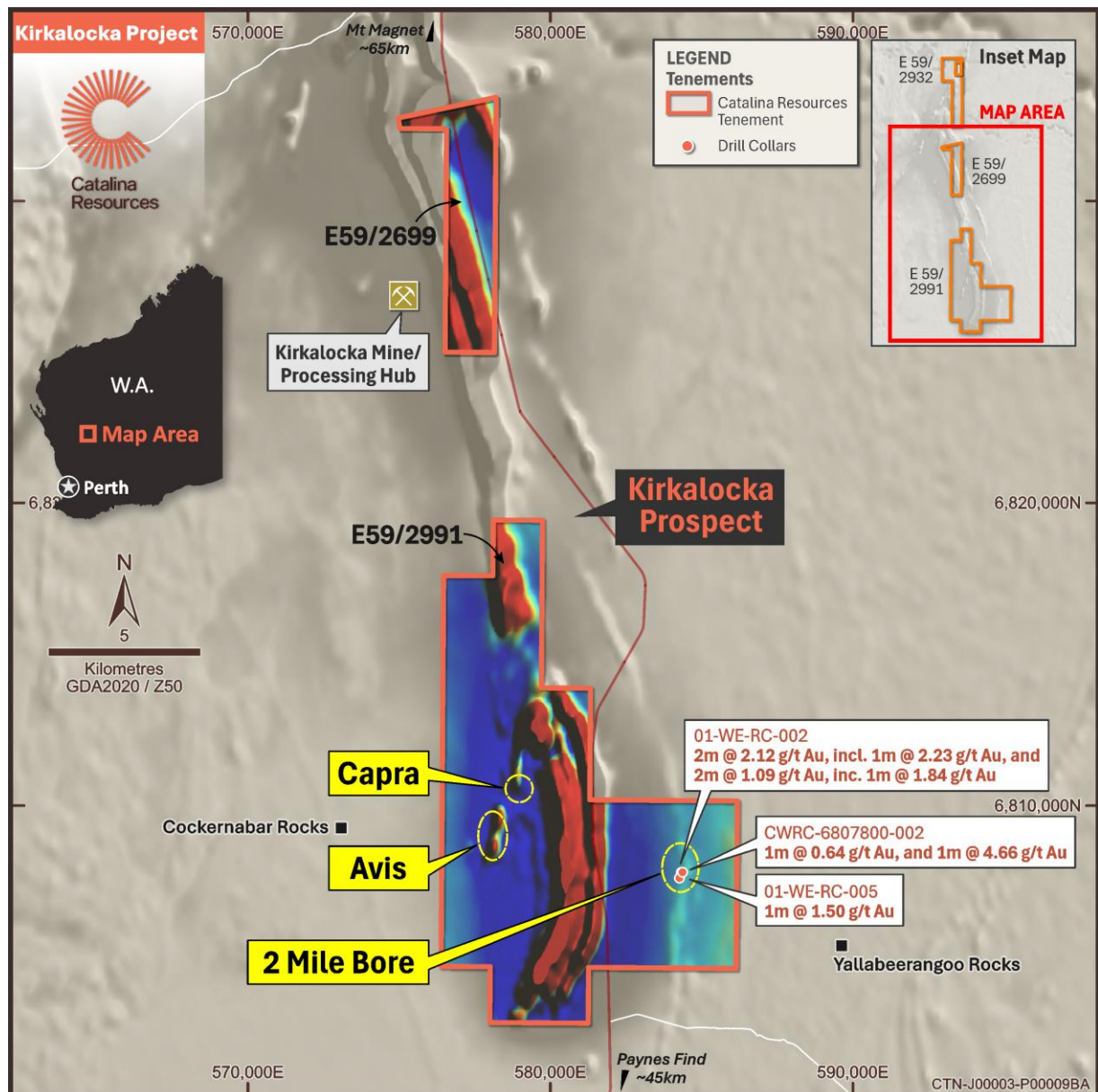
Figure 1: Kirkalocka project 2 with identified high-priority prospects Capra, Avis and Two Mile Bore.
