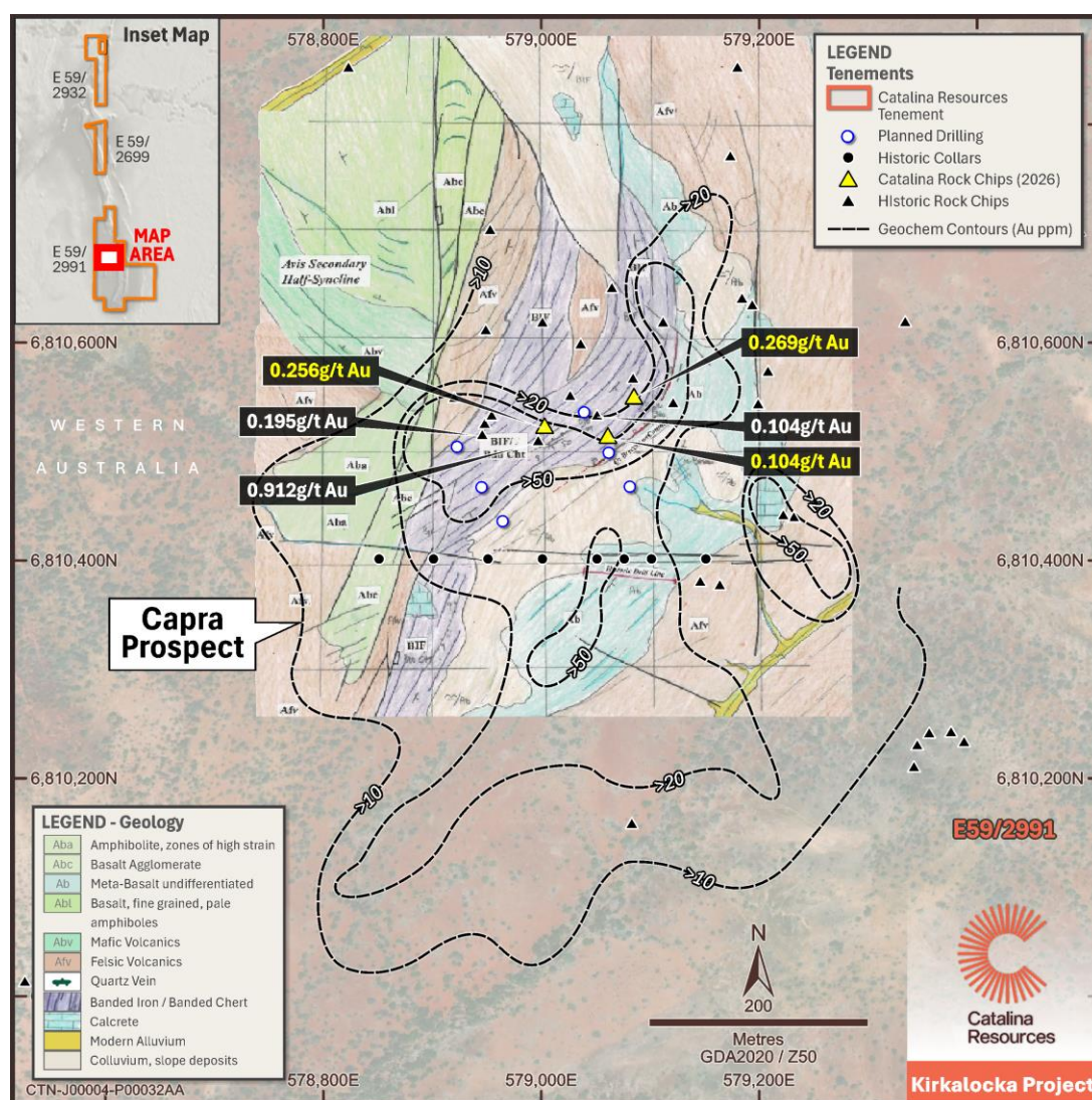
Figure 2: Geological map of Capra illustrating Au soil contours, rock chip results and planned drilling. (Only historical rock-chip samples grading >0.1 g/t Au are labelled)
