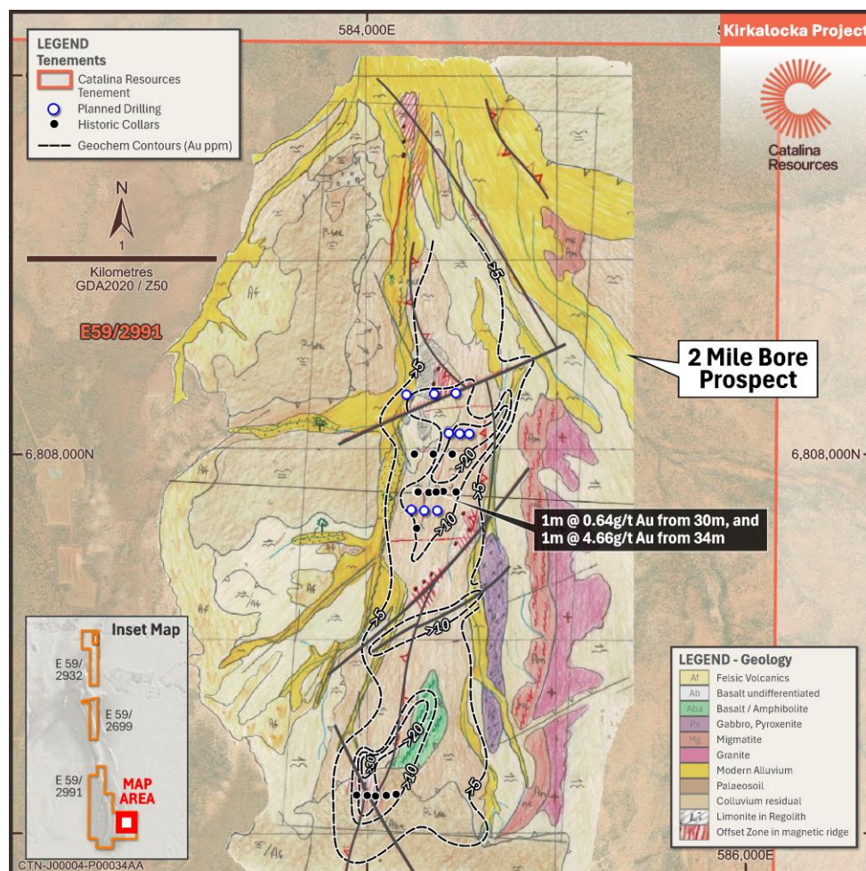
Figure 4: Geological map of Two Mile Bore illustrating Au soil contours, rock chip results and planned drilling.
