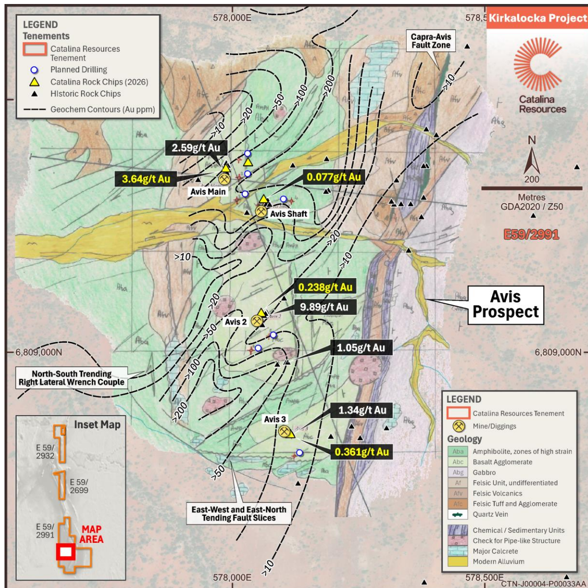
Figure 3: Geological map of Avis illustrating Au soil contours, rock chip results and planned drilling. (Only historical rock-chip samples grading >1 g/t Au are labelled)
