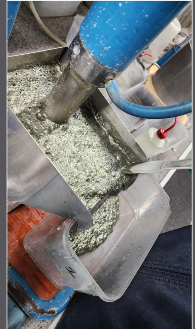
Flotation Testwork on Maronan Copper-Gold samples being conducted at AMML Lab in Gosford
