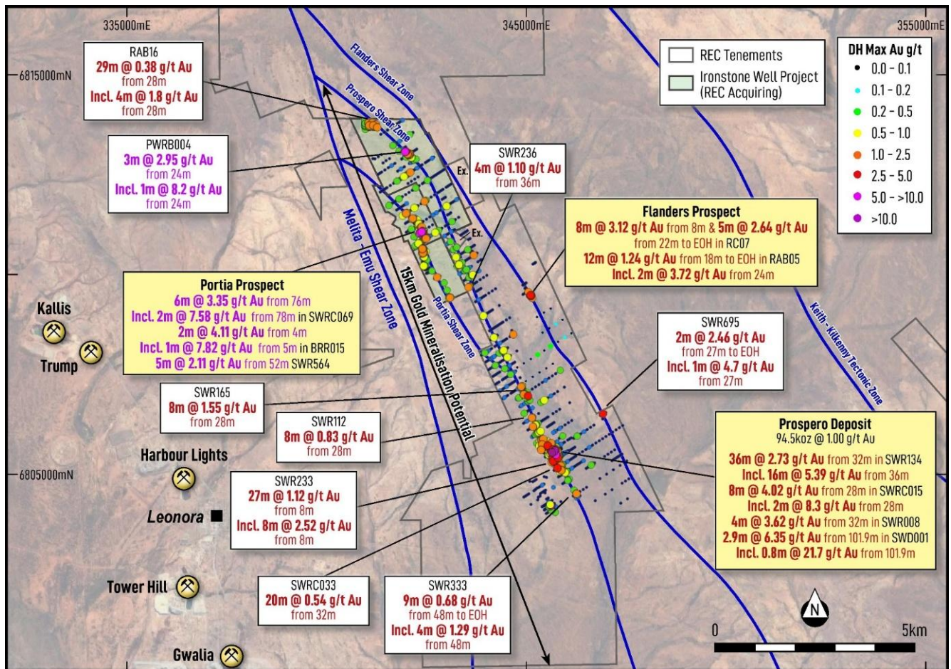
Figure 2: The greater Prospero trend showing high-tenor gold results with minimal follow up and not drilled since the mid 1990s
