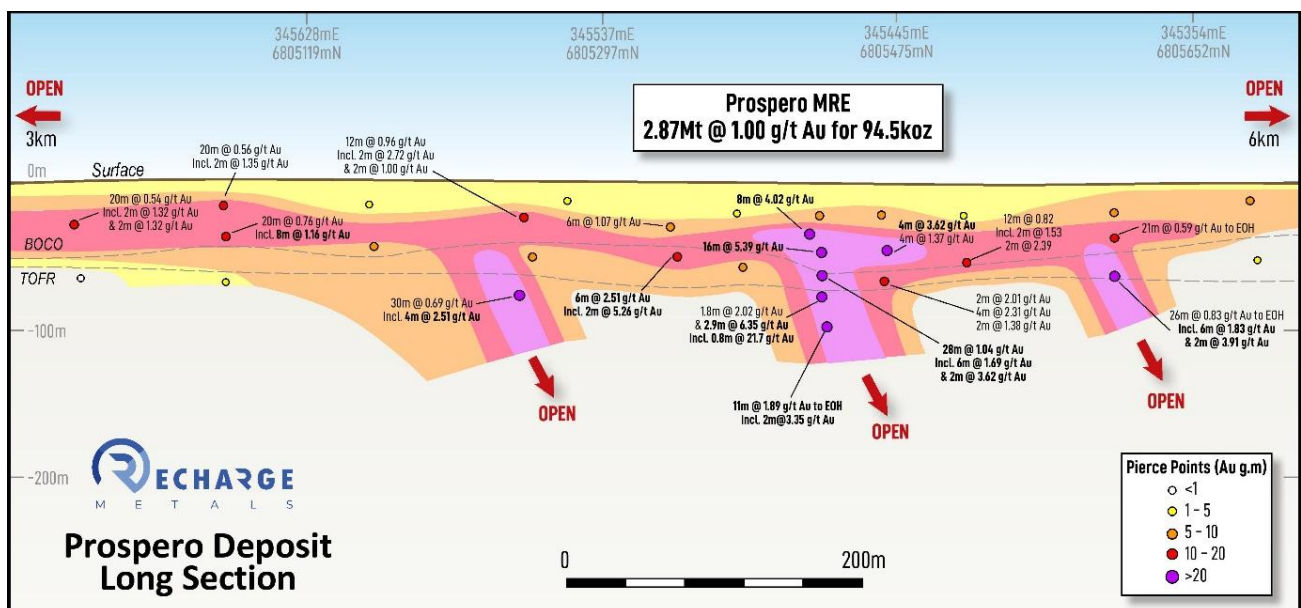
Figure 3: Longitudinal section through the Prospero Gold Deposit showing high-grade shoots and only three holes drilled below 100m vertical depth
