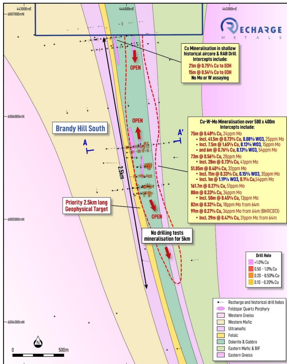
Figure 4: Past drilling at BHS targeting 500m of a 2.5km long low amplitude magnetic anomaly (red dashed polygon)
