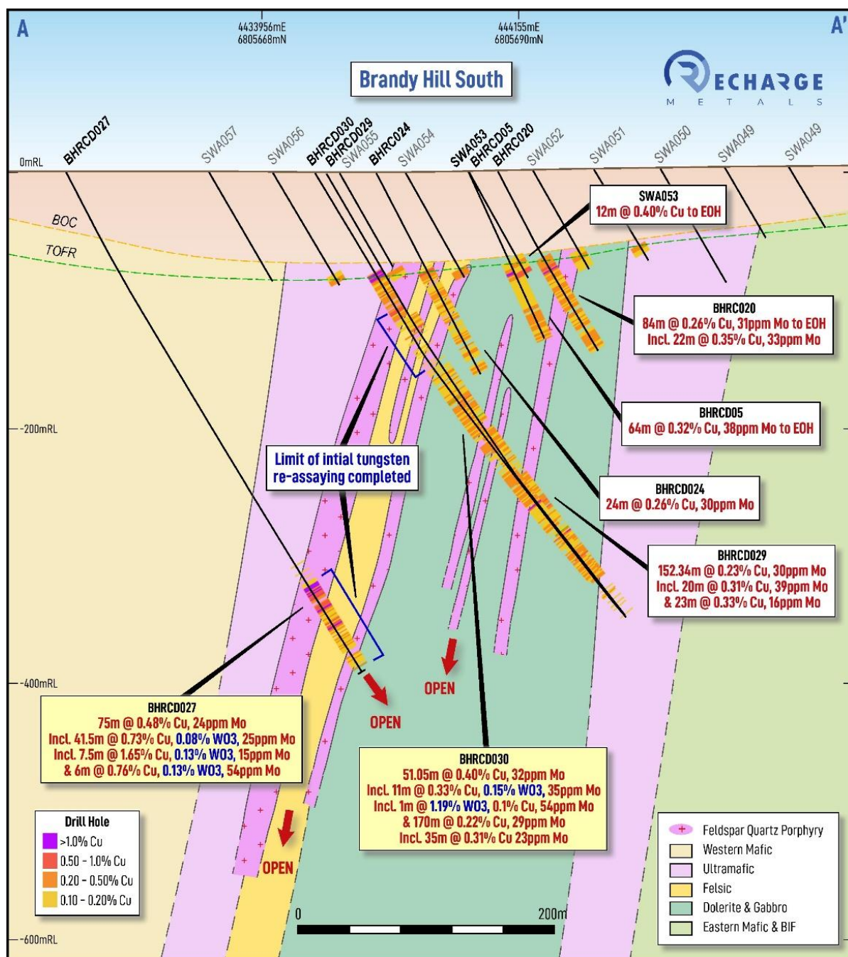
Figure 5: Cross section through BHS showing the mineralised package of rocks is approximately 250m wide
