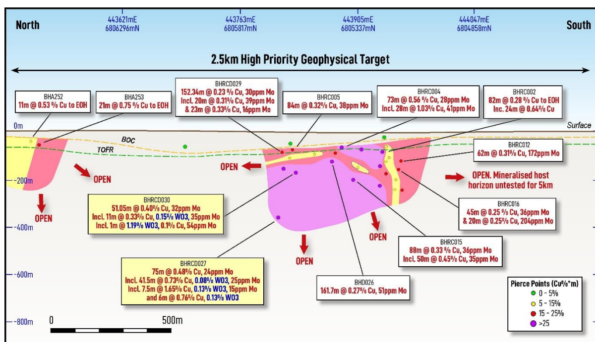
Figure 6: Longitudinal section through BHS showing 500m x 400m x 250m area drilled in 2021/2022 and 21m at 0.75% Cu intercept located 1km to the north
