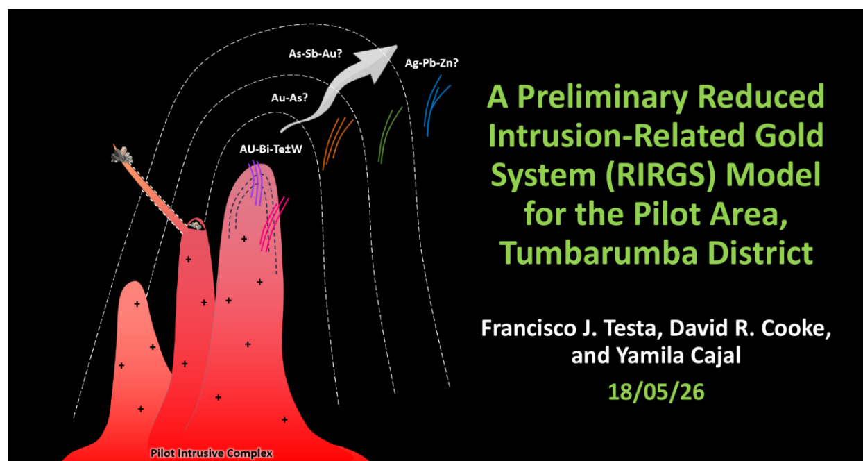
Figure 10: RIRGS metal zonation model for Pilot, showing conceptual Au-Bi-Te-W proximal to the intrusive centre grading to Ag-Pb-Zn at distal margins.
