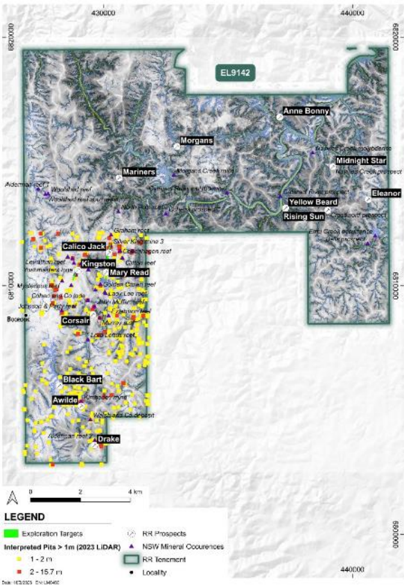
Figure 12: LiDAR interpretation for EL9142 showing significant historical workings in relation to the two exploration targets.
