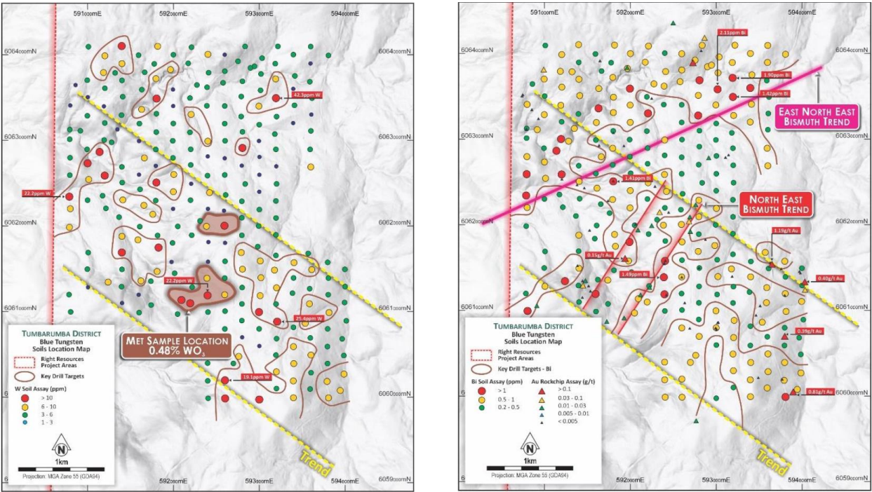
Figure 7: Comparison of laboratory tungsten (W) and bismuth (Bi) soil geochemistry and gold rock assays showing northwest, northeast and east-northeast trends at Blue Prospect
