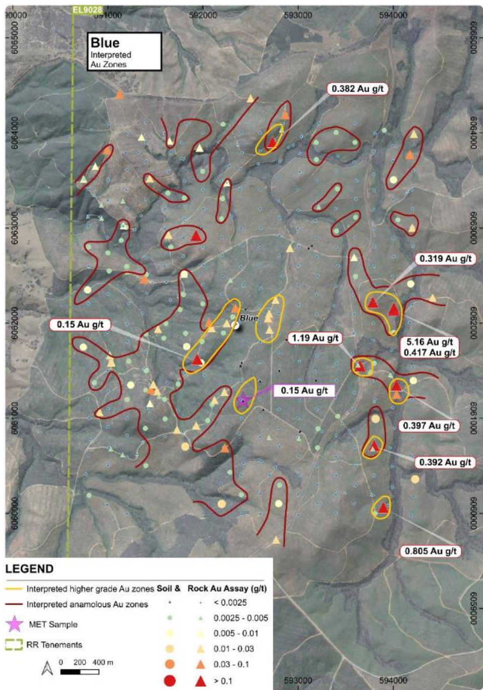
Figure 8: Blue prospect showing interpreted soil and rock gold anomalies
