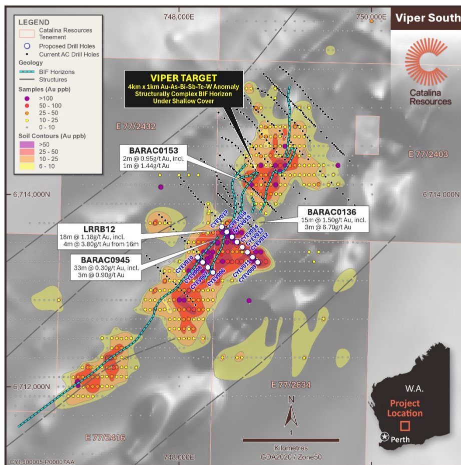
Figure 12: View of the Viper Prospects illustrating the interpreted extent and orientation of gold mineralisation based on Phase 1 RC drilling, historical drilling data, and current geological interpretation
