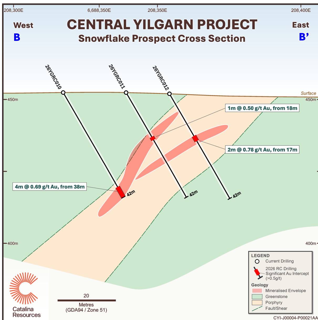
Figure 8: On the southern Snowflake drill section (YGR010–YGR012), drilling intersected narrow zones of low to moderate gold mineralisation at shallow depth, with a broader intersection in YGR010, and the geometry of mineralised intervals suggests the potential presence of more than one mineralised system (Section B).
