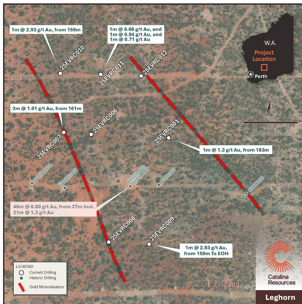
Figure 11: View of the Leghorn Prospect illustrating the interpreted extent and orientation of gold mineralisation based on Phase 1 RC drilling, historical drilling data, and current geological interpretation
