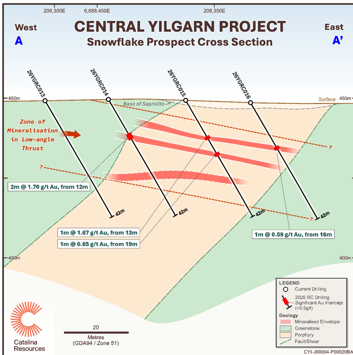
Figure 7: An alternative interpretation suggests gold mineralisation may be controlled by a shallow-dipping thrust structure rather than stratigraphy-parallel shear zones. In this model, the thrust is interpreted to potentially surface to the west prior to YGR013. This interpretation remains conceptual and untested (Section A)
