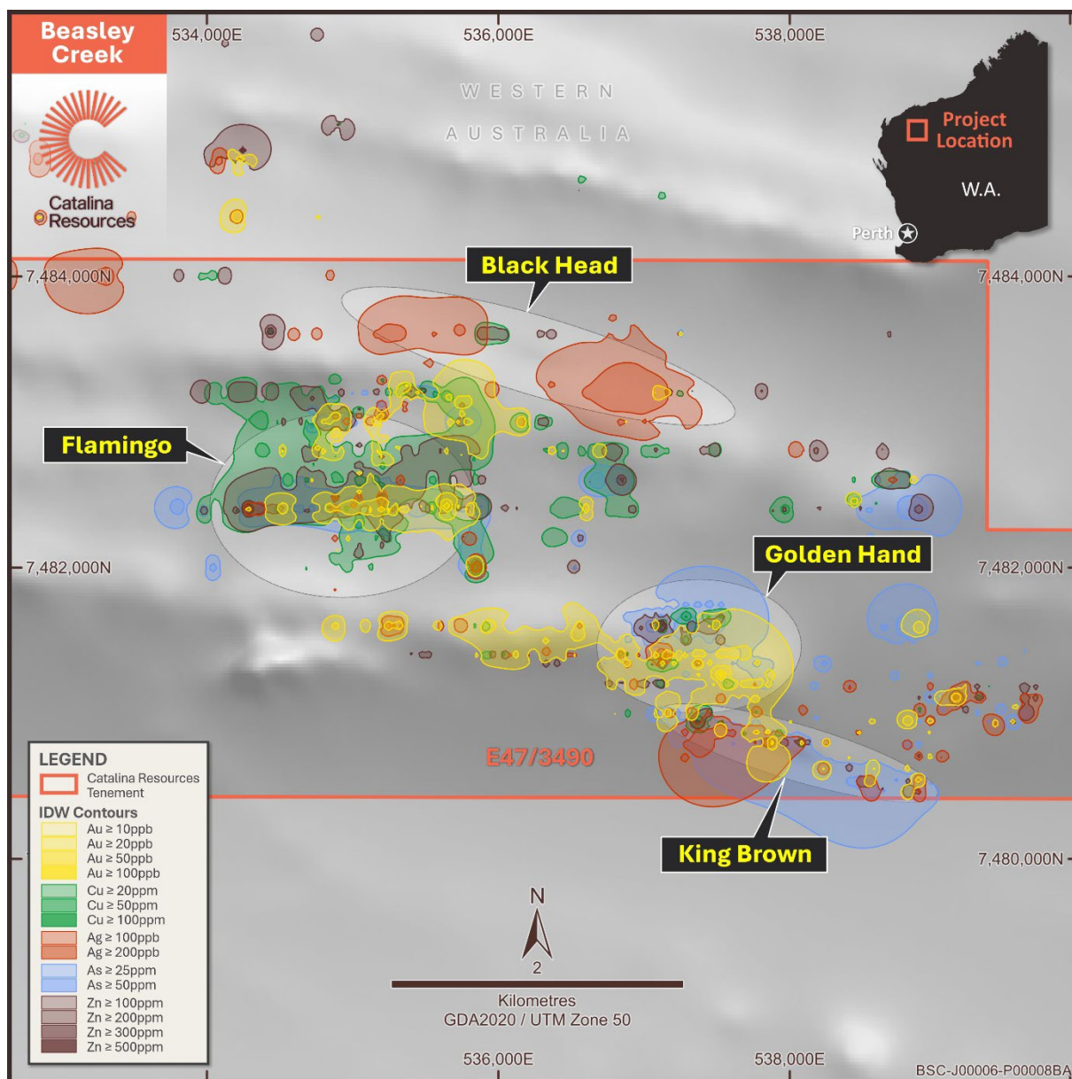
Figure 15: Interpreted soil geochemical contours highlighting the Flamingo, Golden Hand, King Brown and Black Head targets within EL 47/3490.
