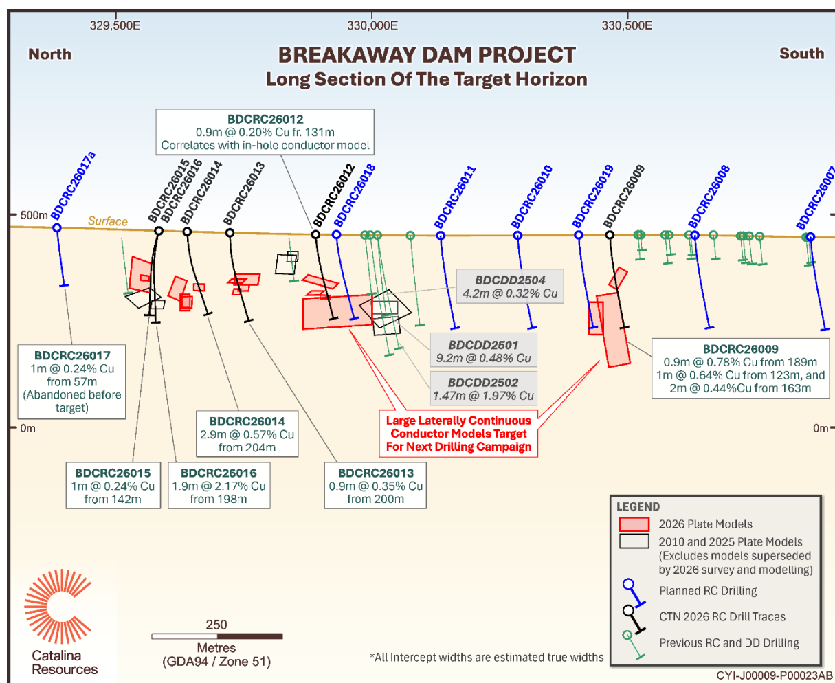
Figure 14: Long section of target horizon showing recently modelled DHEM plates and significant intercepts
