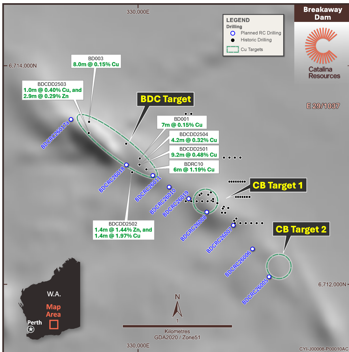
Figure 13: Plan view of BDC Central Zone target drill area including previous drill holes and associated results
