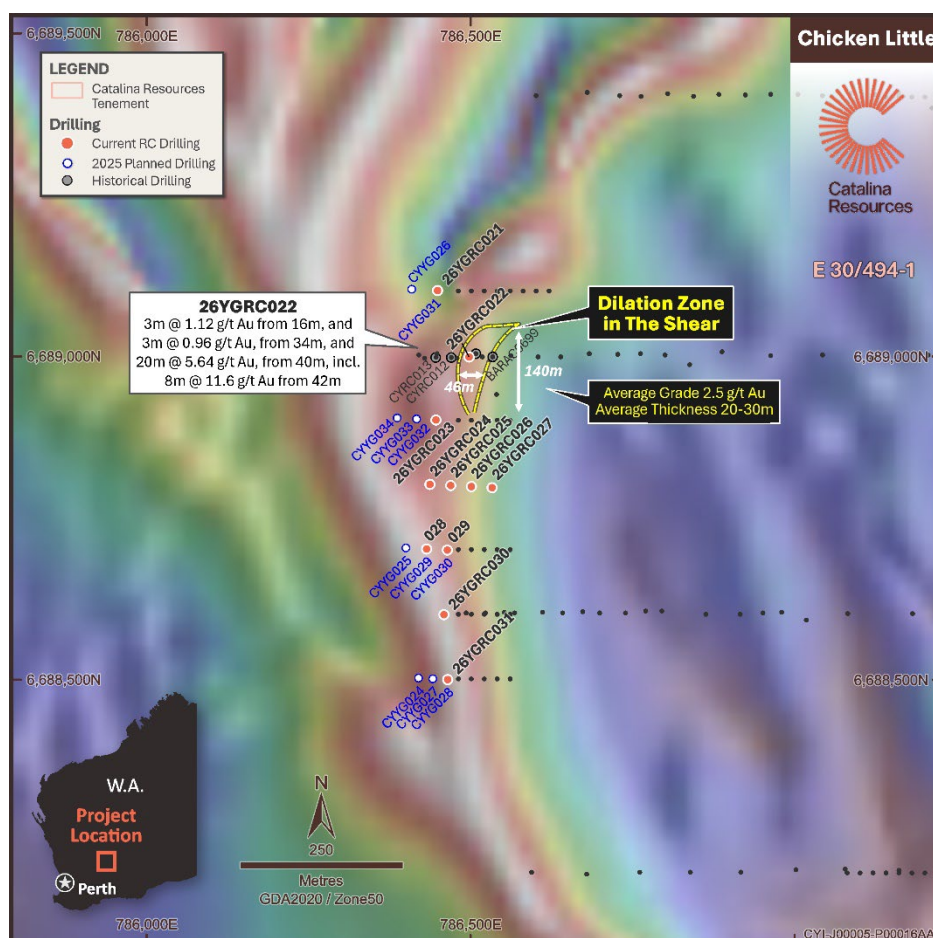
Figure 4: Chicken Little Priority target area where a potential dilation zone within the mineralised shear is interpreted to extend for up to 140 metres along strike
