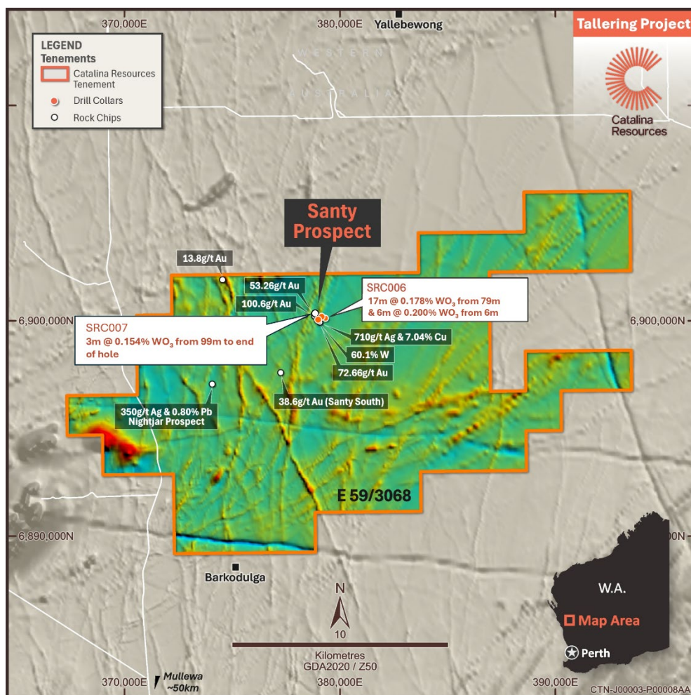
Figure 2: Plan view aeromagnetic image showing selected significant historical exploration results at Talling
