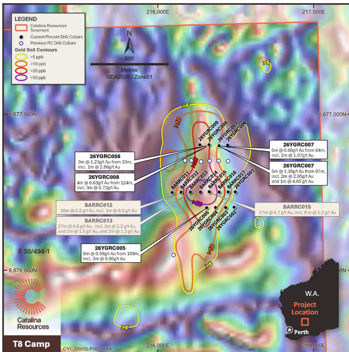
Figure 9. Plan view of T8 showing magnetic & soil contours, current and historic drill results
