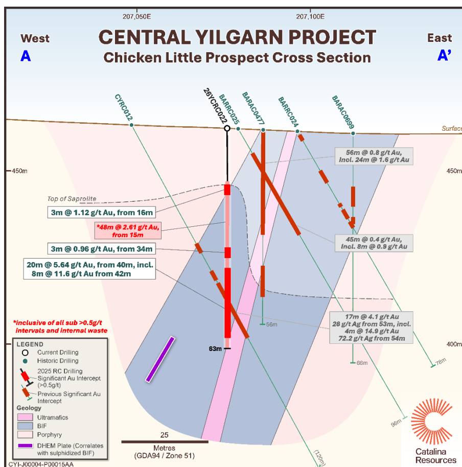
Figure 5: Cross-Section of reported intersections @ Chicken Little
