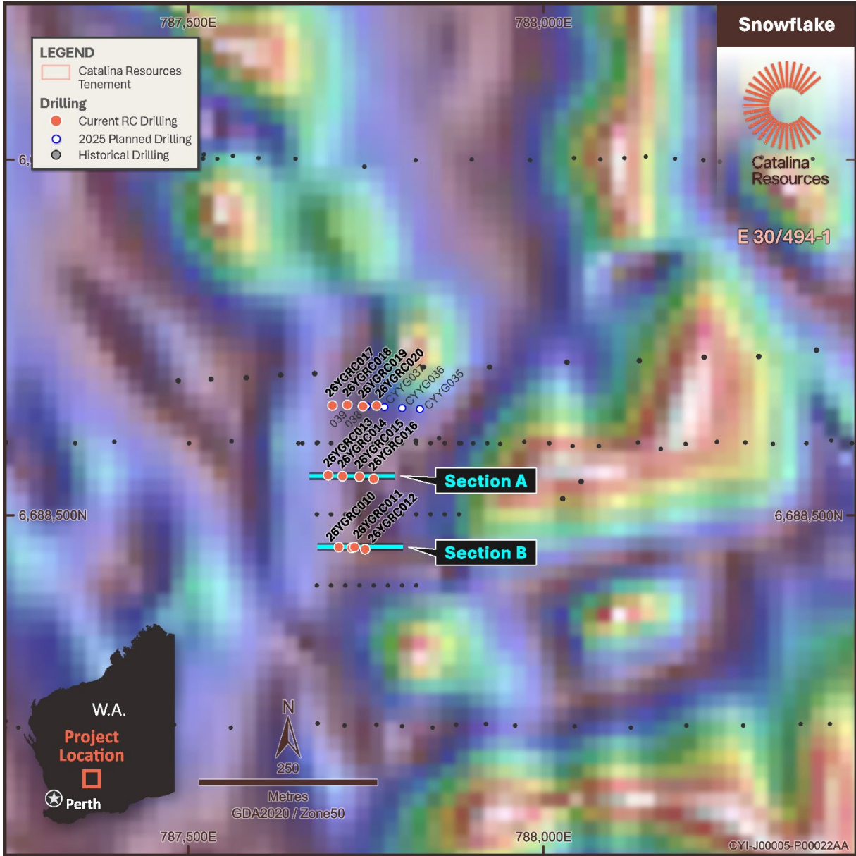
Figure 6: Current and historic drill hole locations at Snowflake
