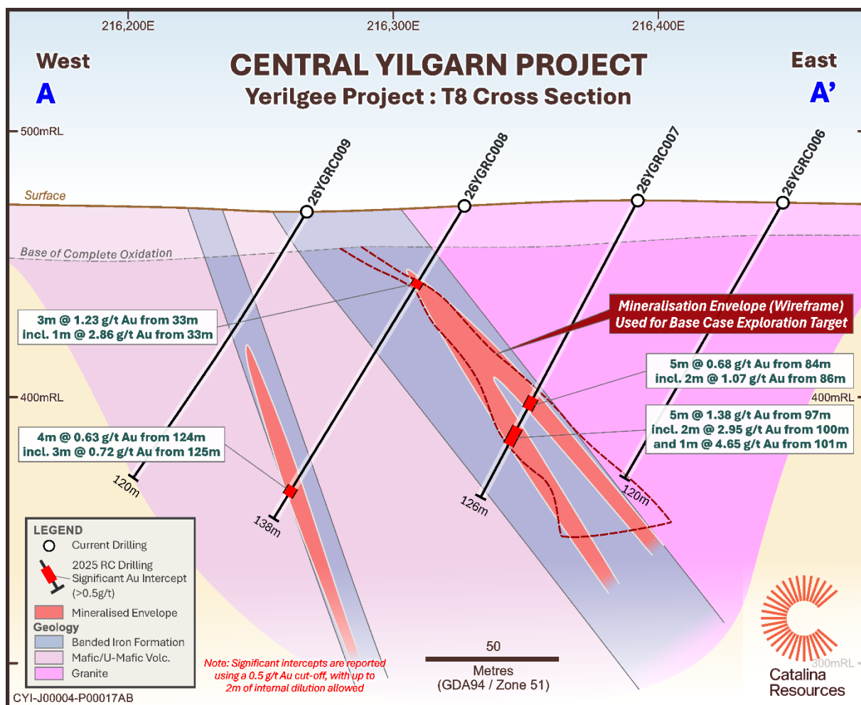
Figure 10: T8 reinterpretation of mineralisation envelopes used for base case Exploration Targets.
