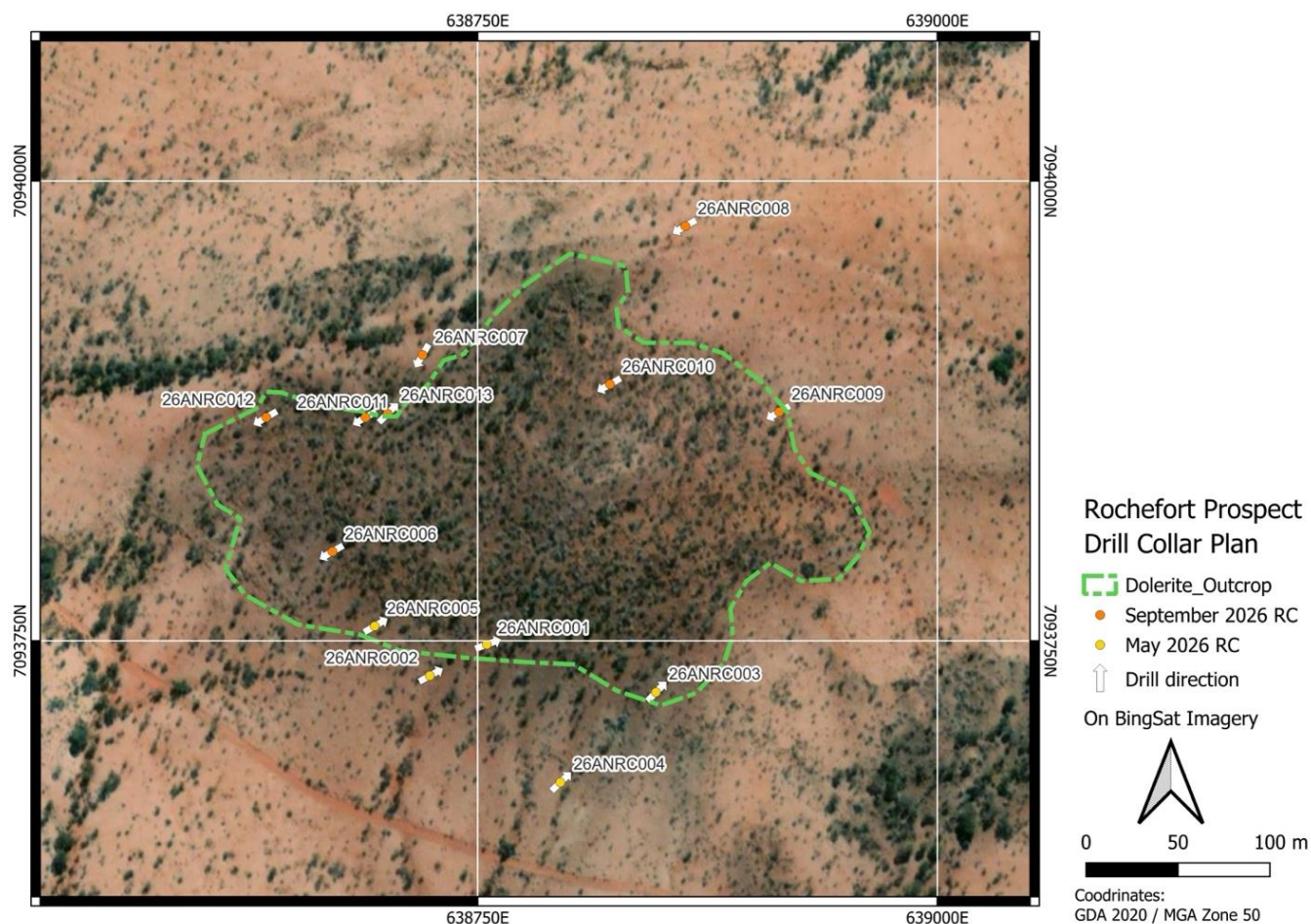
Figure 2: Rochefort drill hole plan showing maiden and current RC drilling over the interpreted fractionated dolerite.
