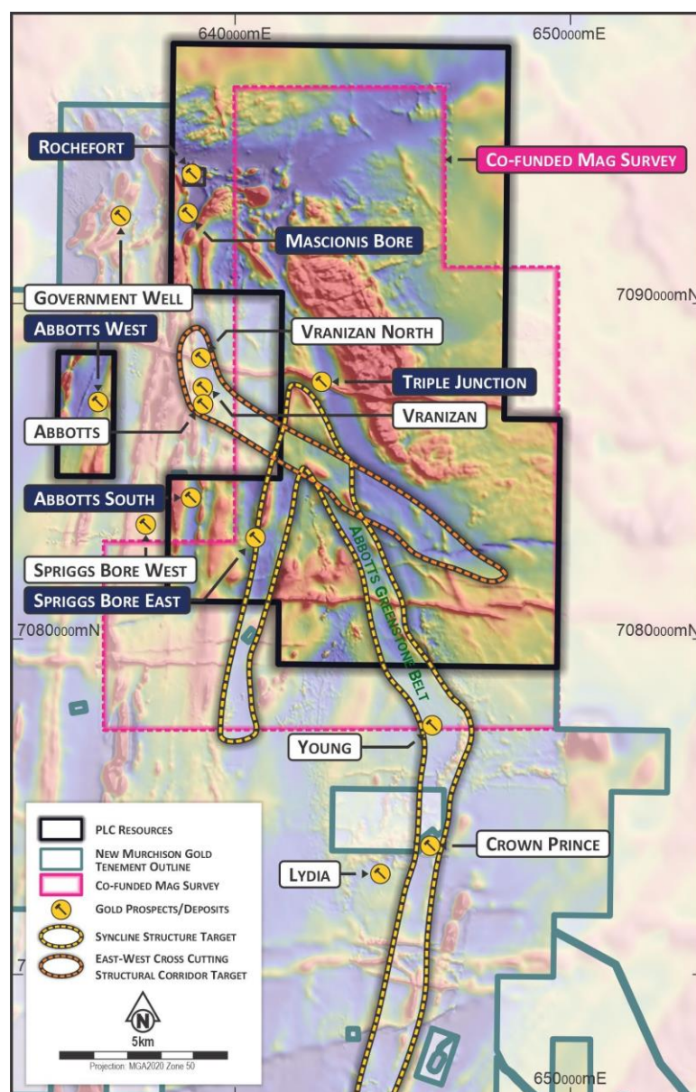
Figure 4: Abbotts North magnetic image showing the interpreted syncline and cross-cutting structural corridor targets.
