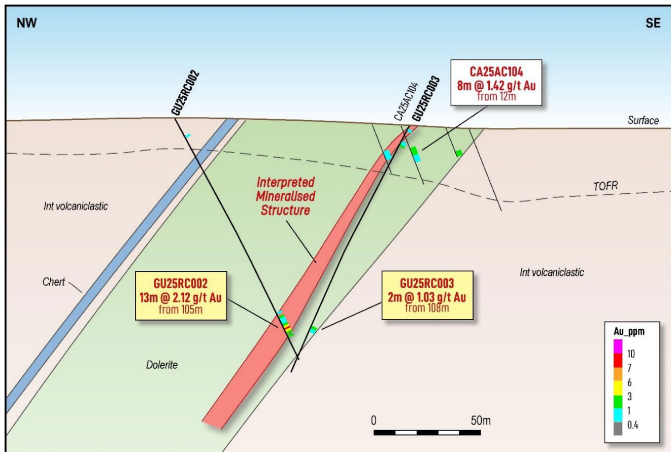
Figure 11: Cross-section on line A-A' looking north-east at Guppy, showing significant intercepts and 8m @ 1.42g/t in CA25AC104 from ASX Announcement 4th August 2025. Mineralisation is interpreted to dip ~50 degrees to the north-west striking north-east.
