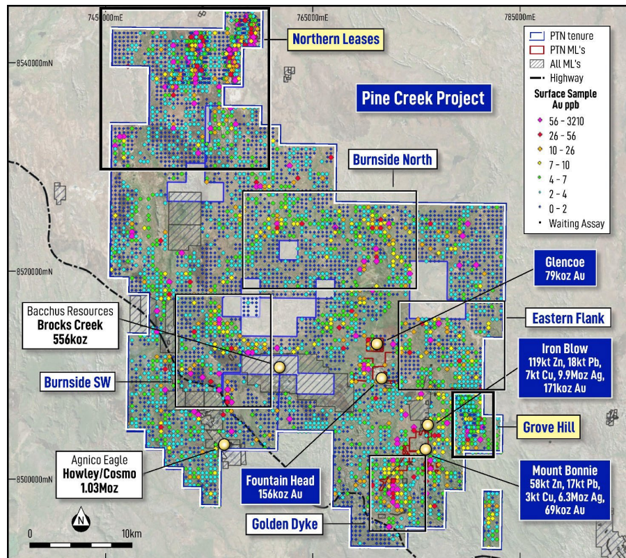
Figure 2: Priority RC drill target areas across the Pine Creek Project showing previously announced surface geochemical results (see ASX Announcement dated 27 February 2026). The 2026 RC drilling programme includes testing of targets within the Grove Hill, Golden Dyke, Burnside North and the Northern Leases project areas.
