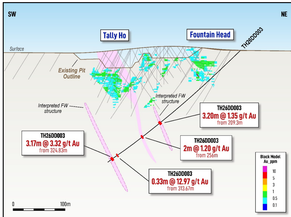
Figure 6: Cross-section through the Tally Ho – Fountain Head mineralised system at TH26DD003 showing reported gold intercepts, the existing Mineral Resource Estimate and historical pit outline.
