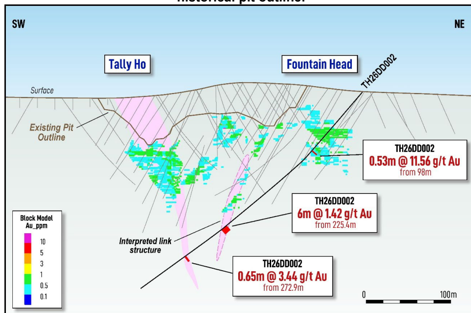
Figure 5: Cross-section through the Tally Ho – Fountain Head mineralised system at TH26DD002 showing reported gold intercepts, the existing Mineral Resource Estimate and historical pit outline.
