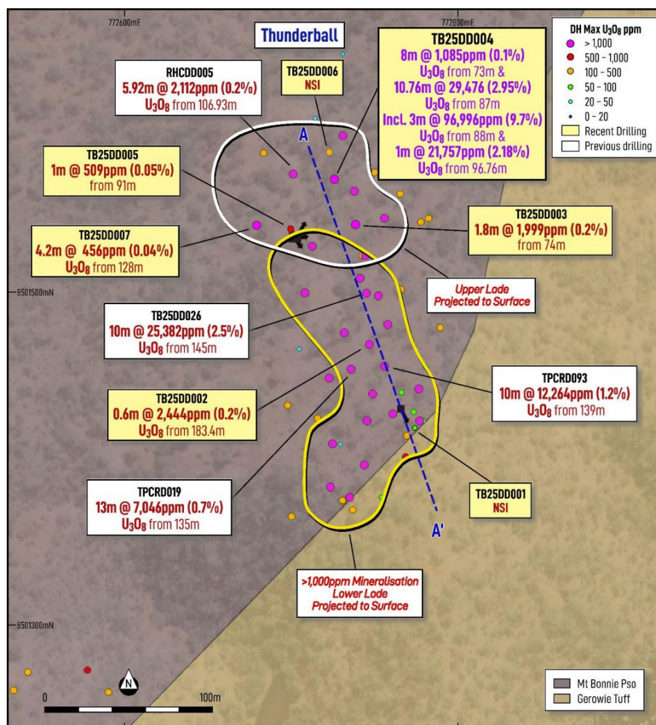
Figure 7: Plan view showing recent Thunderball holes with Max U 3 O 8 ppm (as mid points) over satellite and PTN regional geology. The >1,000ppm U 3 O 8 mineralisation is projected to surface as the yellow polygon and the upper lode as a white polygon.
