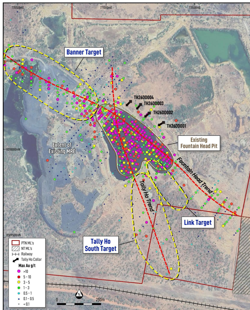
Figure 3: Plan view of the Fountain Head area showing recently completed diamond drill-holes. The Tally Ho and Fountain Head mineralised trends are shown as dashed red lines, with RC drill target areas outlined in yellow dashed lines.
