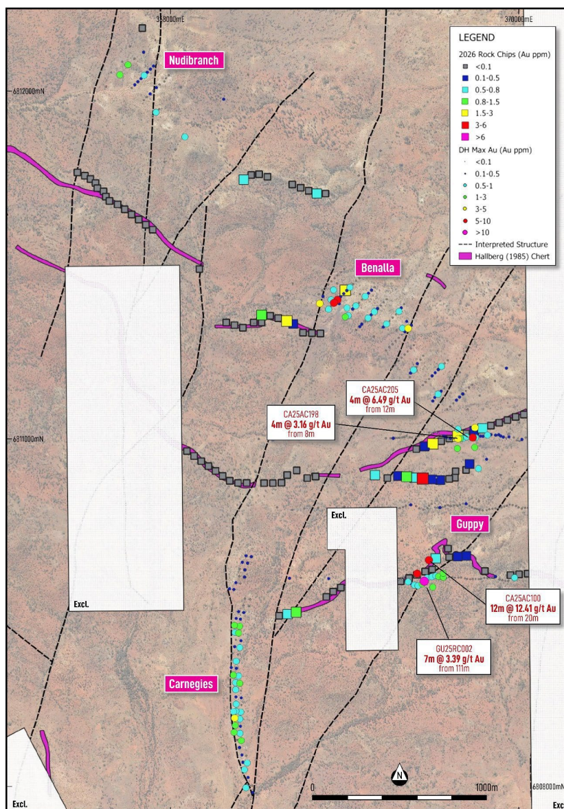
Figure 13: 2026 Guppy-Benalla rock chip results in Au ppm shown with Hallberg (1985) mapped chert, historical drill-hole maximum Au values, over satellite and interpreted structures.
