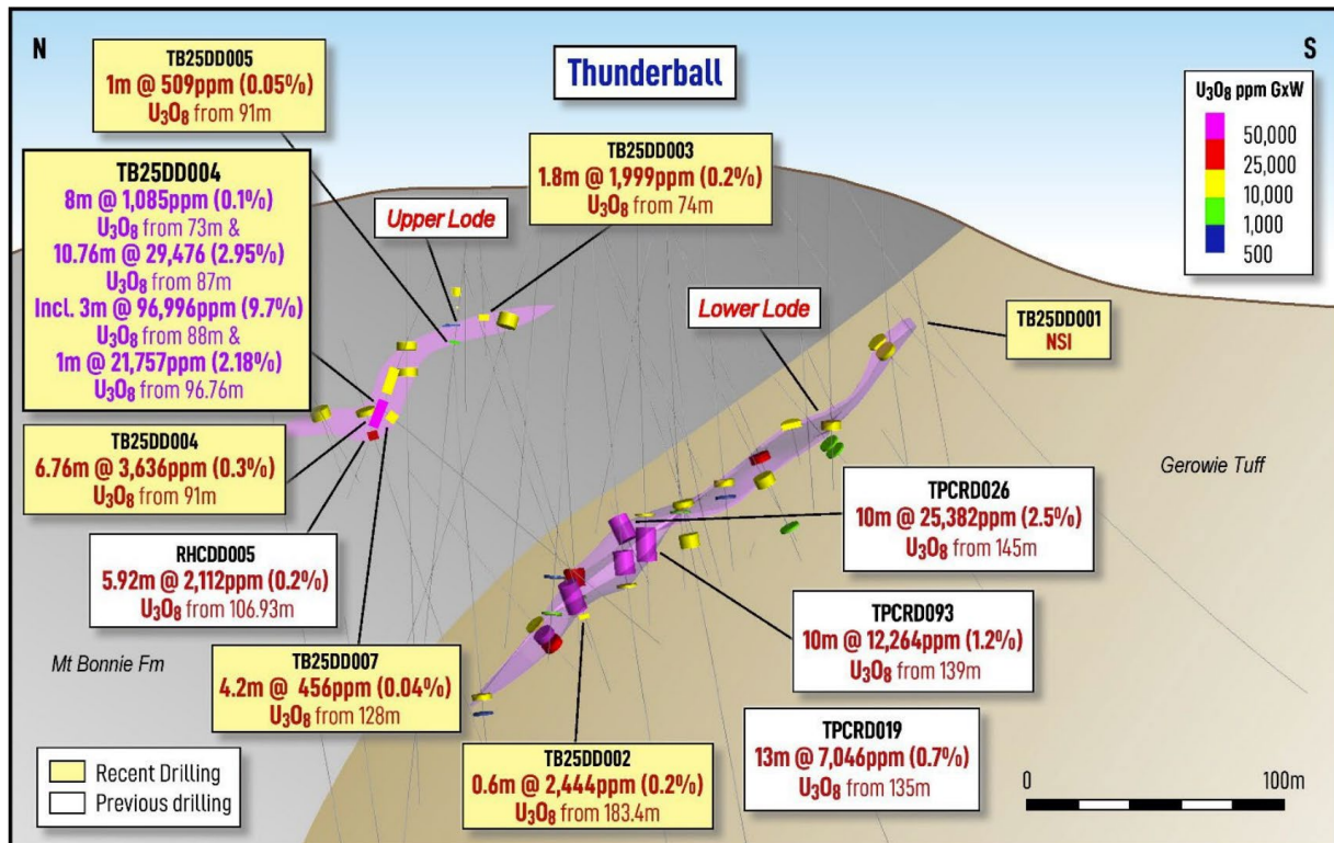
Figure 8: Long section A-A', clipped to 40m, looking East at Thunderball. Mineralisation envelope can be seen in pink, with intercepts from this program shown as yellow text boxes and historic as white text boxes. The lower lode sits in the Gerowie Tuff just below the contact with the Mt Bonnie Formation whilst the upper lode is within a more tuffaceous unit of the Mt Bonnie formation.
