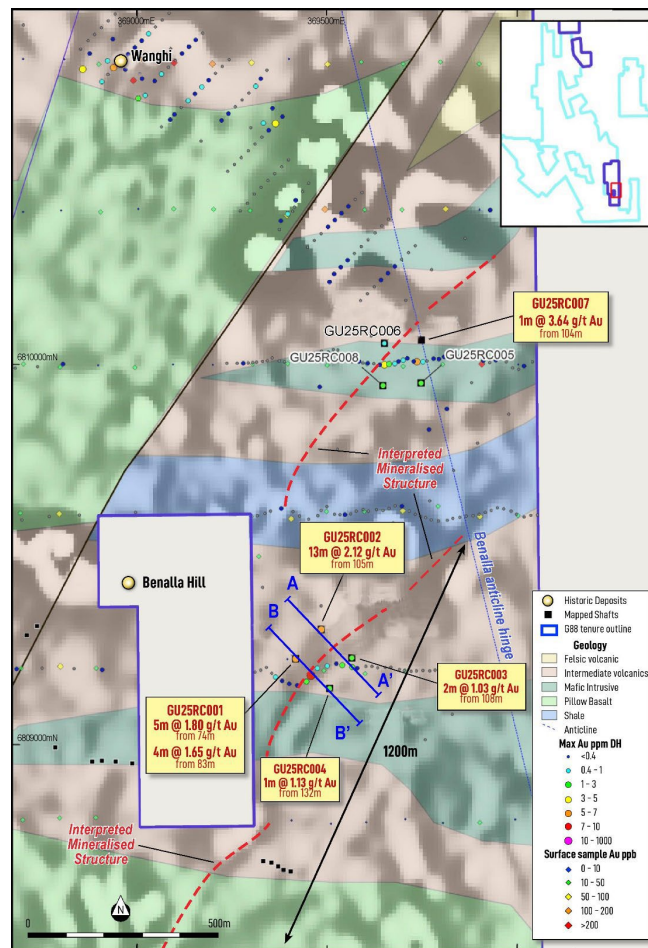
Figure 10: Guppy RC holes showing Max Au and interpreted north-east striking mineralised shears. Lithologies dip to the north-northwest reflecting the position near the nose of the Benalla anticline.
