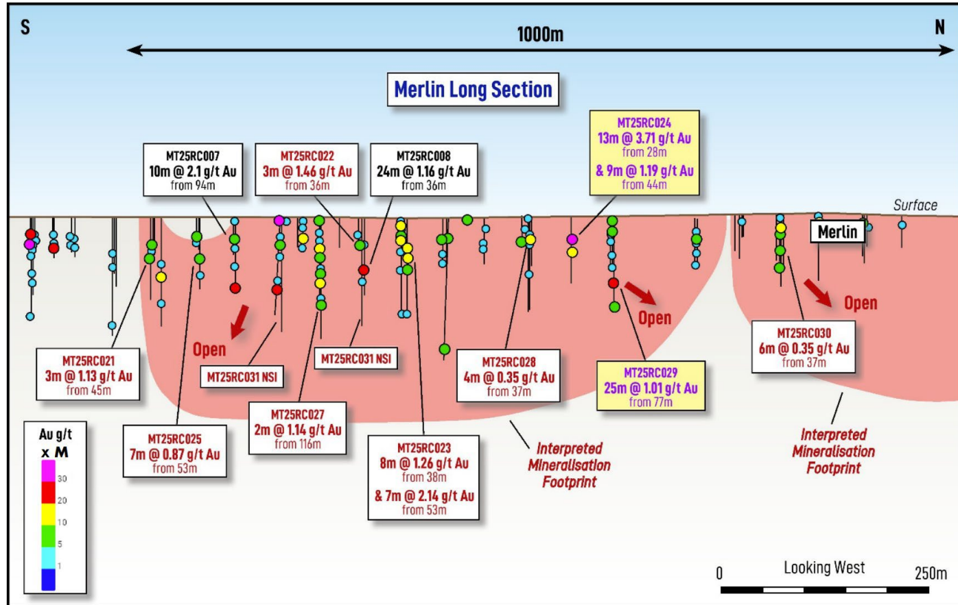
Figure 14: Long section looking west at Merlin, showing recent drill results in red as gram m points and the interpreted mineralisation footprint. Standout intercepts are coloured purple and previously reported intercepts are black (see ASX announcement 21 June 2025).
