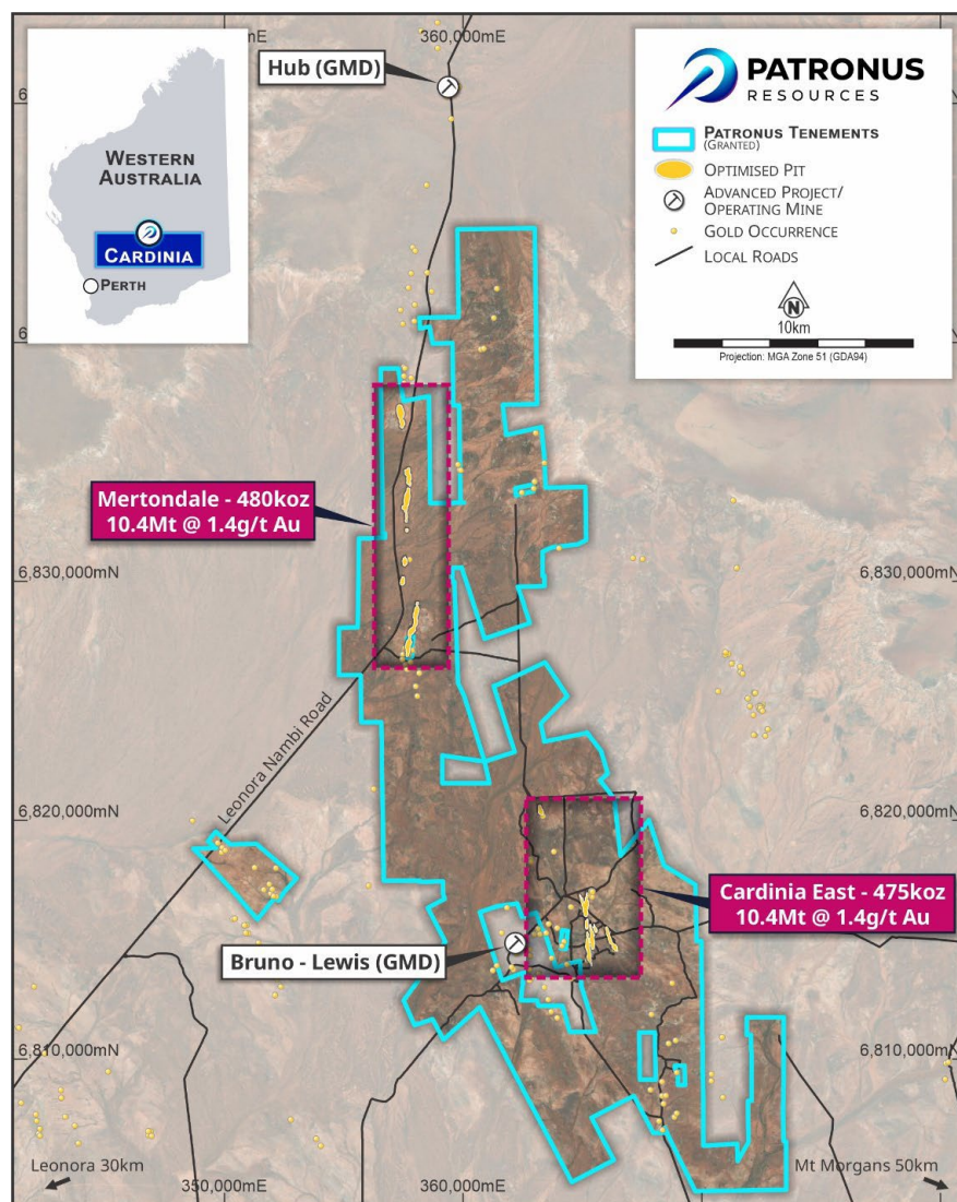
Figure 9: Overview of Patronus' Cardinia tenure showing current Resources Guppy Prospect
