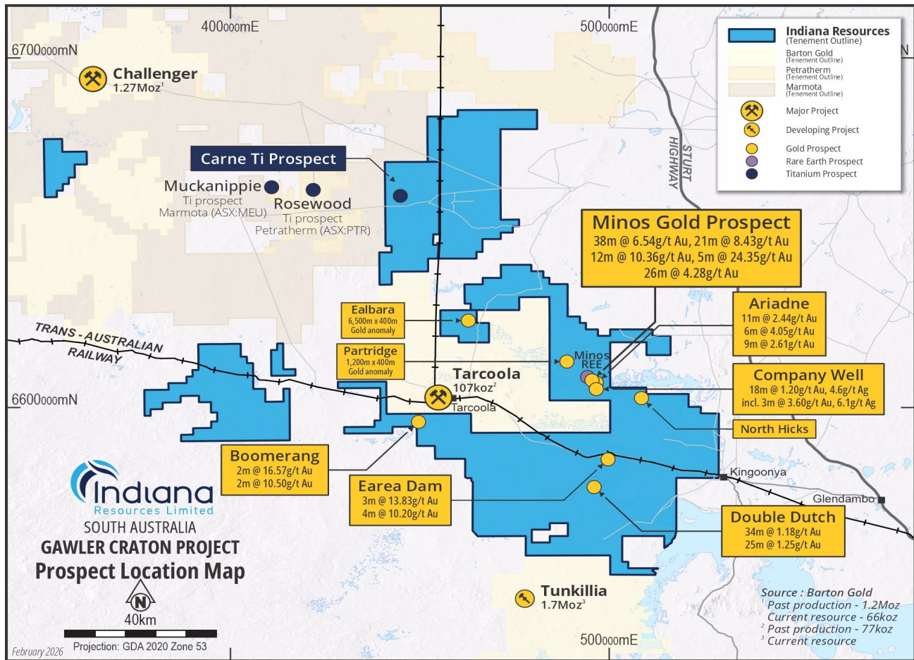
Figure 1: Gawler Craton Project Location Map
