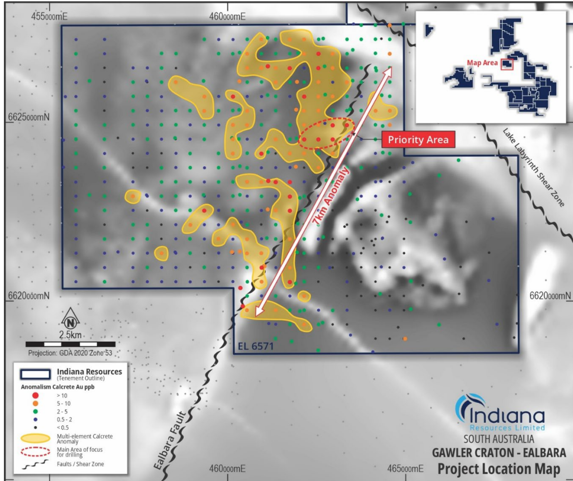
Figure 6: Plan showing surface calcrete samples with Au ppb values (dots) vs the interpreted multi-element calcrete anomaly over TMIRTP magnetics. The anomaly is proximal to the Ealbara Fault and bounded by the LLSZ.
