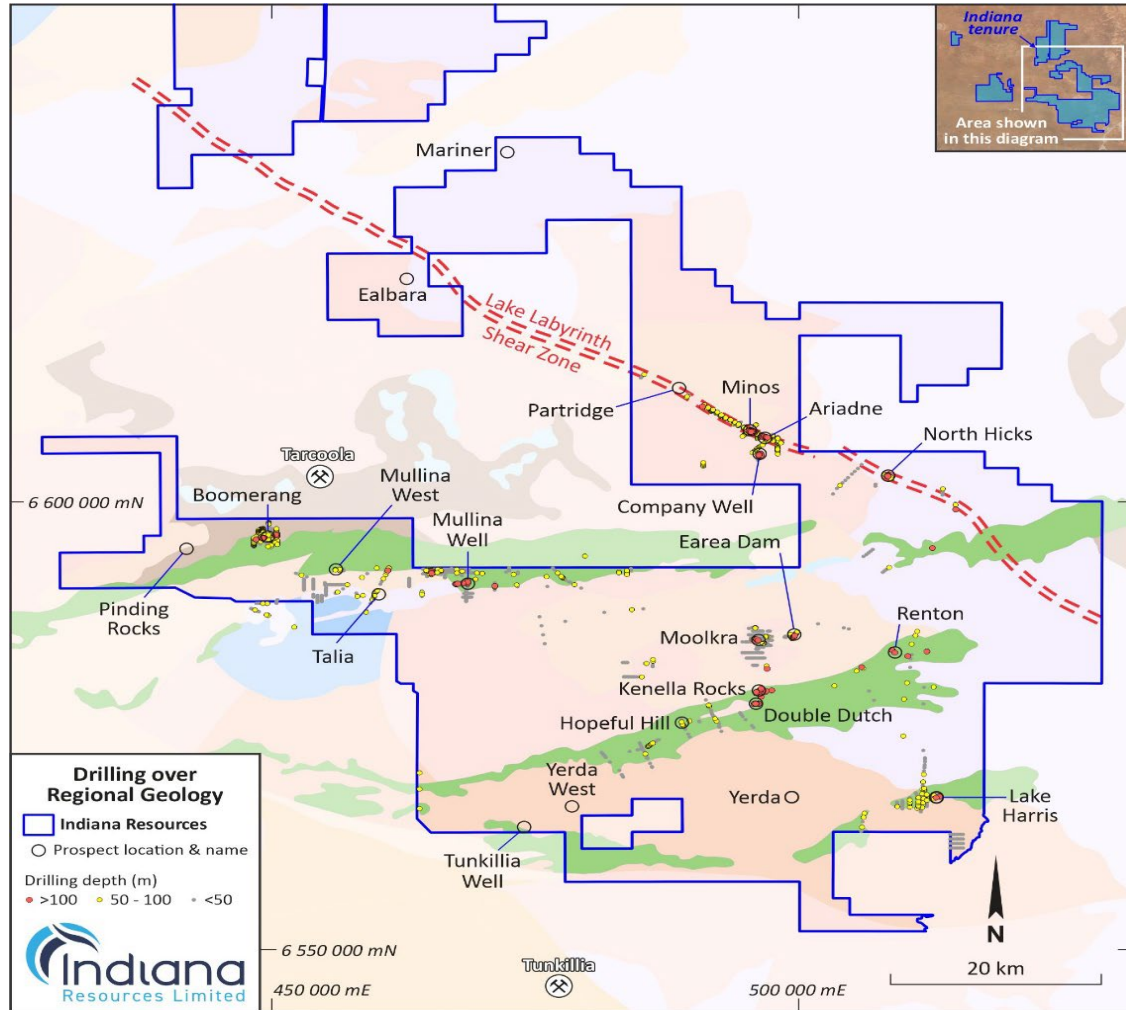
Figure 2: Location map highlighting gold prospects within the Gawler Craton Project area.
