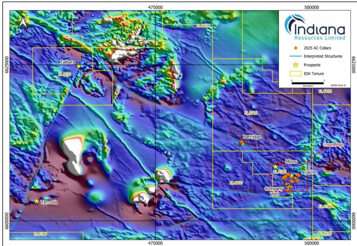
Figure 8: Regional Map (TMI image) showing the key regional structures, notably the major Lake Labyrinth Shear Zone.
