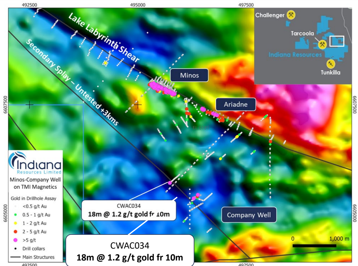
Figure 4: Plan showing CWAC034 and max gold in drill hole assay, over TMI Magnetics, major controlling Lake Labyrinth Shear and Secondary Splay within the Minos-Ariadne-Company Well area of the Minos Gold Project.
