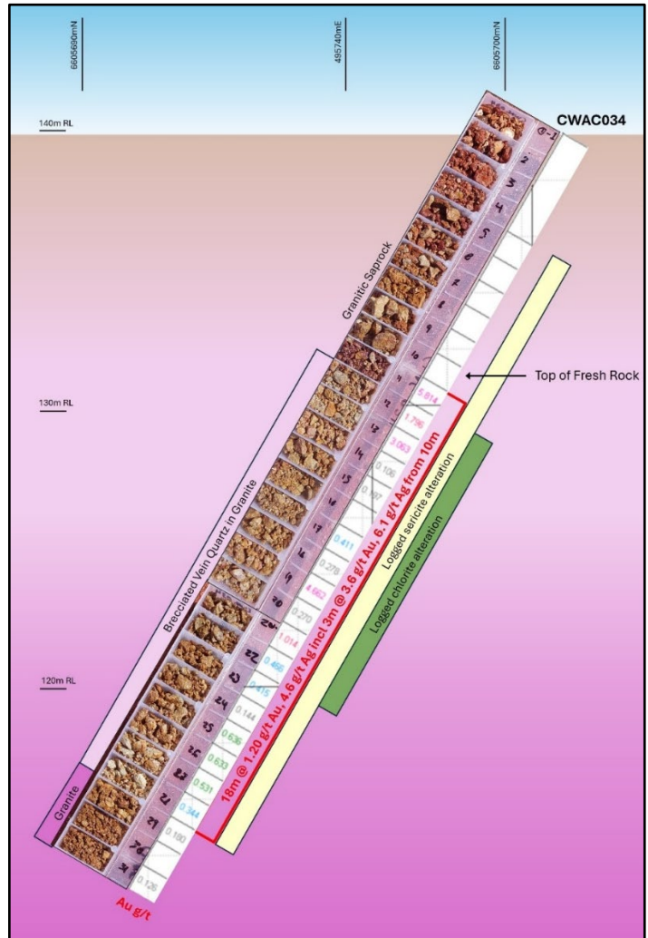
Figure 5: Section of CWAC034 showing the extent of sericite and chlorite alteration with gold.
