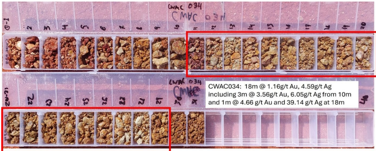
Figure 3: AC chip tray of CWAC034 highlighting the 18m mineralised zone.
