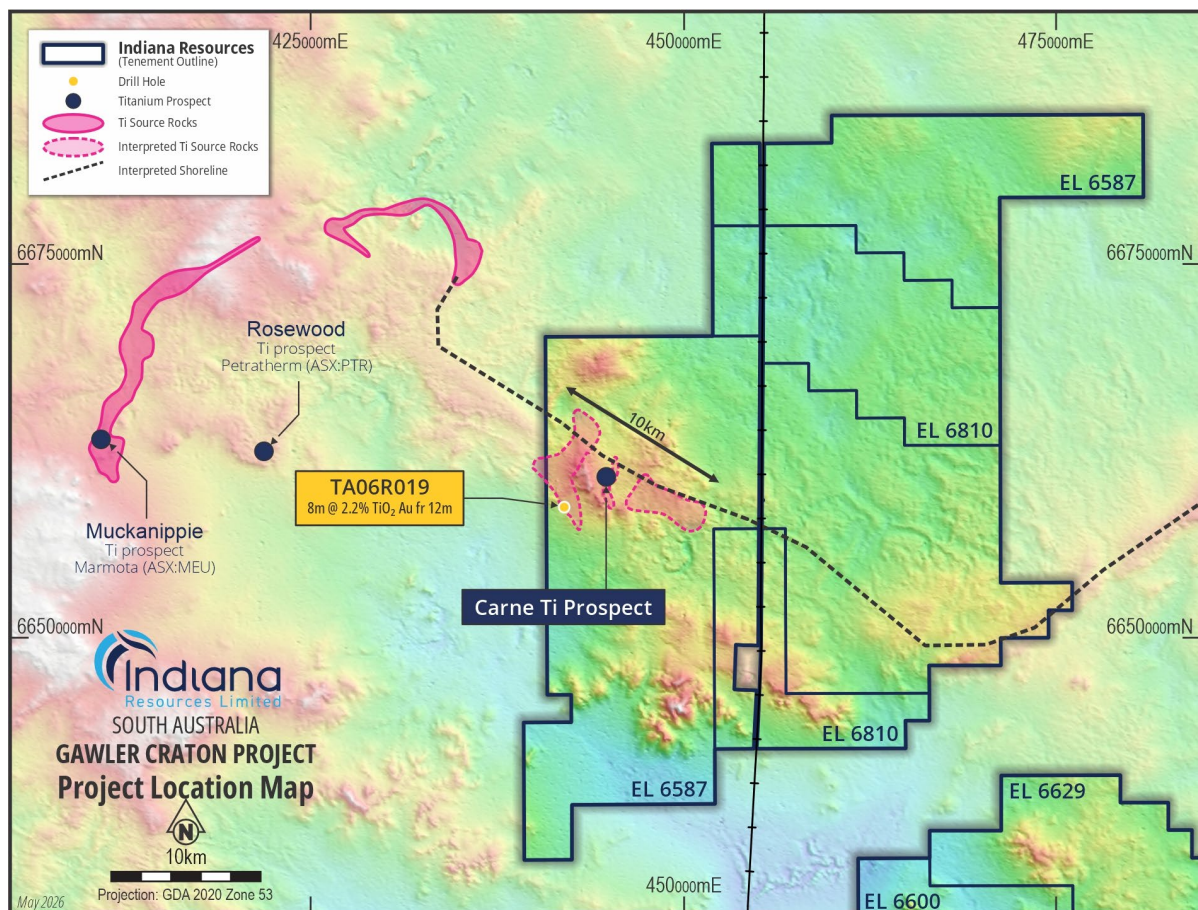
Figure 9: Interpreted Paleo Shoreline over digital terrain model and HM prospects.
