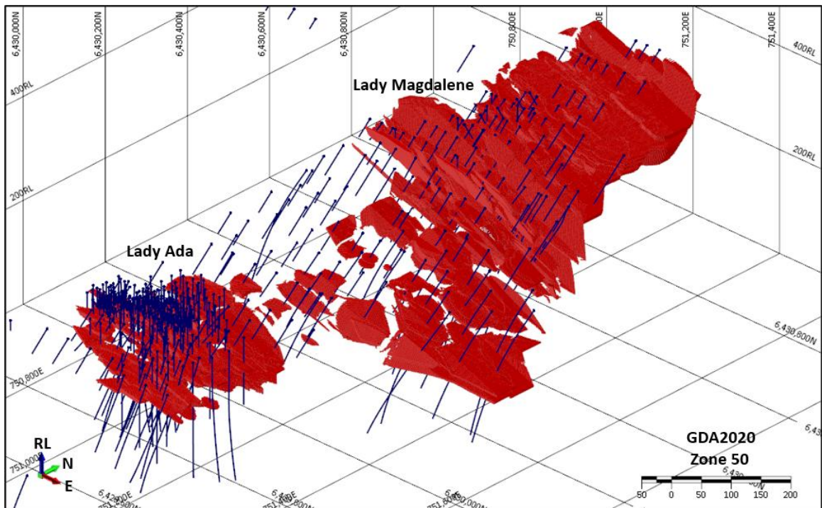
Figure 4: Perspective View of Indicator Model Wireframes and Drilling Data
