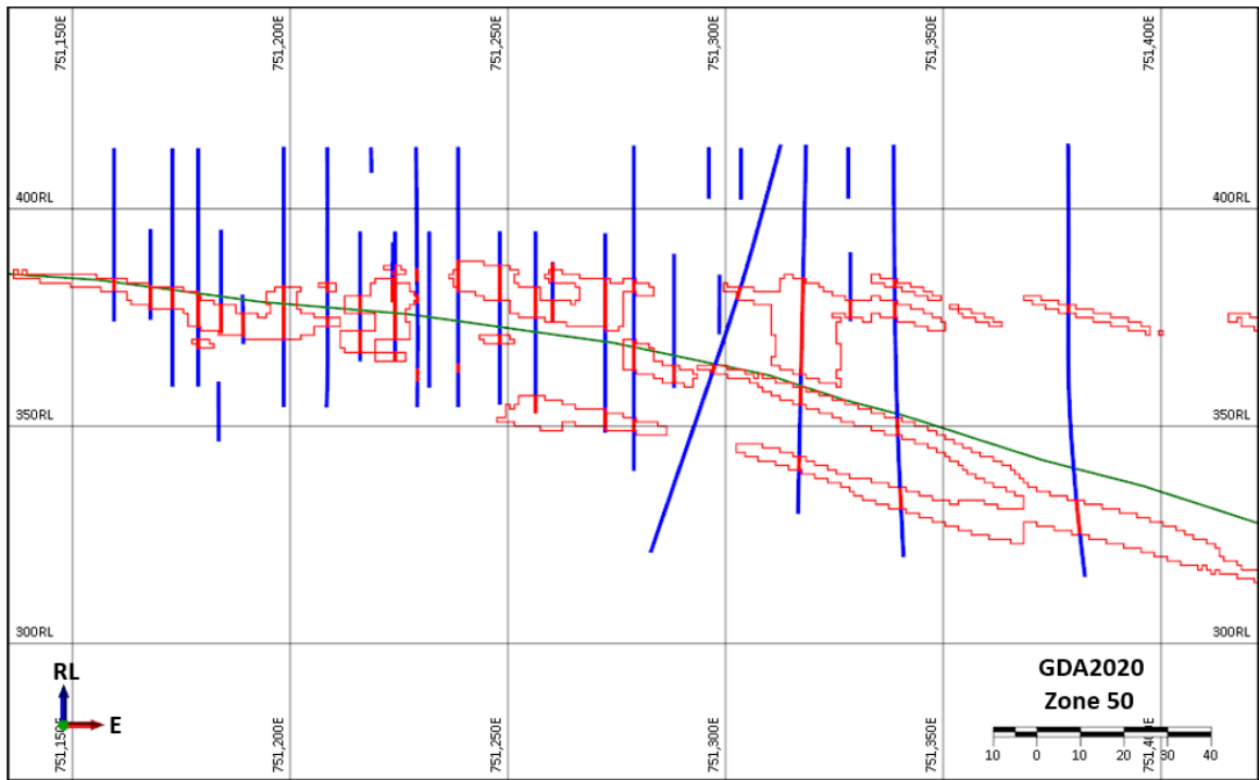
Figure 3: Cross Section of Mineralisation Intersections, Drilling Data and Unfolding Plane
