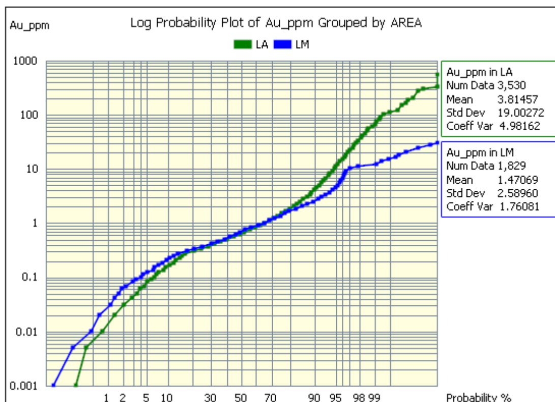
Figure 8: Au Log Probability Plot
