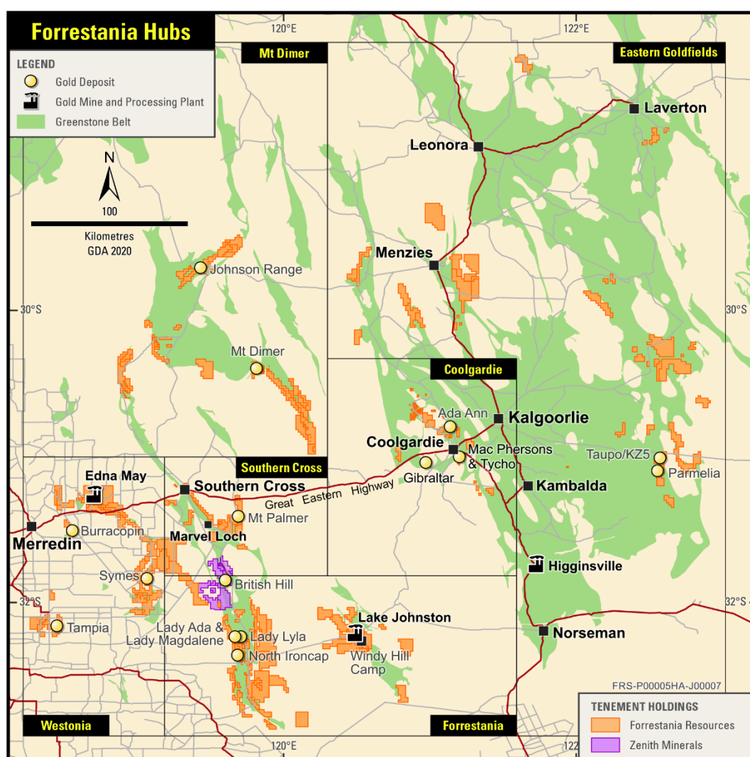
Figure 14: Forrestania Regional Hub locations
