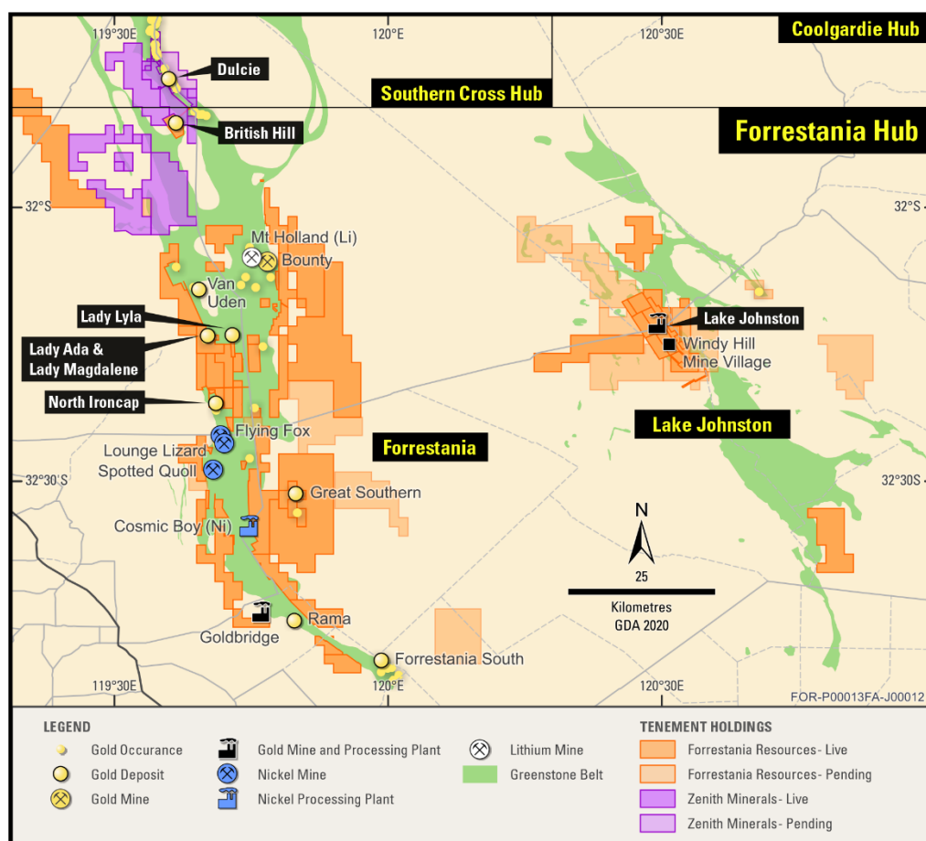
Figure 2: Forrestania Hub location
