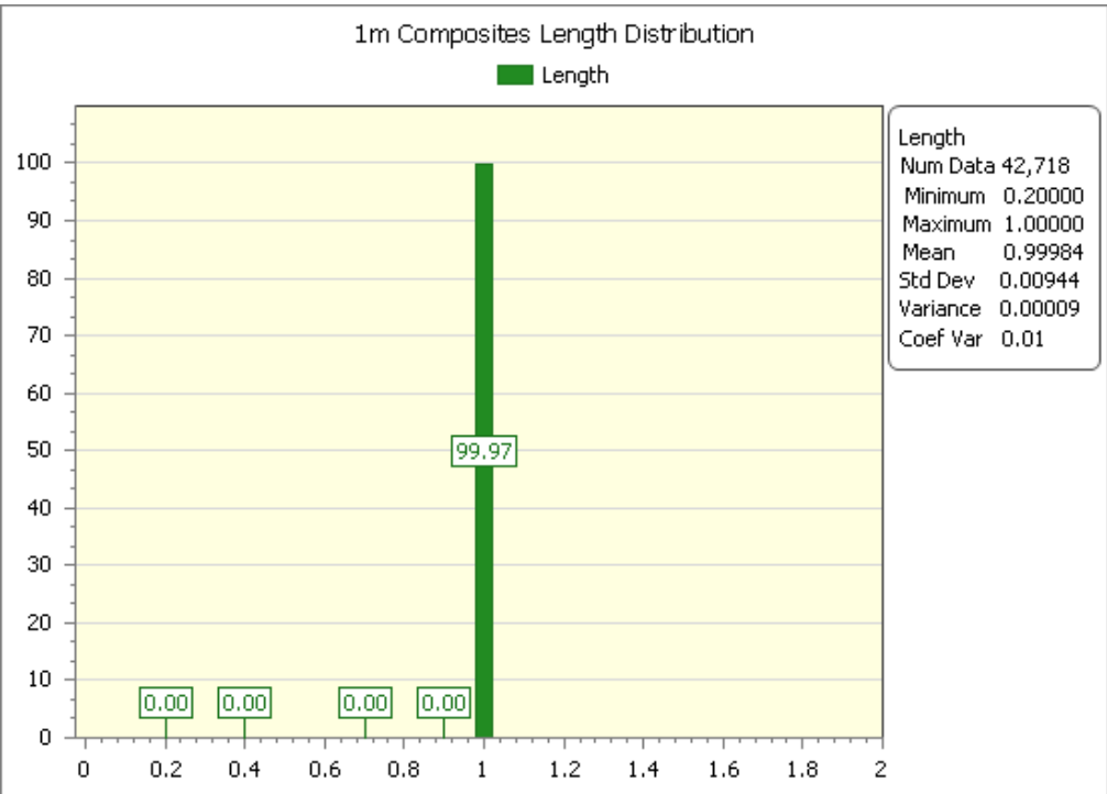
Figure 7: One Metre Composite Length Distribution
