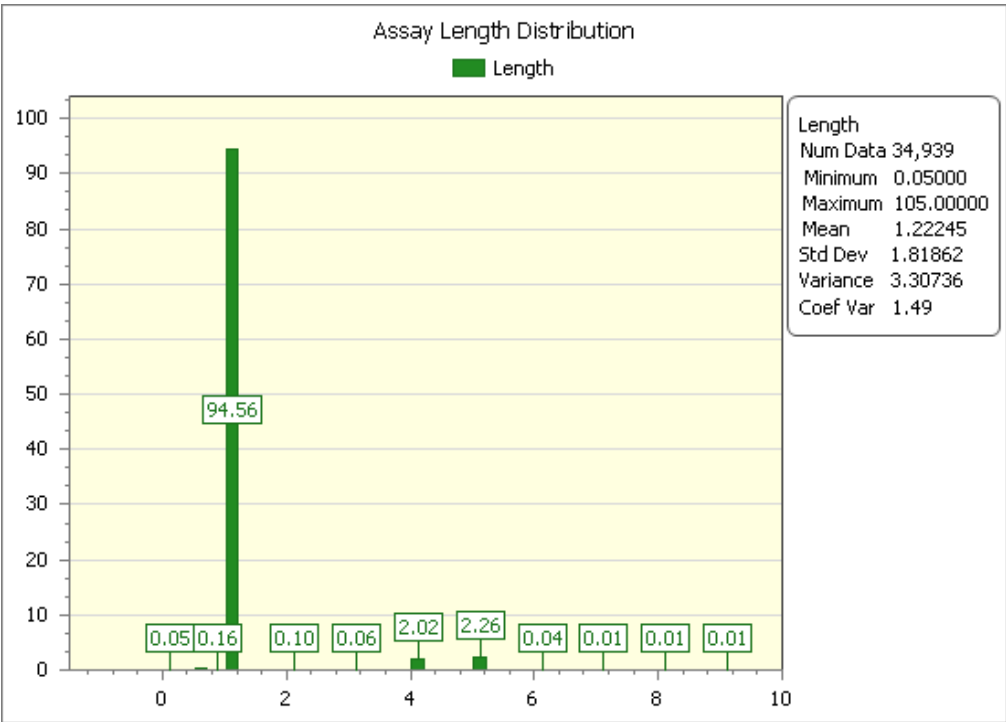
Figure 6: Assay Sample Length Distribution
