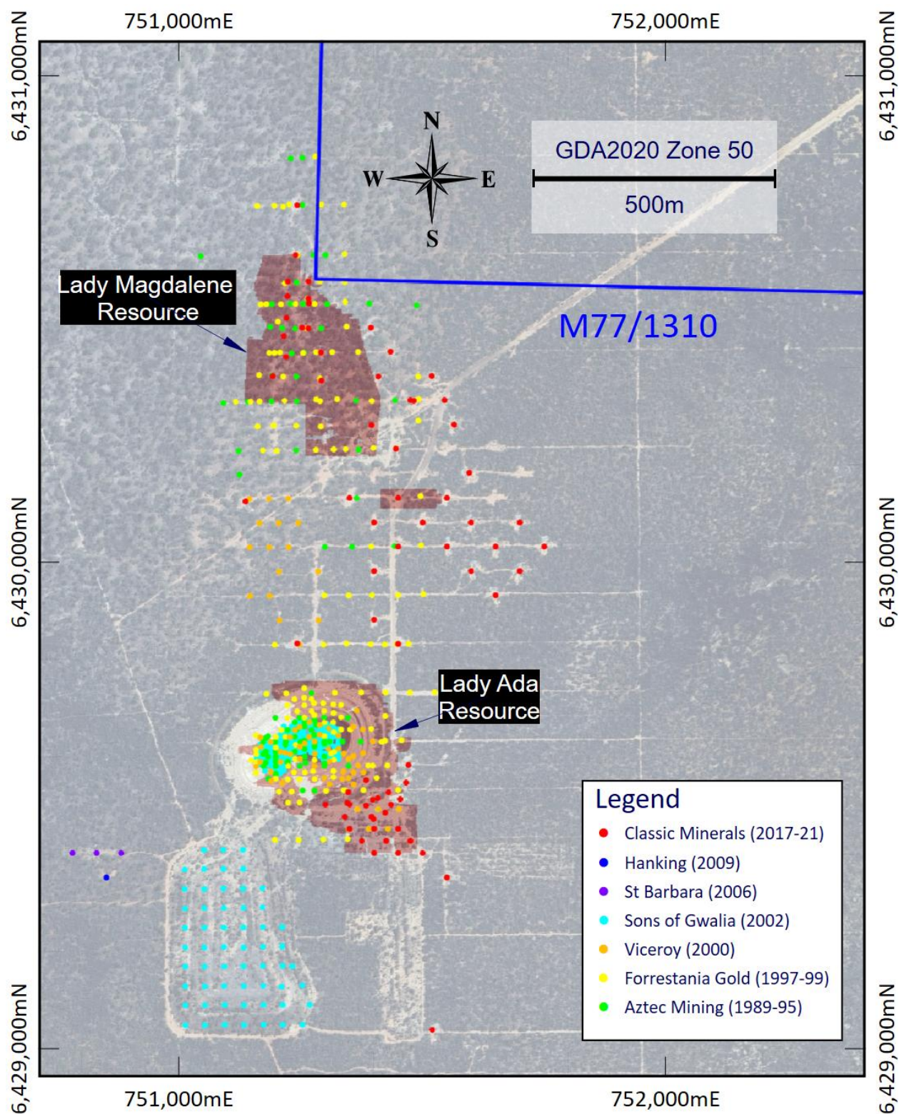
Figure 5: Ladies Drill Holes by Company and September 2026 Resource Outline
