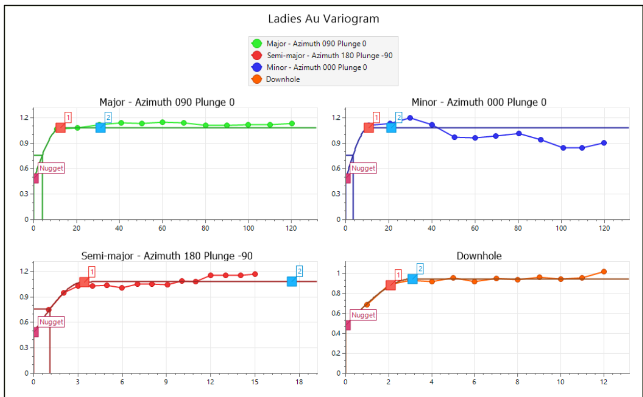
Figure 9: Variogram Models
