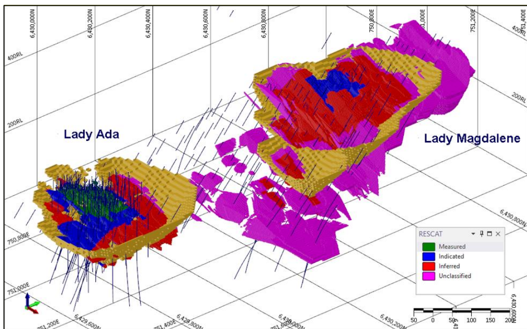
Figure 11: Ladies Deposits with AUD 6,000 Optimal Pit Shell
