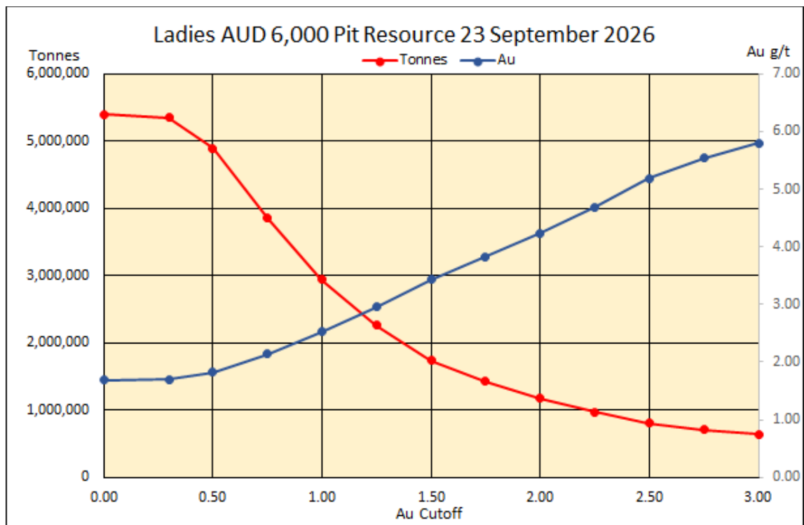
Figure 13: Optimal Grade Tonnage Curve for the Ladies (Measured + Indicated + Inferred)
