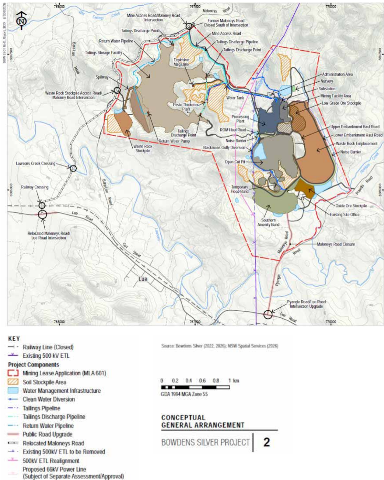
Figure 5. Bowdens Silver Mine Site Layout
