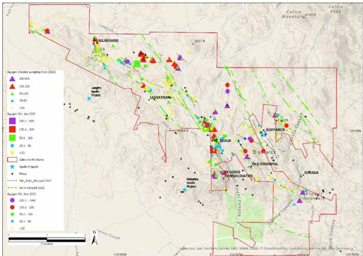
Figure 12. Calico North project, silver assay results, showing mapped veins and results of rock chip sampling. Note the number of clusters with good silver grades that will be followed up by drilling. It is possible that these clusters, are controlled by intersecting vein systems and stratigraphy.
