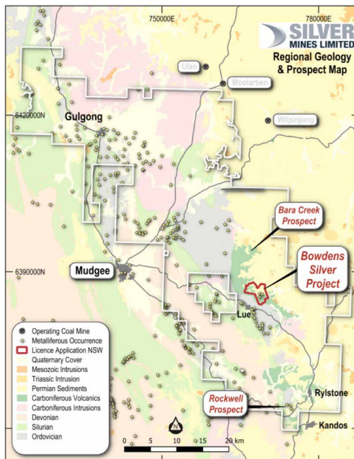
Figure 9. Bowdens Silver Project with prospects and geology.
