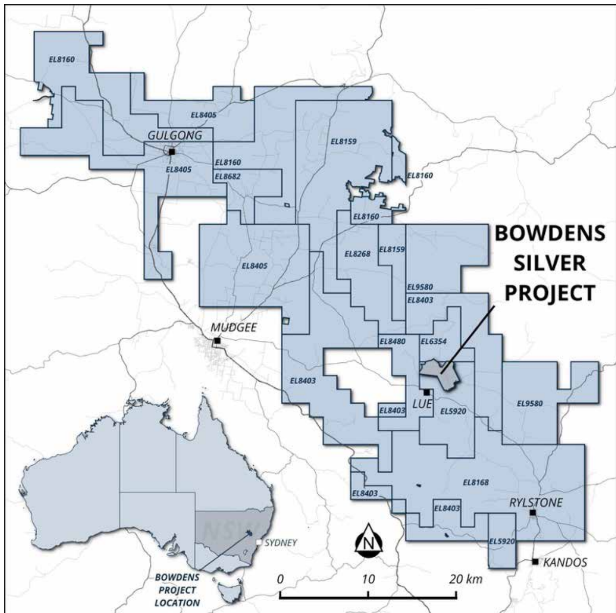
Figure 3. The Group's Exploration tenure and Bowdens Silver Project, Mining Lease Application near Mudgee.
