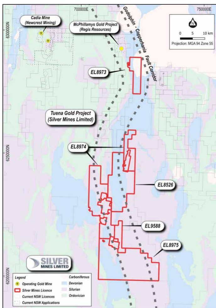
Figure 11: Map showing the Tuena Project
