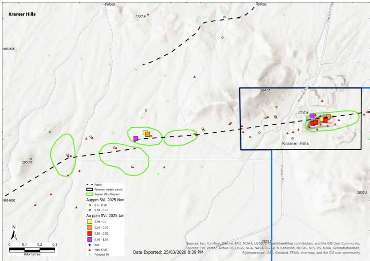
Figure 15. Zoomed view of the oxide prospect area. Note alignment with a mapped fault zone and presence of mine shafts that are spread along the zone, which were all worked prior to 1942. Silver Mines verification samples taken in 2025, confirm presence of mineralised system.
