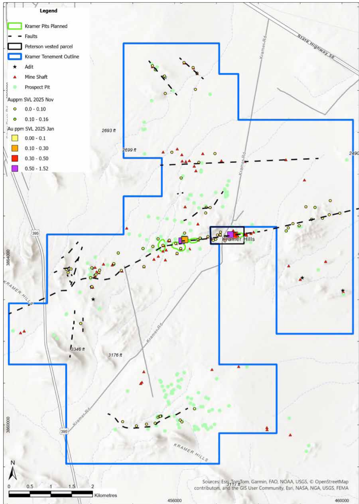
Figure 14. Kramer Hills Claim Map with Historic Workings and Faults. Note the exploration potential for areas outside of pits permitted for mining in the 1980's. A mapped and inferred fault running through the prospect area extends for over 7 km, aligned with pre-1942 mine shafts. There are also various repeated faults and lines of historical shafts that are prospective.
