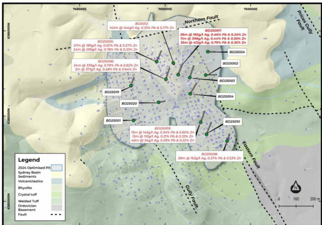
Figure 8: Drill hole locations and significant intercepts and 2024 Optimised Pit design.
