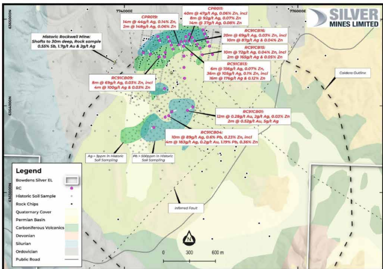
Figure 10. Rockwell prospect historic drilling, geology and soil anomalism. Soil anomalies shown by light green (Ag>3ppm) and light blue (Pb>500ppm) shapes. Rock chip sample locations shown as Black dots.
