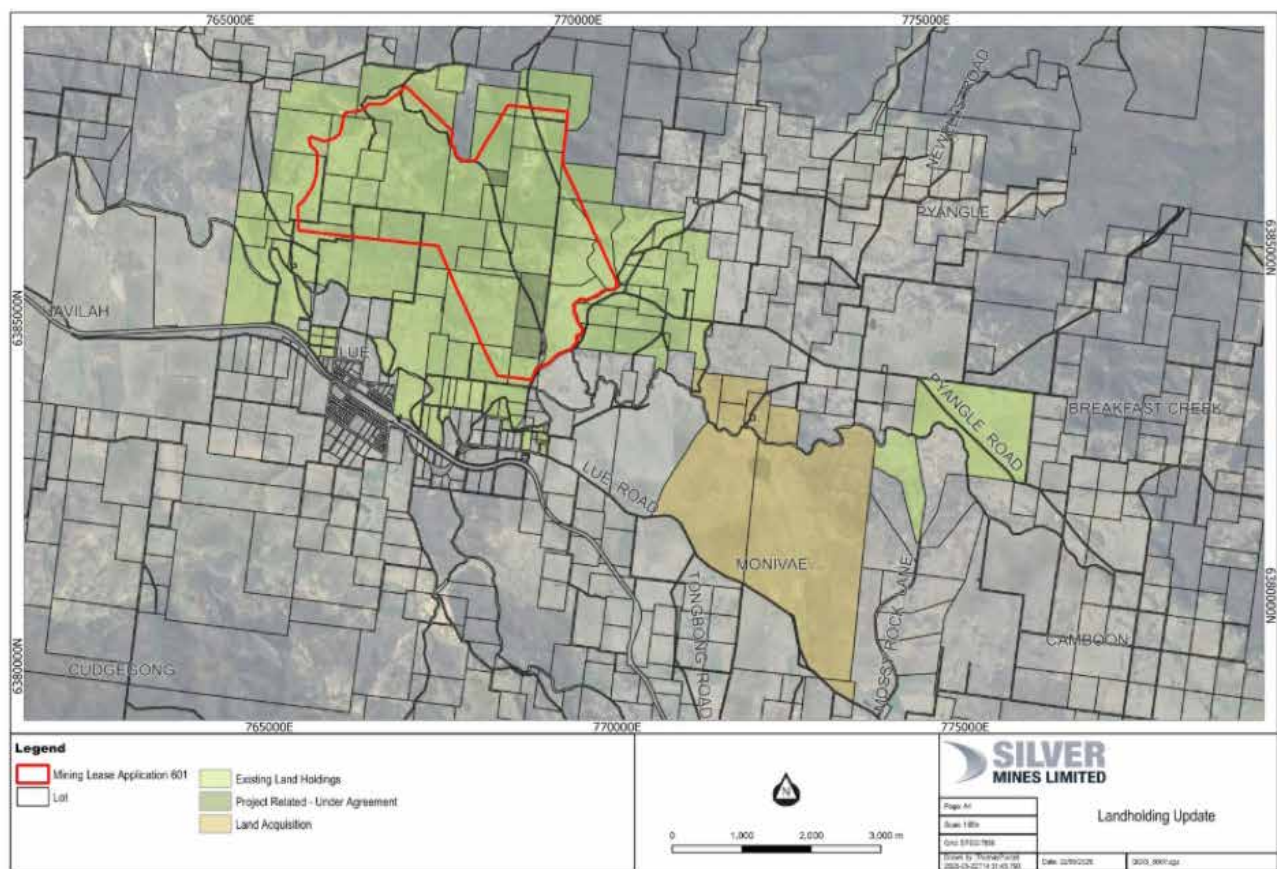
Figure 7. Satellite image overlain with property lots, the Bowdens Mining Licence Application and Bowdens Silver freehold land package.
