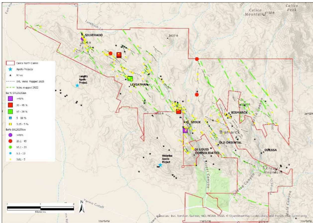
Figure 13. Calico North project, barite assay results. Note samples from Leviathan Barite Mine returned results of 10-20%, while other targets show results of greater than 20% Barite.
