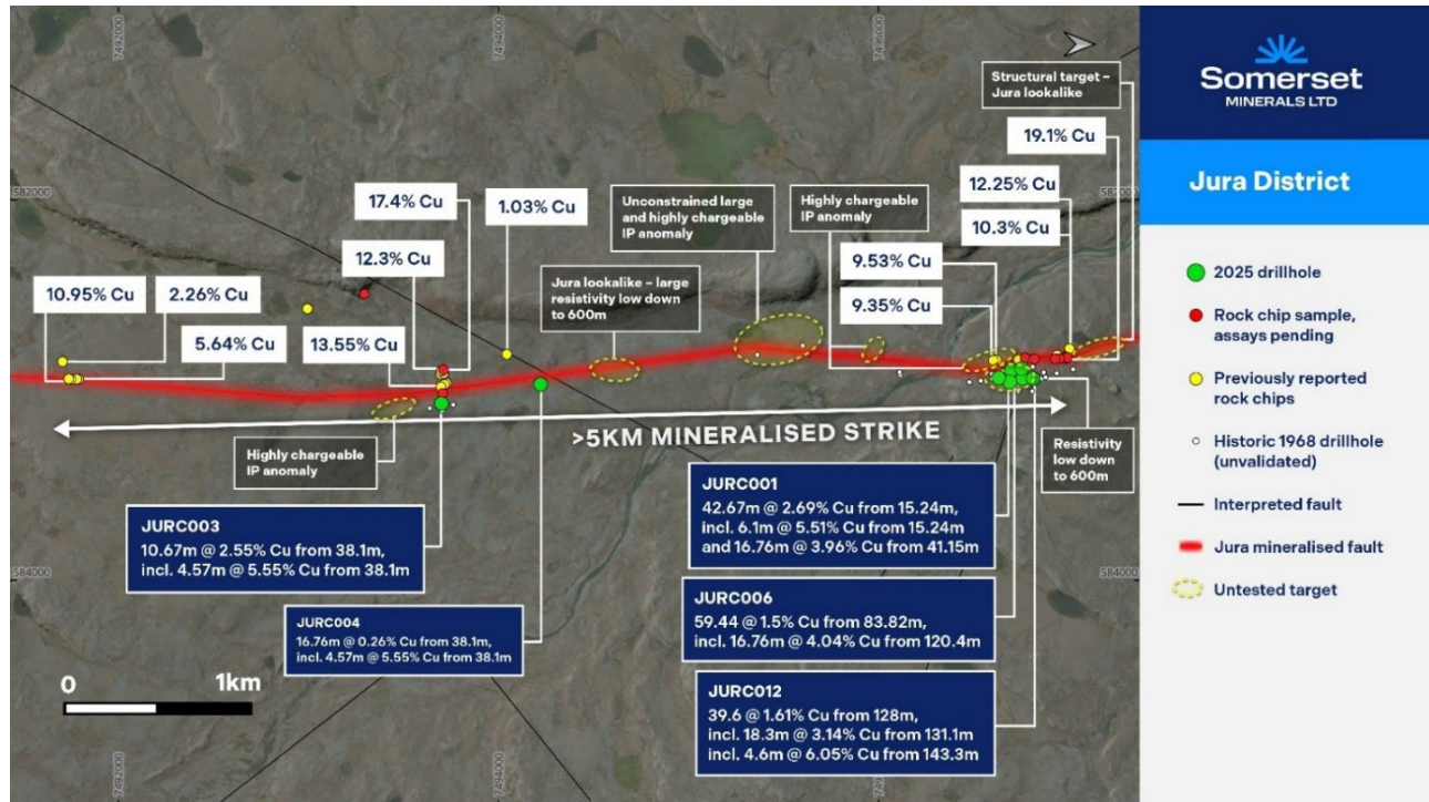
Figure 3: Plan map showing wider Jura prospect area, drill hole collar locations, significant intercepts and rock chip samples.
