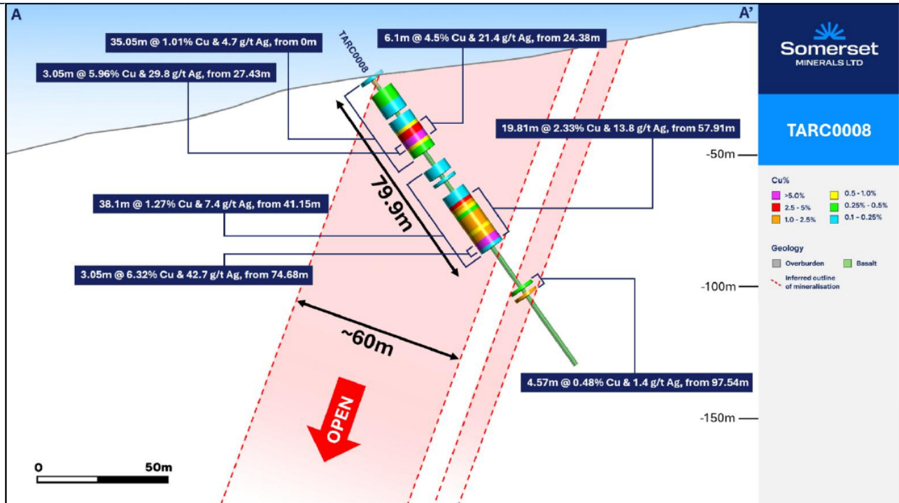
Figure 7: Cross section through TARC0008.
