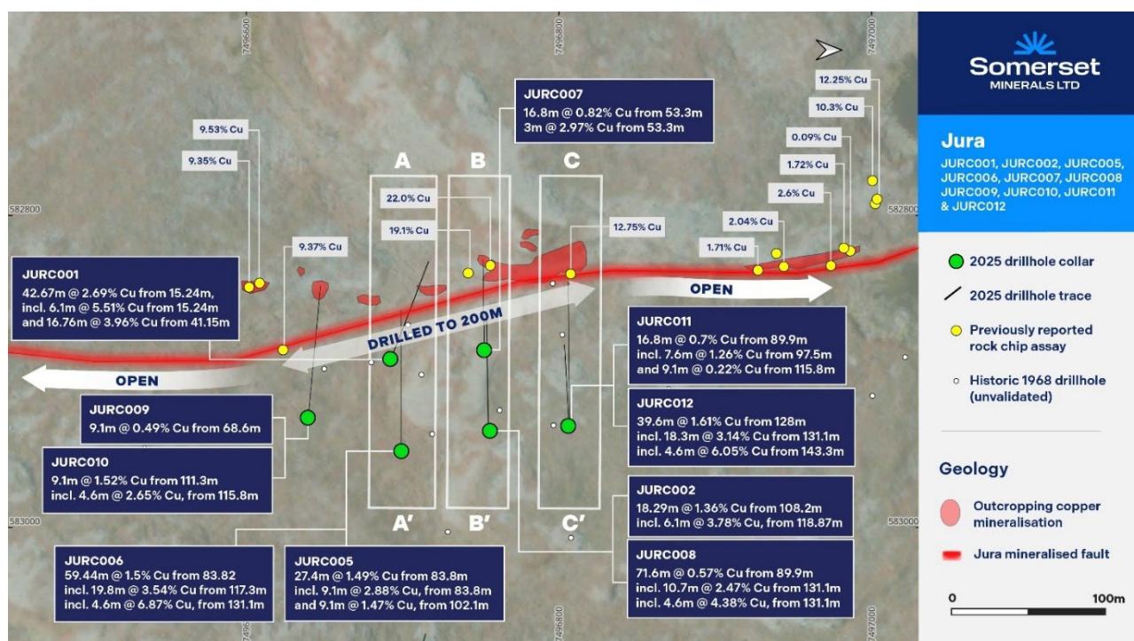
Figure 2: Plan map showing drill hole collar locations and significant intercepts.
