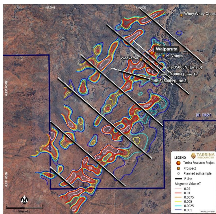
Figure 3. Location of the IP lines in relation to the magnetic anomaly highlighted by previous targeting in relation to historic drilling and historic mines at Walparuta 1 .
