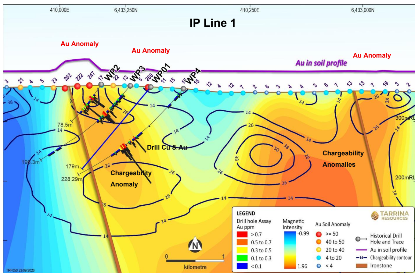
Figure 2. Profile sectional plot of the gold soil geochemistry over the bedrock copper and gold in historic drilling relative to the magnetic intensity and chargeability anomalies and down dip projection of mapped ironstone alteration.
