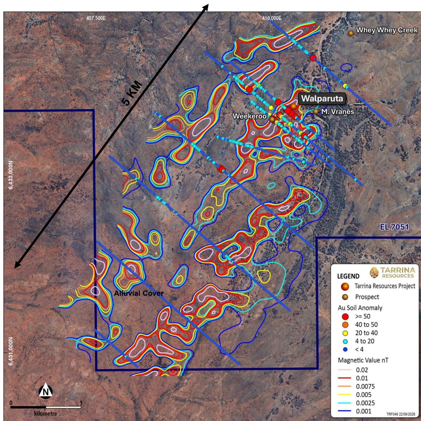
Figure 5. Gold soil anomalies on the IP lines plotted relative to the anomalous magnetic-gravity-chargeability corridors, ironstones, drill locations and historic mines.
