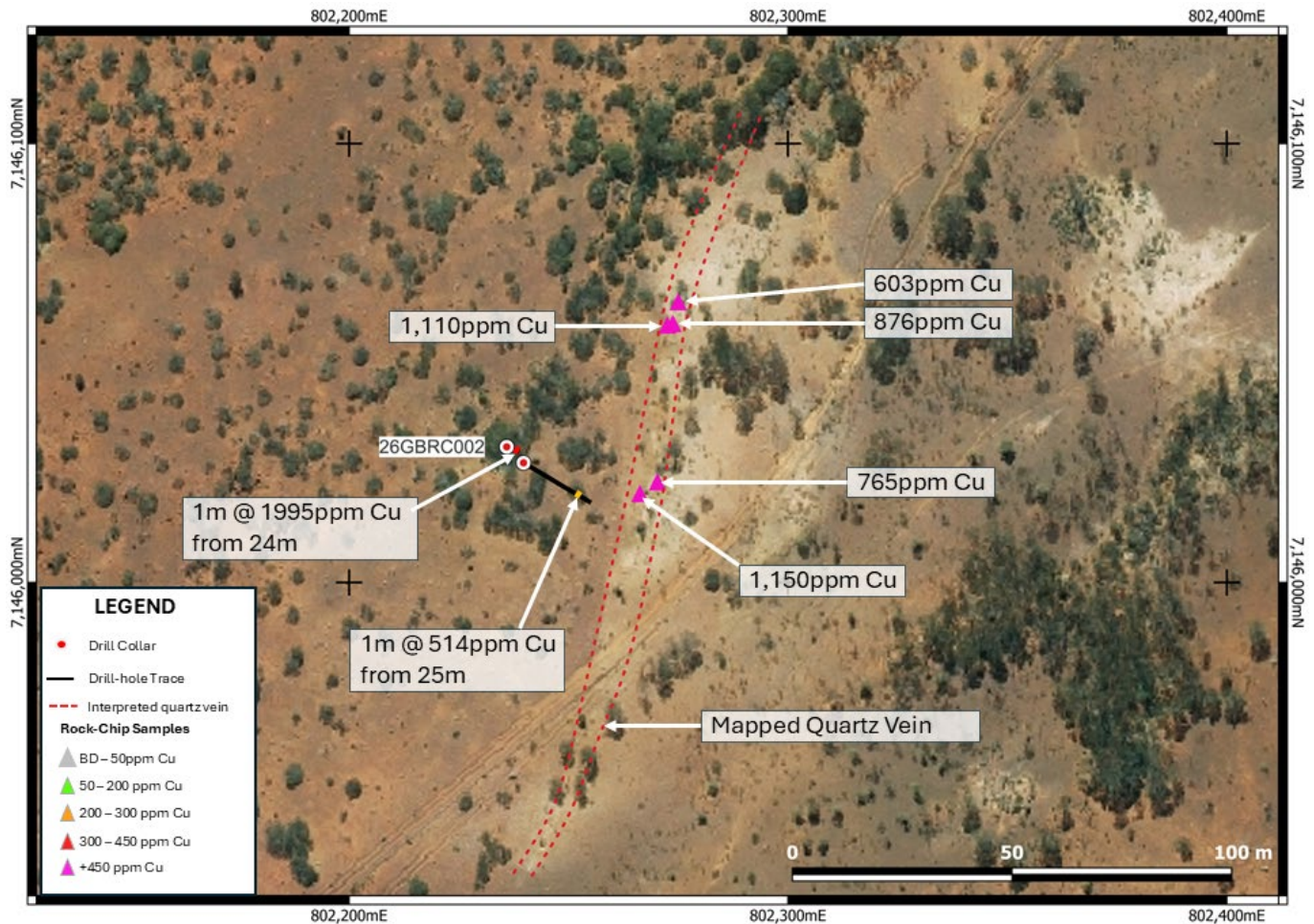
Figure 6: The Baroo mapped and interpreted quartz vein, overlaid with anomalous copper rock-chip samples (GTE ASX Announcement 2 February 2026), and maiden RC drill holes. Highest copper result recorded from this target was from drill-hole 26GBRC002 with 1m @ 0.2% Cu from 24m.
