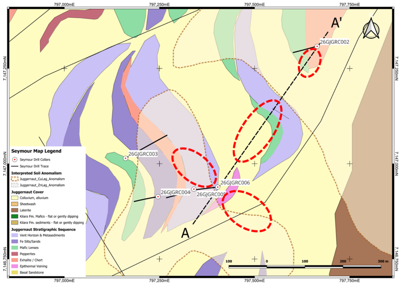
Figure 5: Seymour follow-up drill targets in red to test mineralised stratigraphy identified in the maiden RC drilling programme.
