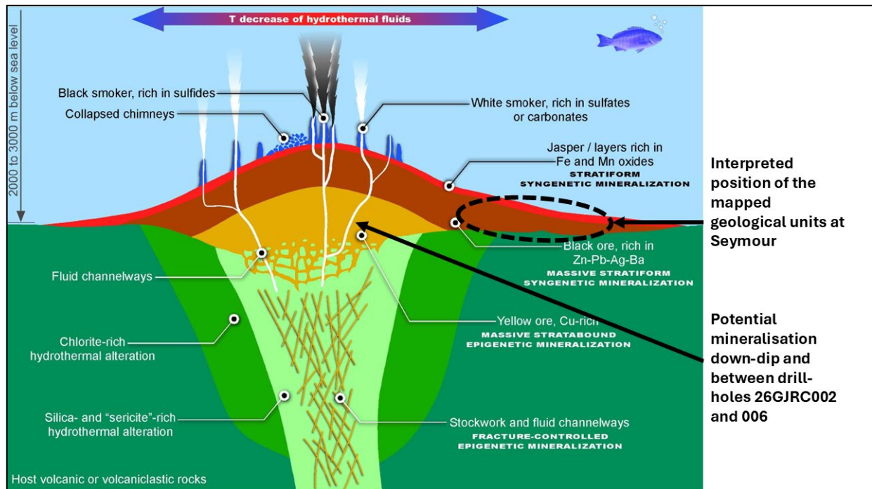
Figure 3: Schematic diagram of a volcanic hosted massive sulphide system (VHMS), and the interpreted mapped position of the drilled intercepts at Seymour (after Colin-Garcia et al, 2016).
