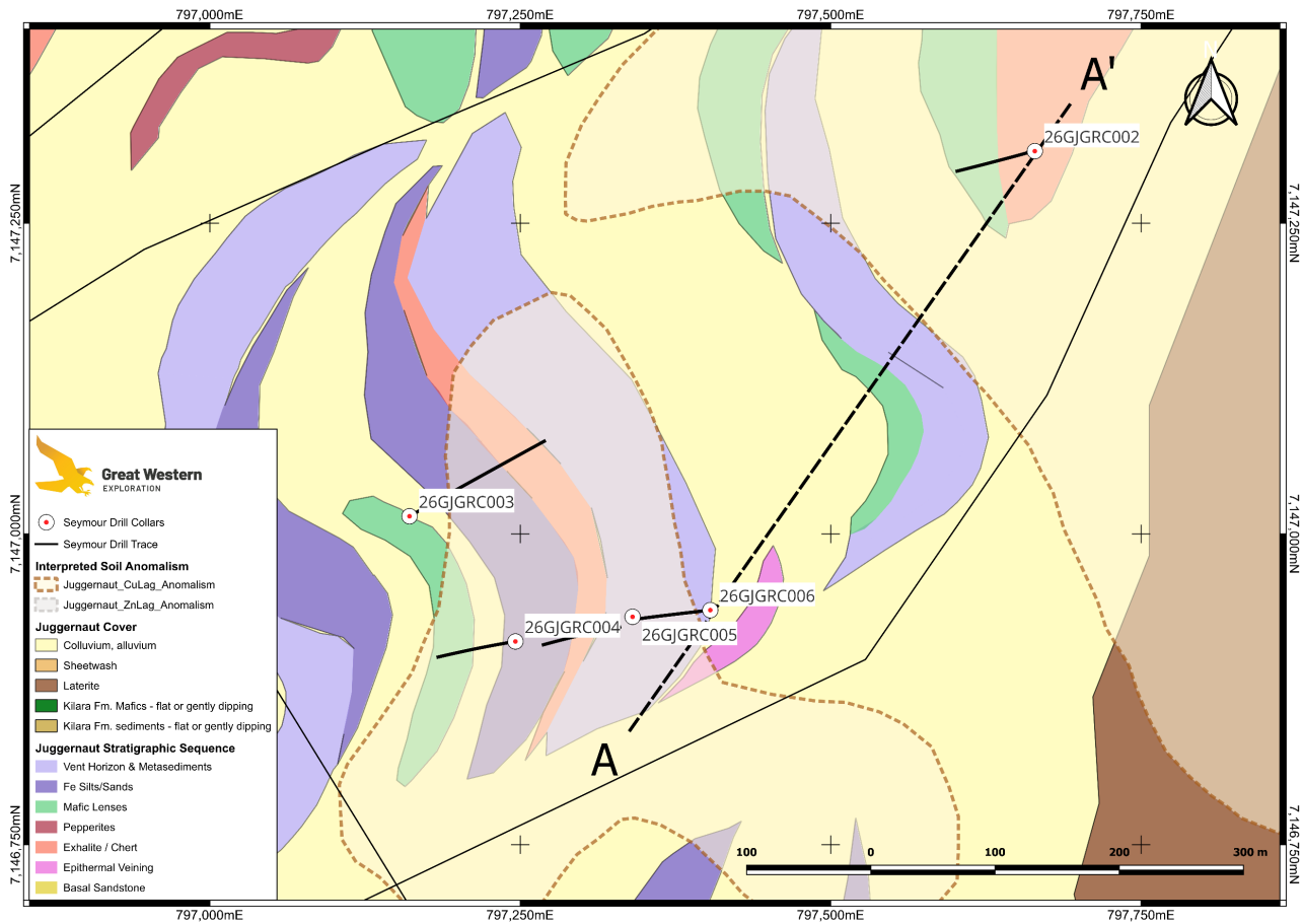
Figure 2: Plan section of completed RC drill-holes at the Seymour Target. Note section line referenced in Figure 4.
