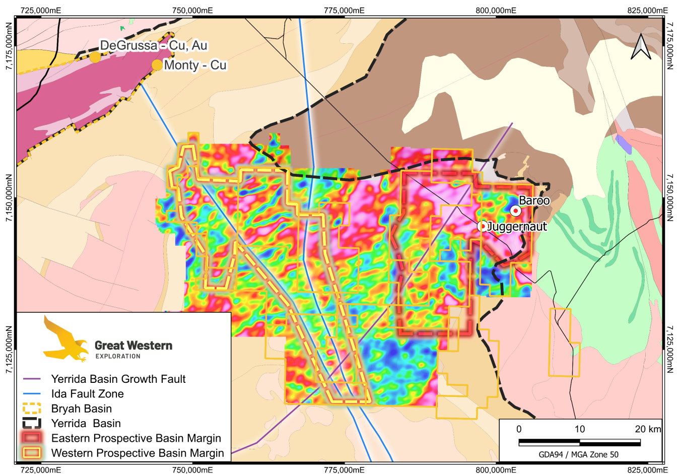
Figure 1: Location of the Juggernaut VHMS Target in relation to Great Western Tenements within the Yerrida Basin and the nearby DeGrussa and Monty copper-gold VHMS deposits.
