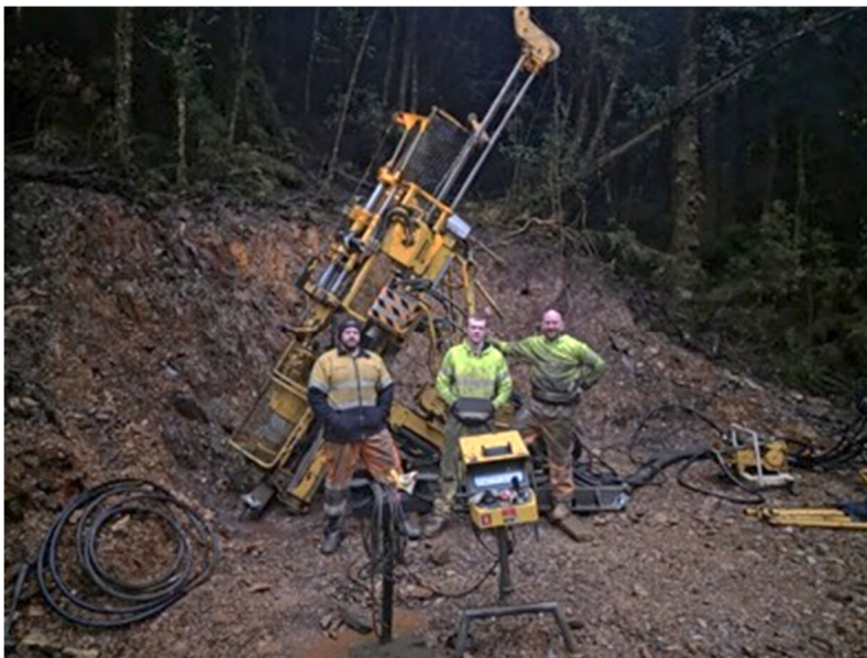
Figure 4 Drilling rig set up on hole MZS43 at Montezuma
