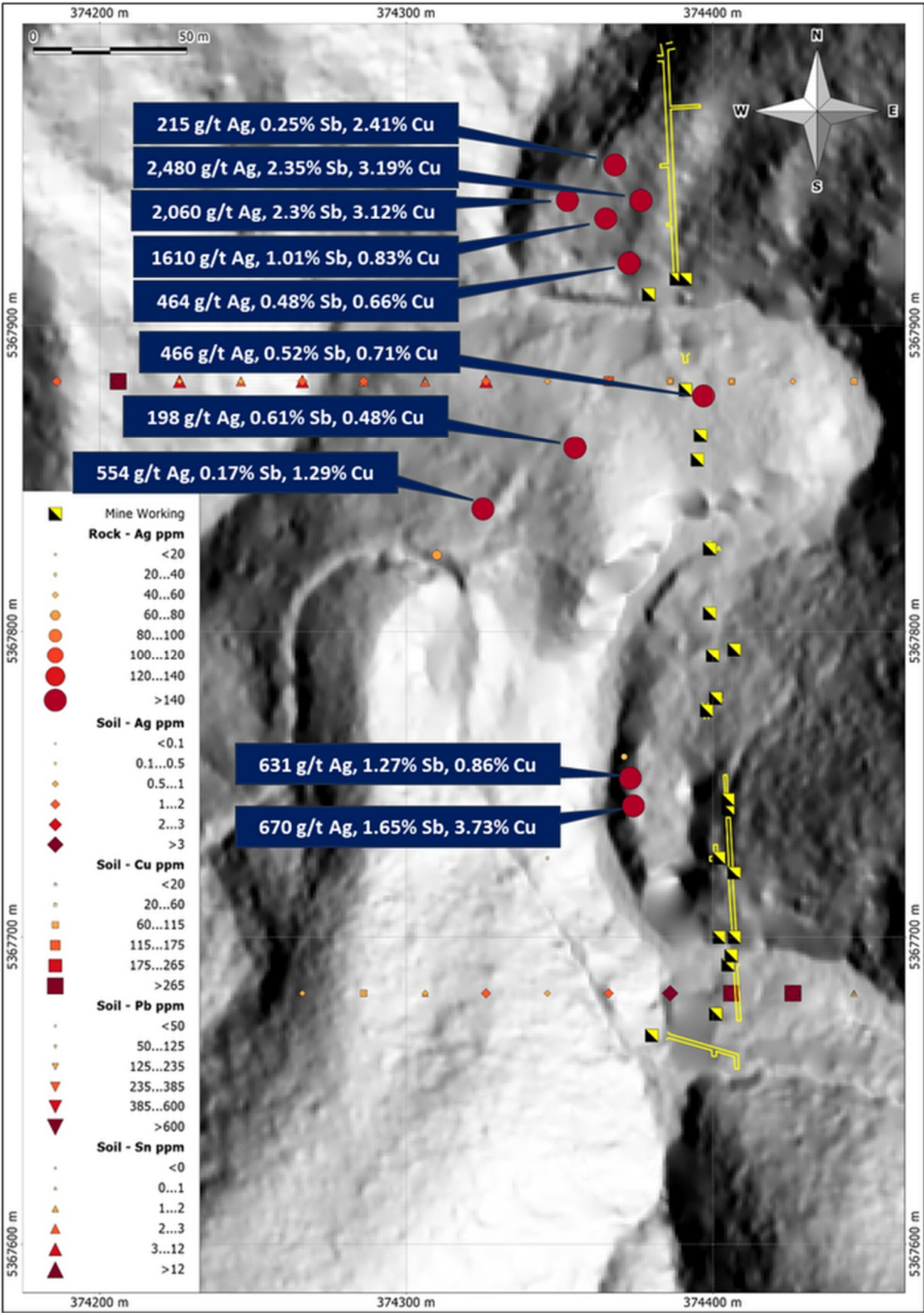
Figure 10 Montezuma Silver & Antimony Project – Fahlore mine work
