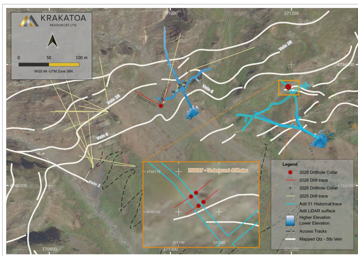
Figure 5: Plan view showing the 2026 Phase 2 resource definition drilling programme and mapped mineralised quartz-antimony veins at Zopkhito
