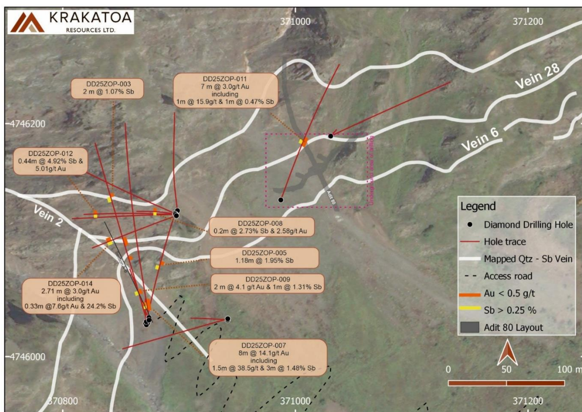
Figure 2: Plan view showing Phase 1 surface diamond drill hole locations, drill traces, mapped quartz-antimony veins and significant gold and antimony intersections at Zopkhito
