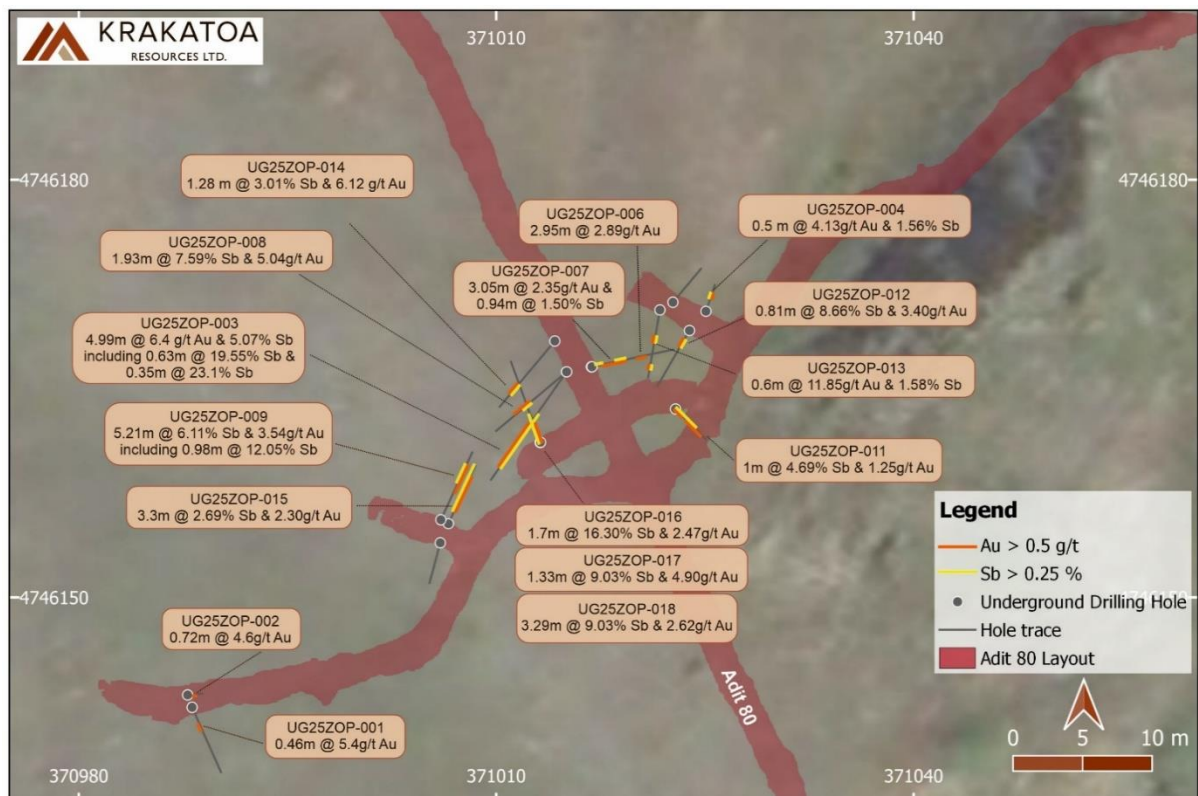
Figure 3: Underground drilling at Adit #80 showing drill hole locations and significant gold-antimony intersections
