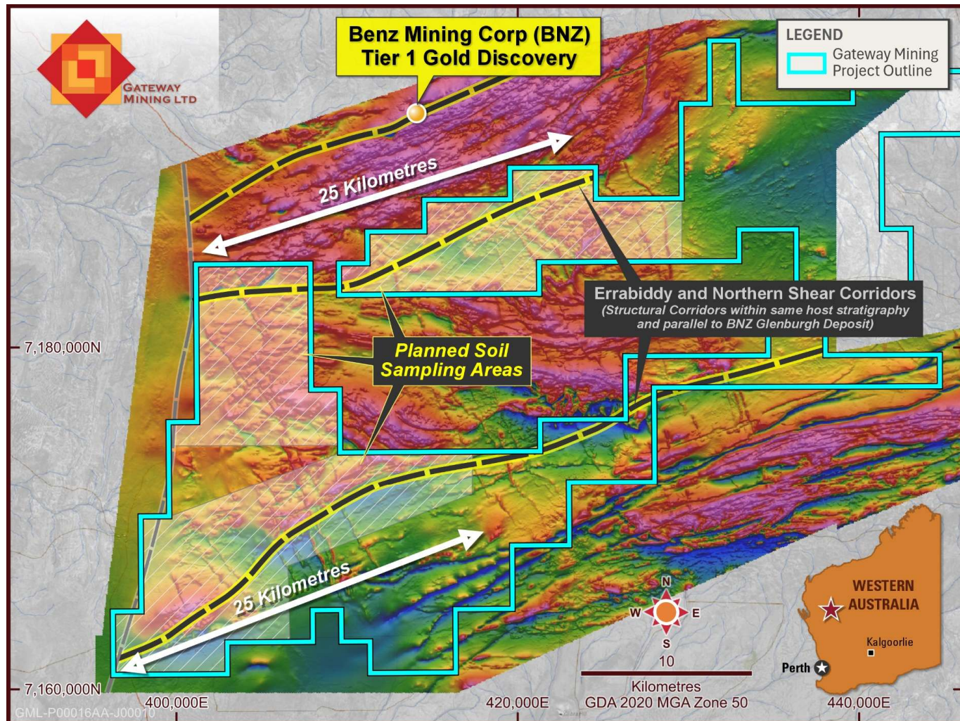
Figure 9: Planned soil sample areas in relation to key regional structures. Coloured airborne magnetic underlay.
