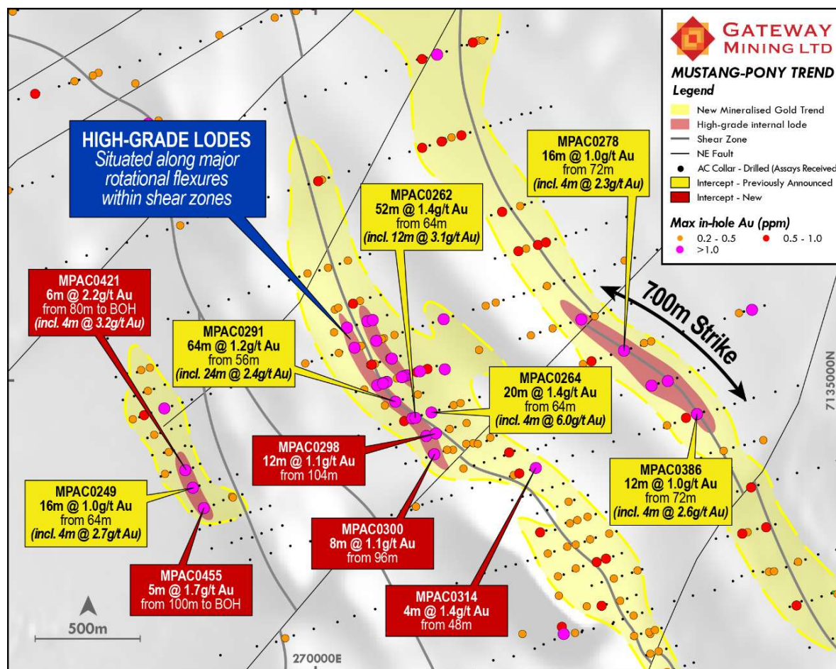
Figure 5: Zoomed in map of the Hummer, Haflinger and Rubicon prospects, highlighting new and previously announced key results.
