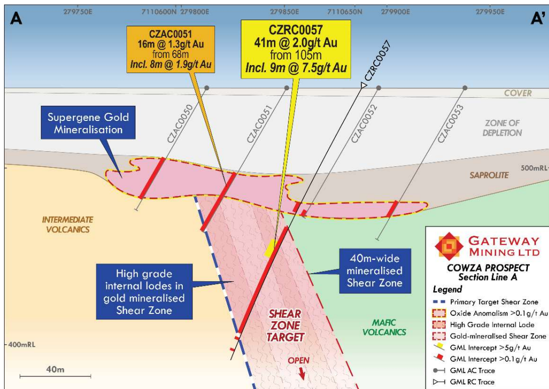
Figure 3: Cross section A-A' highlighting the new high-grade primary gold discovery at Cowza from RC hole CZRC0057.
