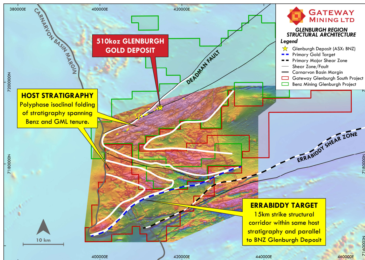
Figure 8: Plan view map of the Glenburgh South Magnetic survey overlain on regional GSWA Magnetic Imagery. Folded stratigraphy highlighted (white lines), along with major shear structures.
