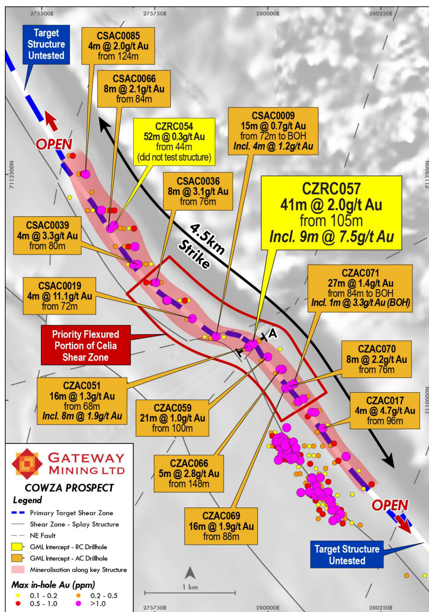
Figure 2: Plan view highlighting the new high-grade primary gold discovery at Cowza from RC hole CZRC057.
