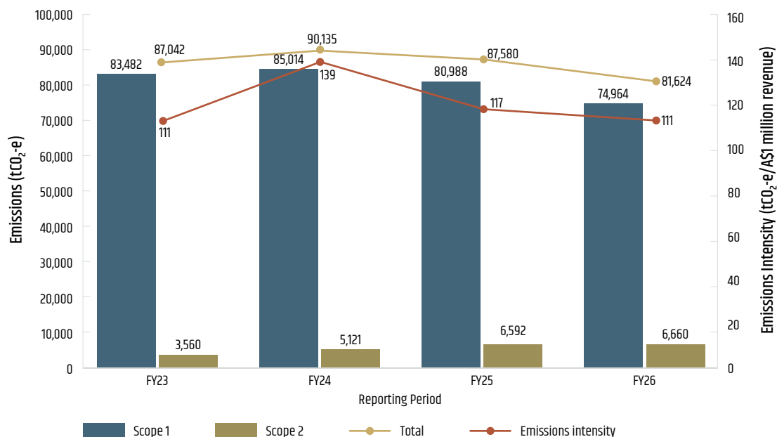
Figure 6: Tshipi's total Scope 1 and 2 emissions and operational GHG emissions intensity from FY23 to FY26
