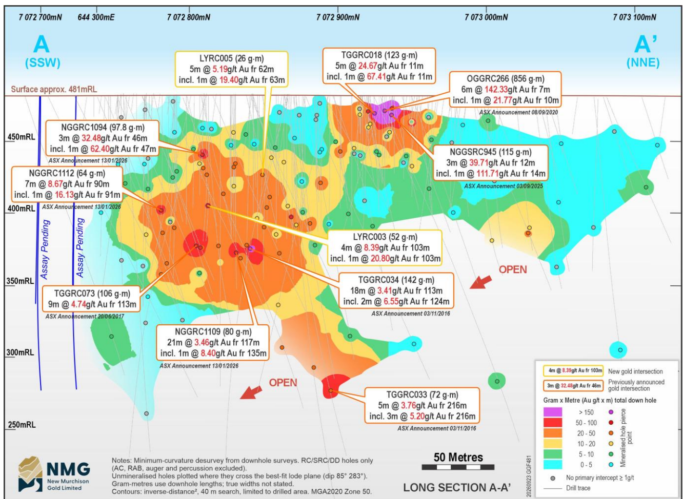
Figure 7: Lydia Main gram-metre (Au g/t x m) long section looking 284°, showing primary intercepts ≥1g/t Au. Includes previously reported and historic drill results.
