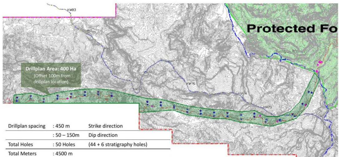
First stage TBAR Drill plan
