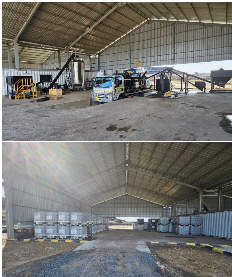
Drill & Blast Mixing Plant Facilities
