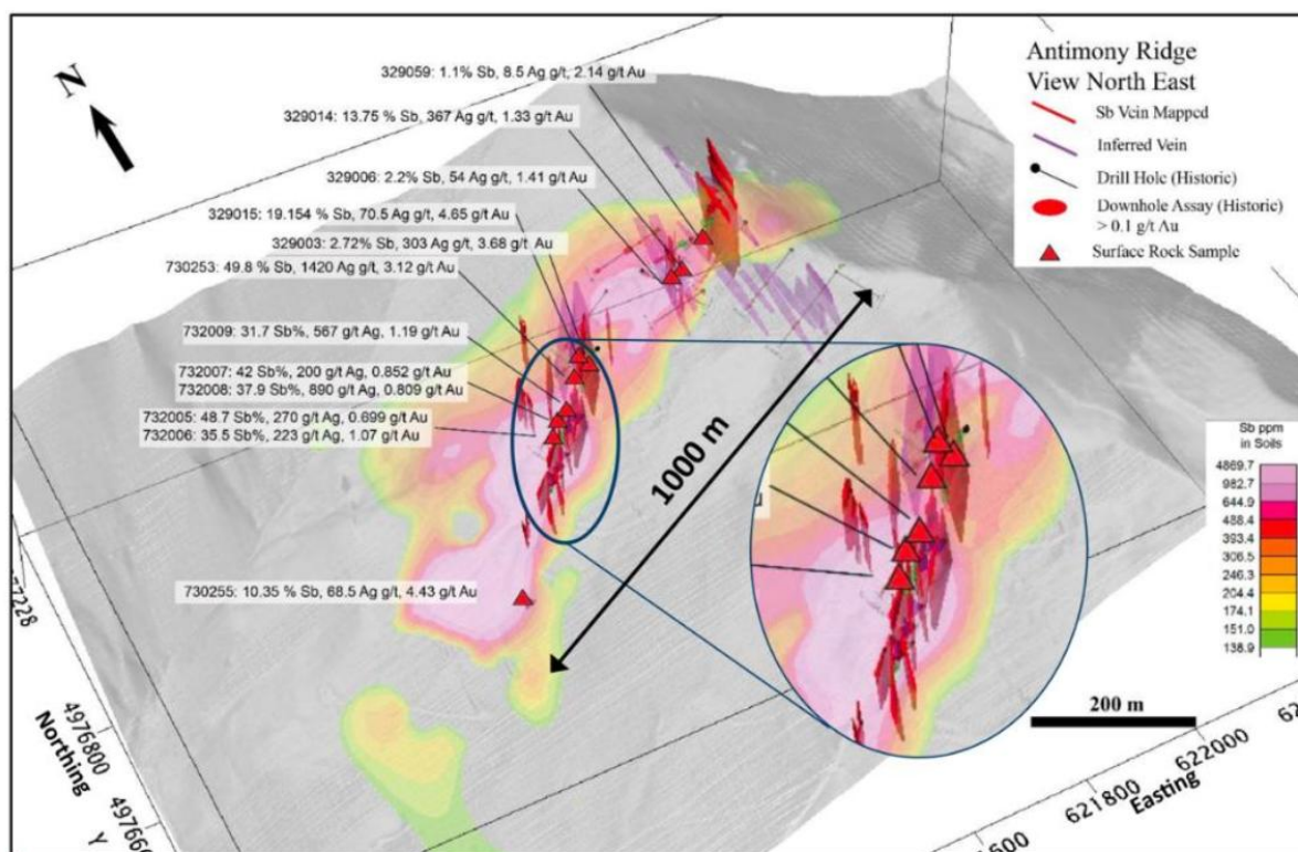
Figure 3: Antimony Ridge – High grade antimony veins and mineralisation with assays, modelled as 30 discrete mineralised vein swarms, fault breccias and stockworks, within past open pits and trenches. Veins and vein swarms are surrounded by a lower grade antimony halo of veinlets and stockwork shown in a coloured antimony-in-soil geochemical anomaly map with averaged assays. Veins, assays and soil geochemistry are draped over a 3-D shaded image. Results extend over a large area 1000m x 700m and 250m vertically.
