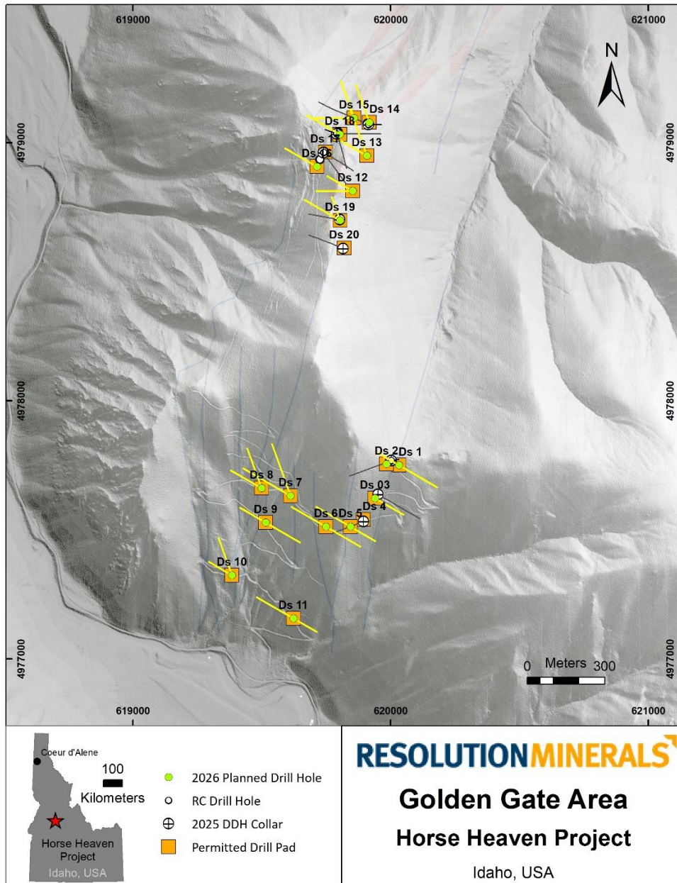
Figure 2. Horse Heaven Project location map showing the Golden Gate prospect and identifying locations of completed Phase 1 drill hole locations (2025 DDH Collar) and ongoing Phase 2 drill hole locations (2026 Planned Drill Hole)
