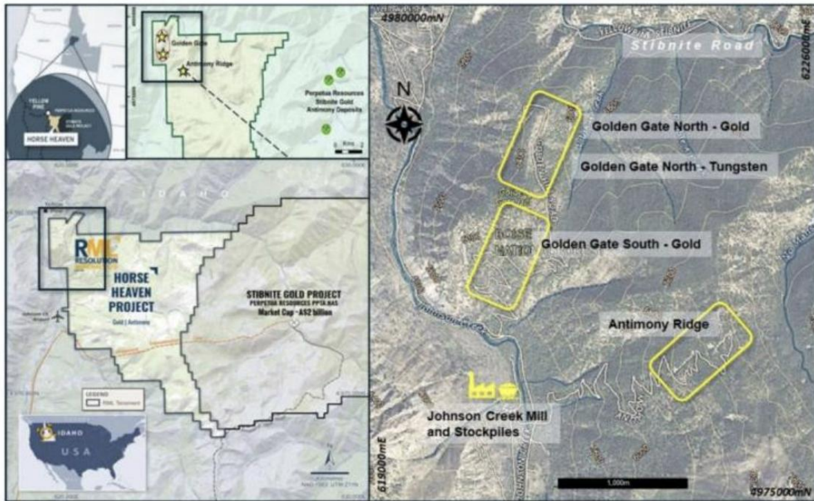
Figure 1. Horse Heaven Project location map showing the location of the Antimony Ridge antimony-silver prospect, Golden Gate gold-tungsten prospects, Johnson Creek processing infrastructure and neighbouring Stibnite Gold Project in Idaho, USA.
