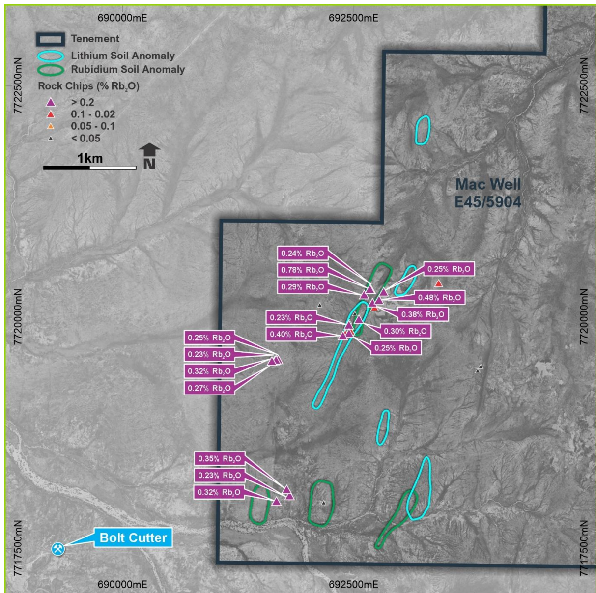
Figure 3: Mac Well Rock Chip Samples showing \text{Rb}_2\text{O} (%) grade
