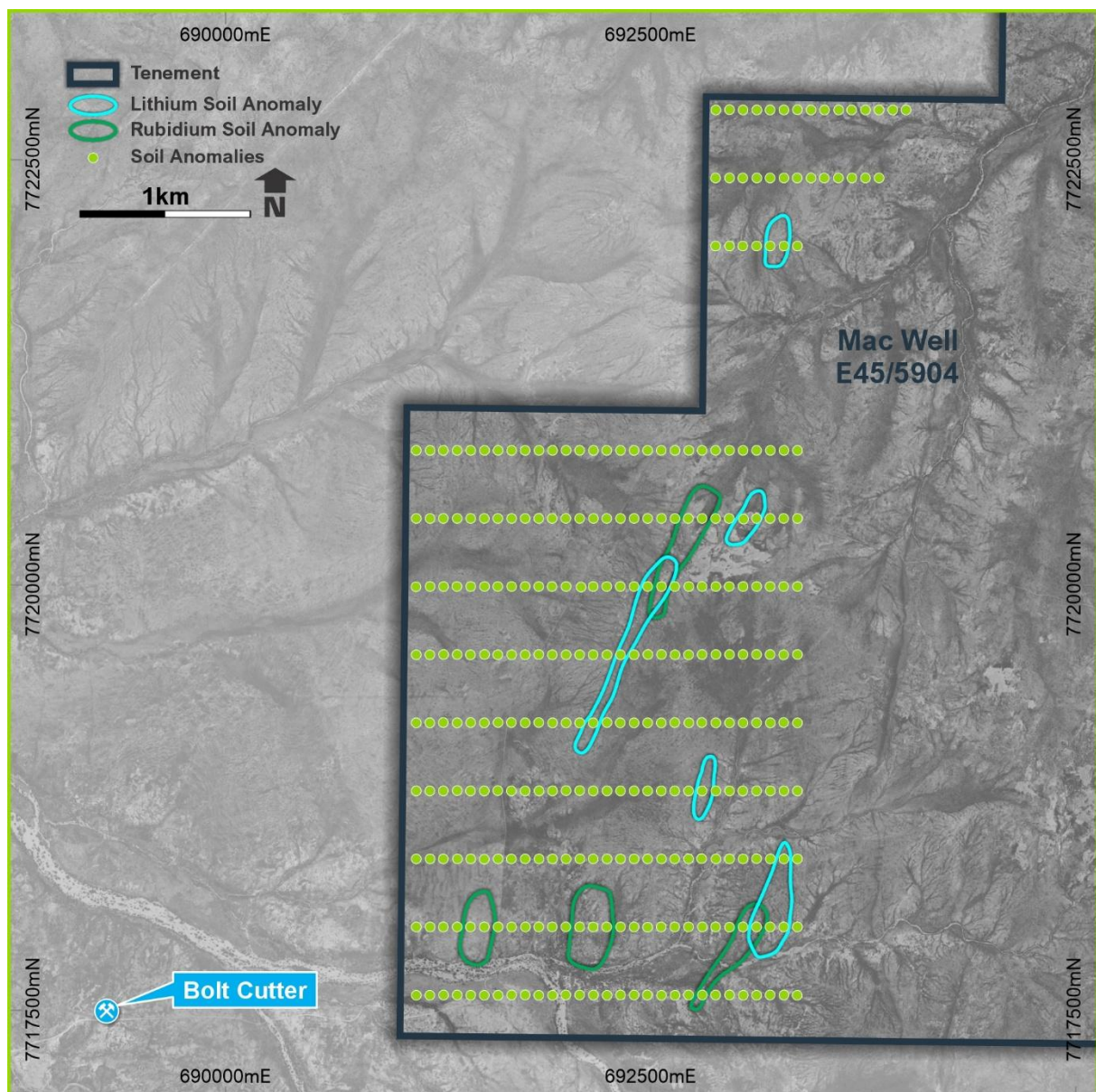
Figure 2: Mac Well soil sampling program
