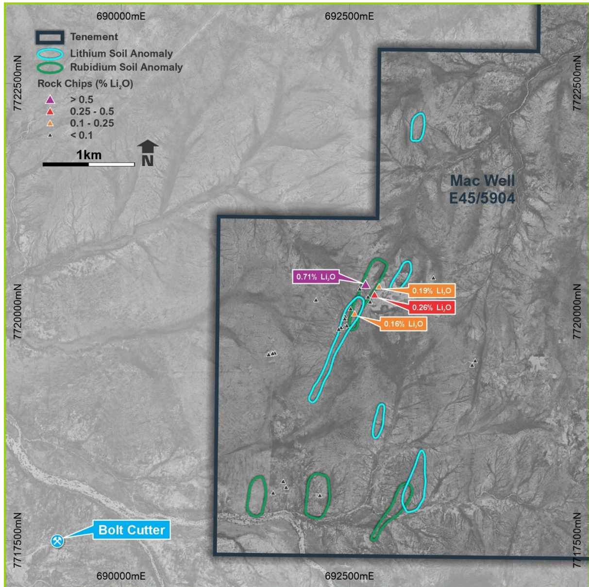
Figure 4: Mac Well Rock Chip Samples showing \text{Li}_2\text{O} (%) grade
