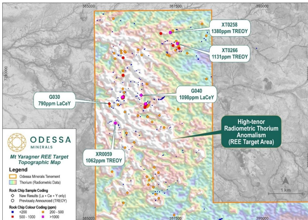
Figure 7: Rock chip samples at Mt Yaragner colour coded by TREOY ppm (pre-2026 samples), and La + Ce + Y ppm (new samples) underlain by radiometric thorium gridded data. 5
