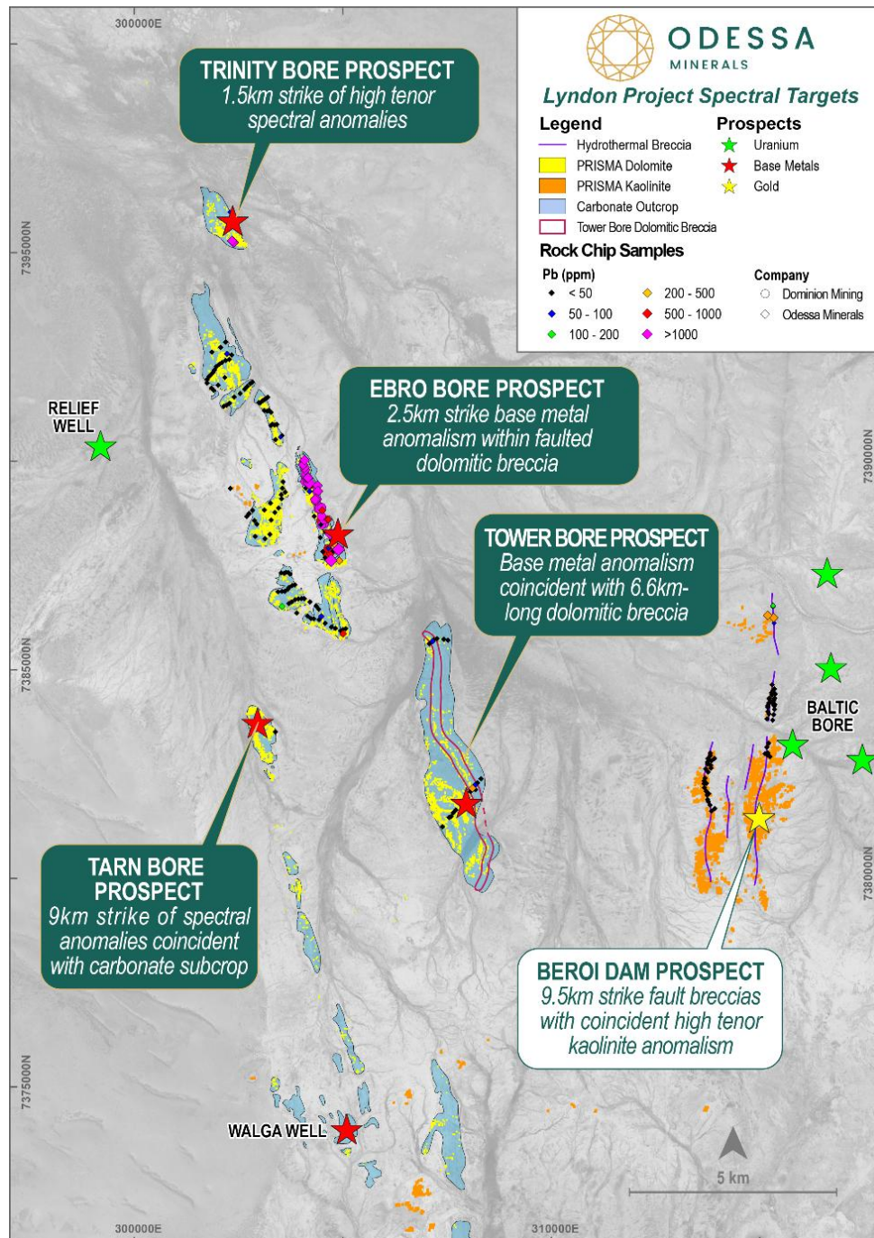
Figure 5: 95th percentile dolomite (yellow) and kaolinite (orange) anomalies at Lyndon in relation to mapped Gneuda Formation and hydrothermal fault breccias. Rock chip samples coded by Pb ppm displayed. 4
