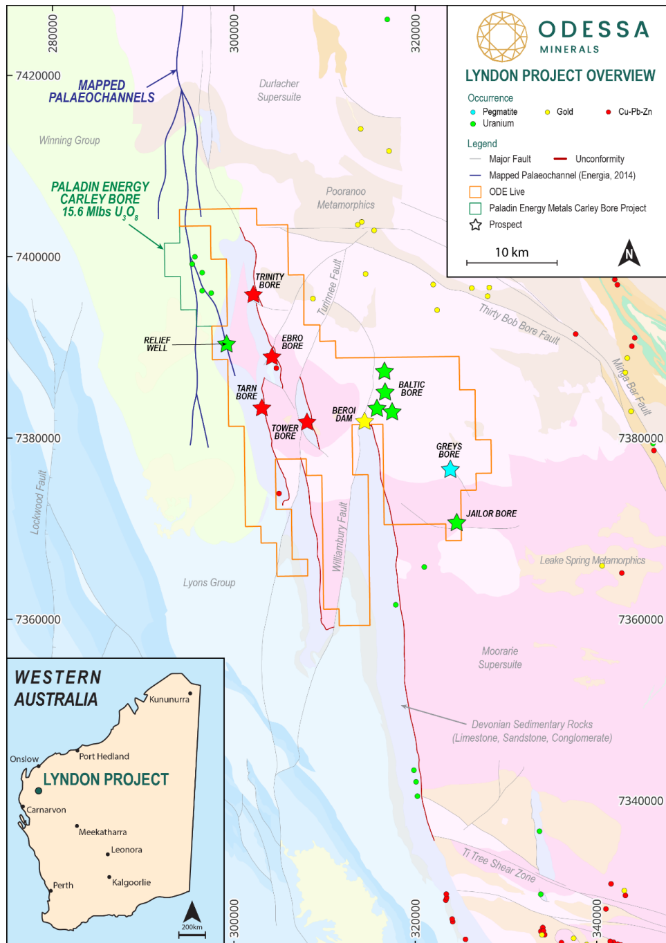
Figure 2: Lyndon Project in relation to Minedex occurrences and the Carley Bore Project (Paladin Energy). Underlain with GSWA 1:500k bedrock geology and structures. 2
