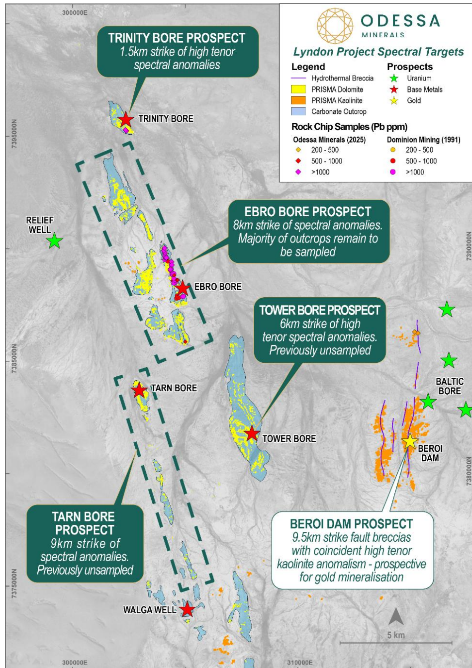
Figure 4: 95th percentile dolomite (yellow) and kaolinite (orange) anomalies at Lyndon in relation to mapped Gneuda Formation and hydrothermal fault breccias. 2
