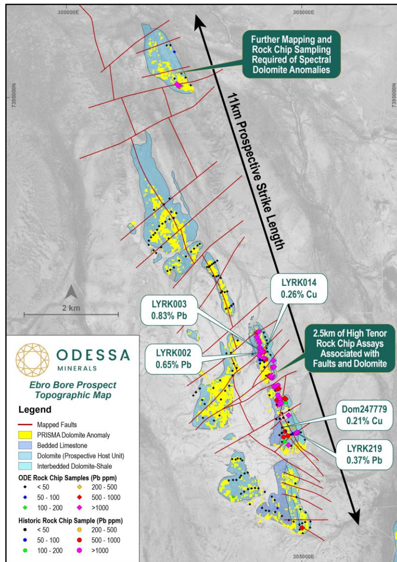
Figure 6: Ebro Bore Prospect rock chip samples coded by Pb ppm. 95th percentile PRISMA dolomite anomalies highlighted in yellow overlain on outcropping carbonates. Rock chip samples coded by Pb ppm displayed. 4
