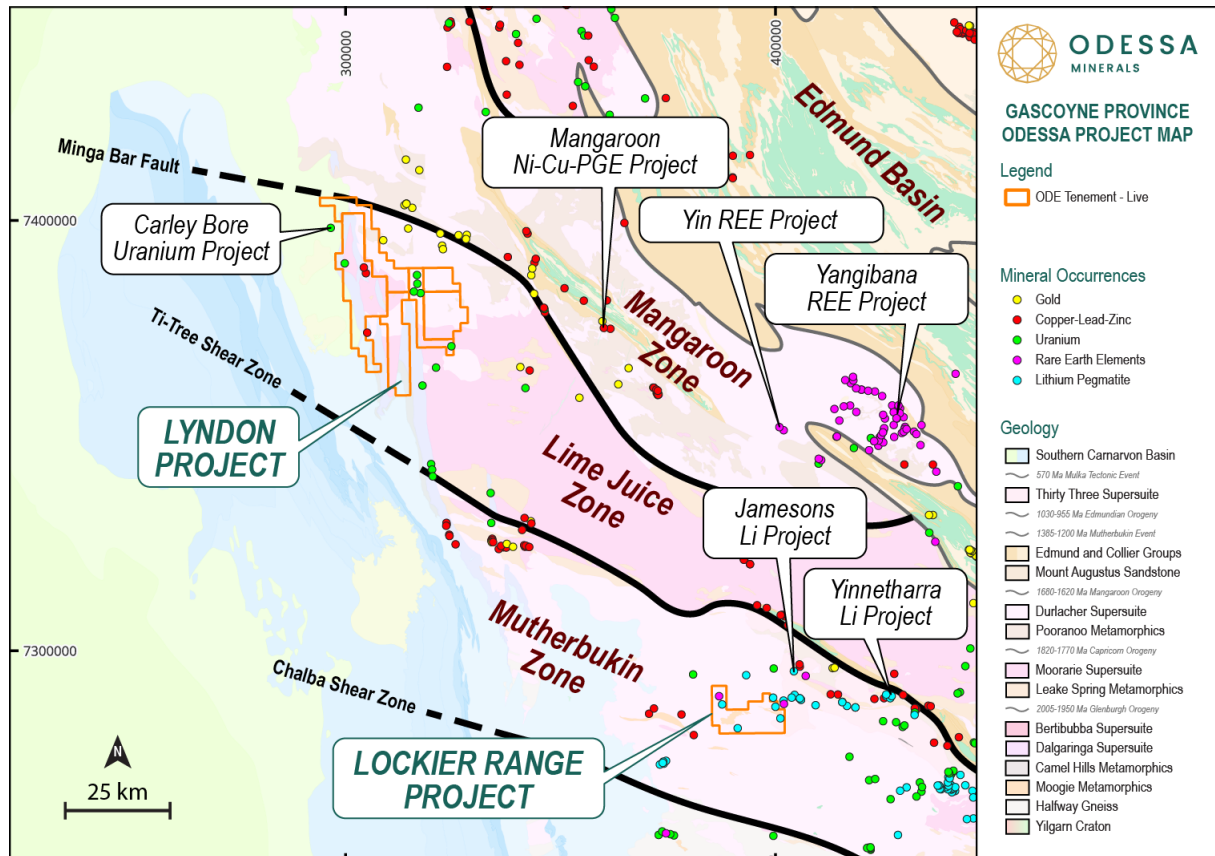
Figure 1: Odessa regional Gascoyne Project location map overlain with Geological Survey WA Minedex Occurrences. 1
