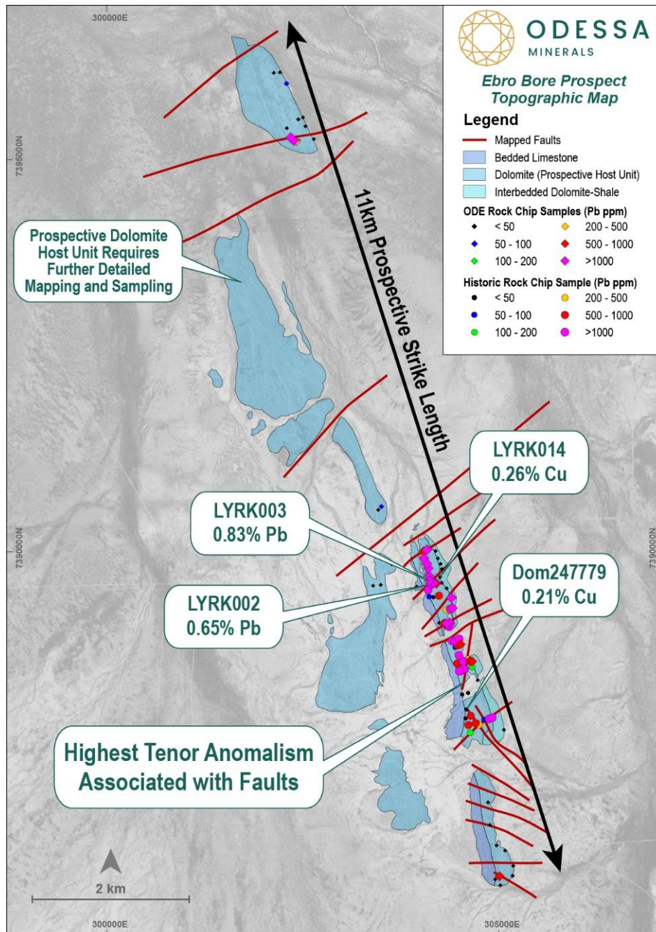
Figure 3: Ebro Bore Prospect first-pass rock chip samples coded by Pb ppm. Mapped Gneuda Formation units and faults displayed. 1
