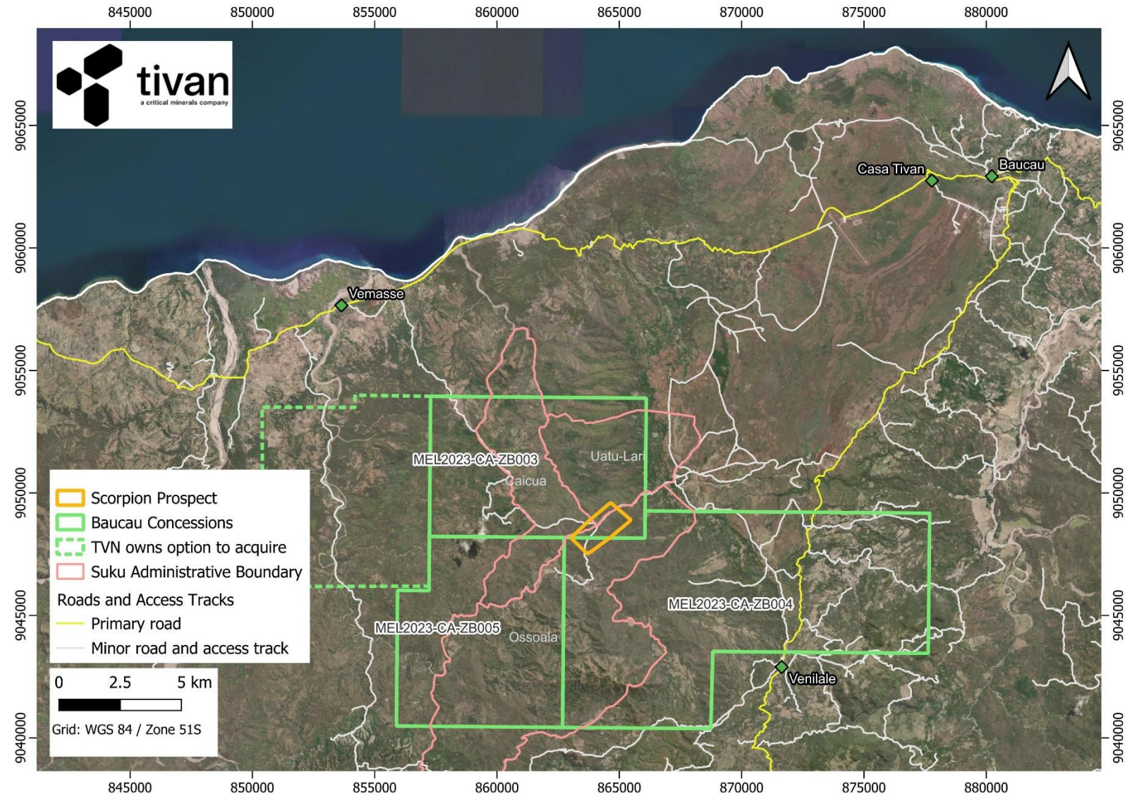
Figure 8: Baucau project concessions, with the proposed Scorpion Prospect activity extent polygon
