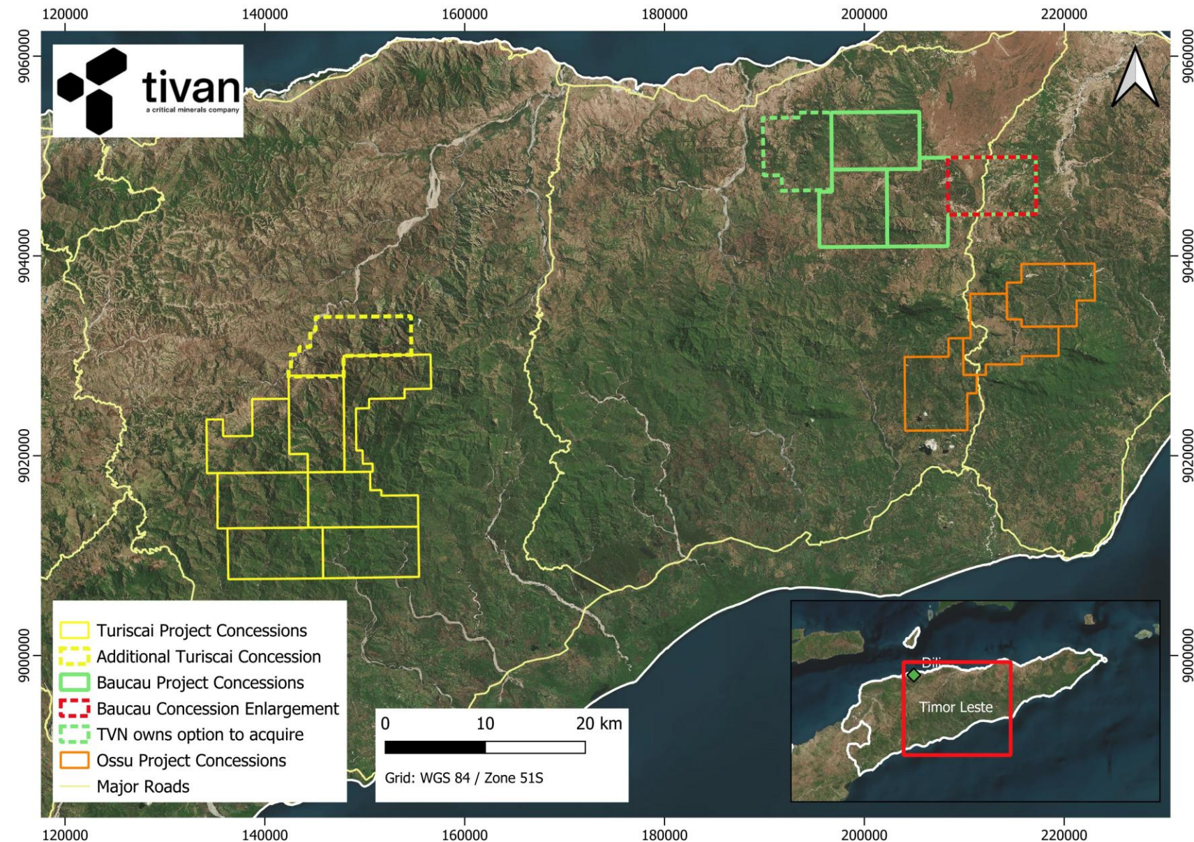
Figure 7: Location Map showing Tivan's Timor-Leste projects with recently granted expanded footprint shown in dashed lines (29 September 2026)
