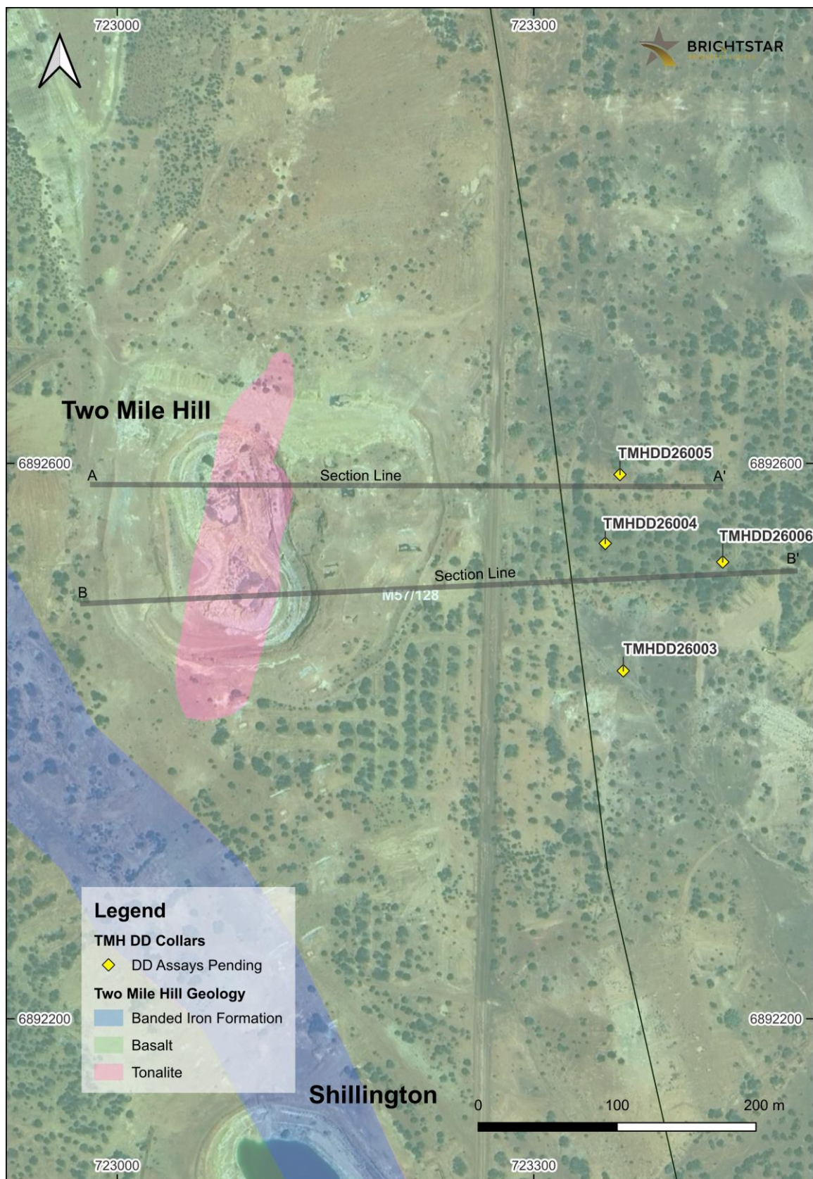
Figure 3: Location map of the Two Mile Hill diamond drillhole collars
