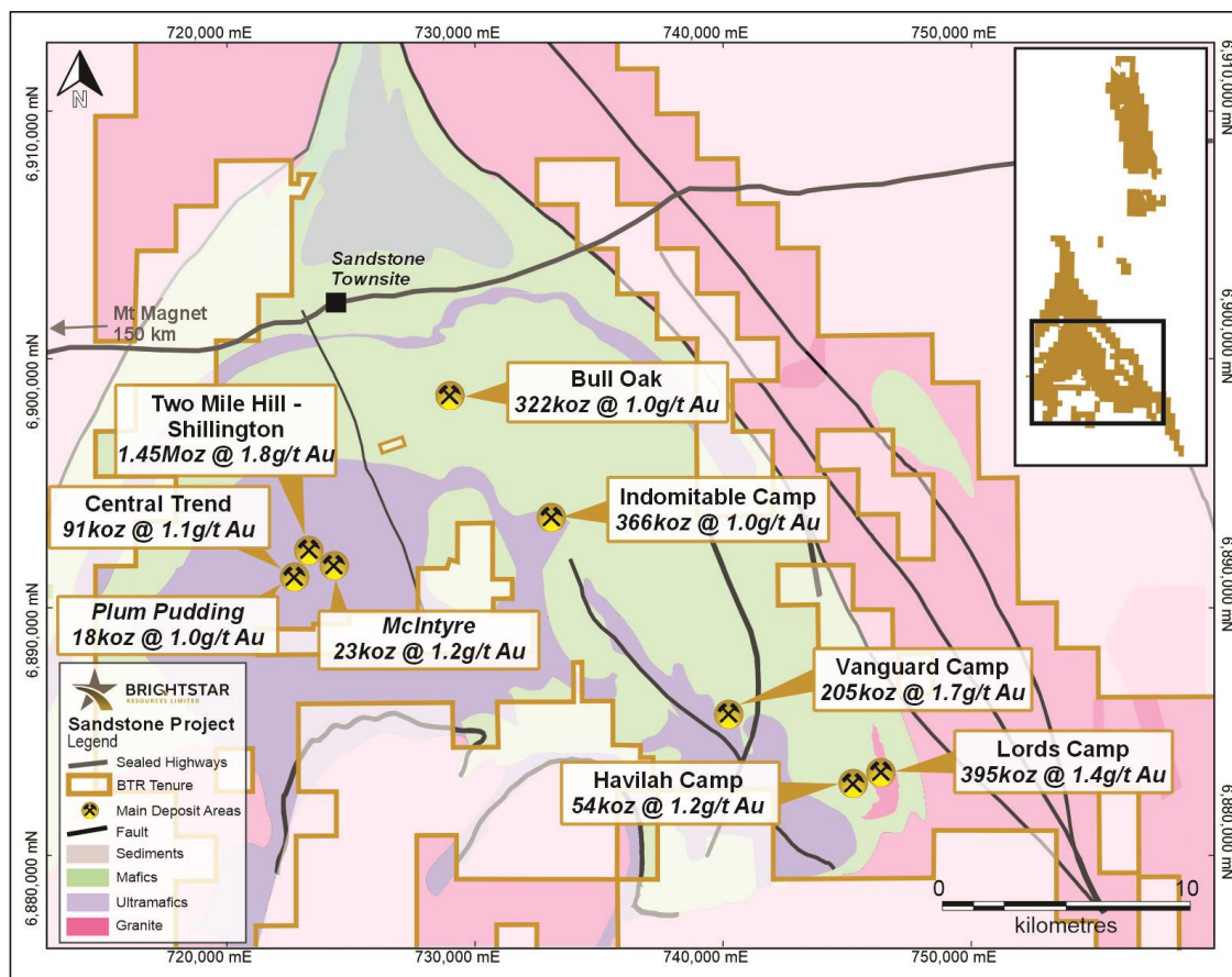
Figure 1: Central Sandstone Gold Project area
