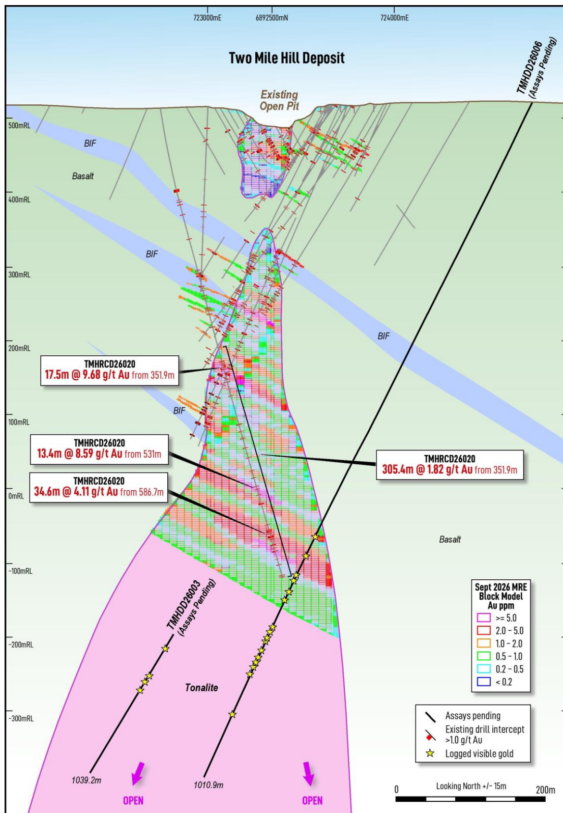
Figure 5: Cross section B-B' at the Two Mile Hill deposit, showing TMHDD26006 and TMHDD26003 (projected) in relation to the current MRE 1 .
