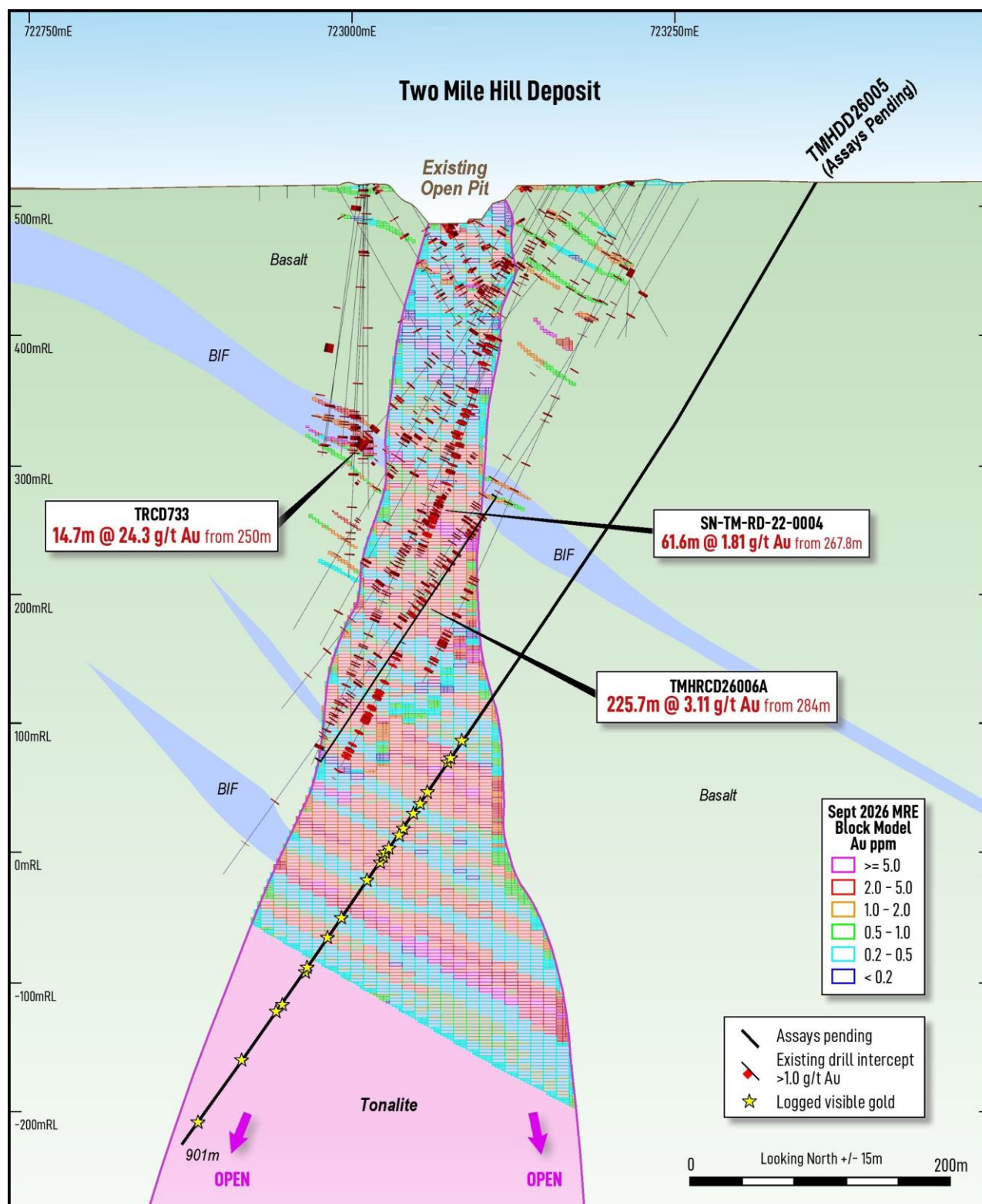
Figure 4: Cross section A-A' at the Two Mile Hill deposit, showing TMHDD26005 in relation to the current MRE 1 .
